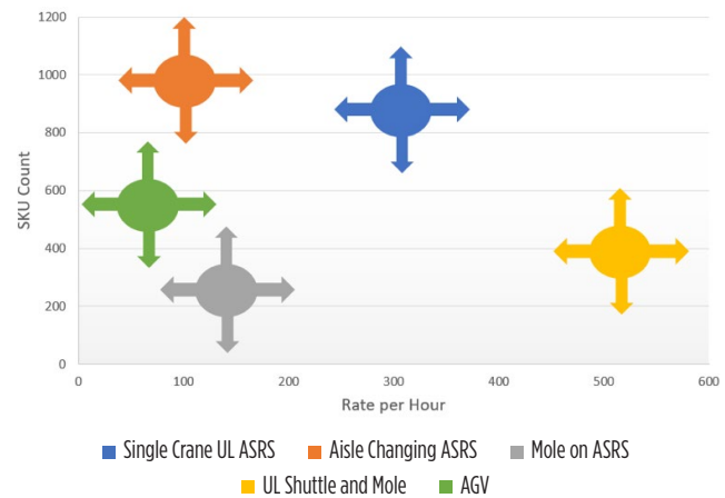
FIGURE 3: Unit load ASRS general selection based on SKU count and throughput. System throughput and SKU count are important considerations when selecting pallet-picking technology.
