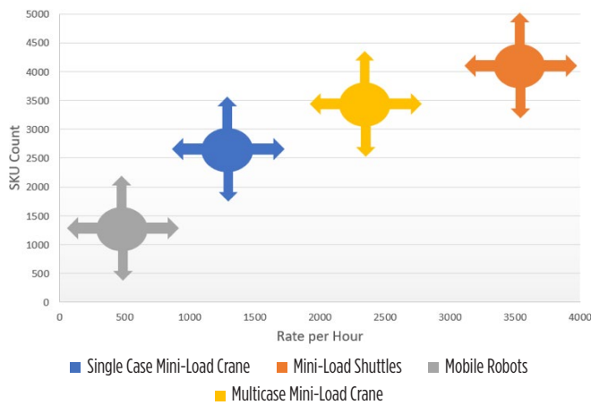
FIGURE 4: Case level ASRS general selection based on SKU count and throughput. System throughput and SKU count are critical when selecting case-picking technology.
