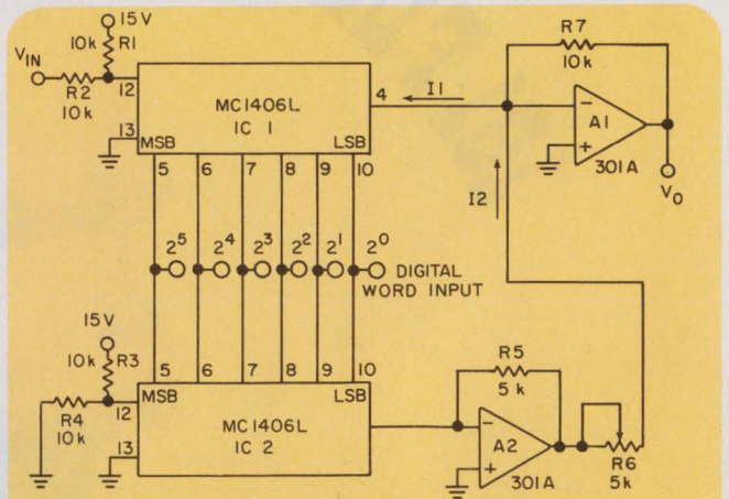
A combination of two unipolar multiplying d/a converters provides a bipolar-output scaled by the digital word input. Resistor R 6 should be set to equal the value of R 5 .
