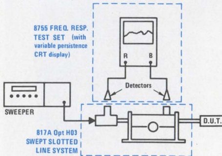
Simplified diagram of swept SWR test setup.
