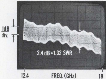
Trace envelope develops as probe is moved along slotted line while frequency is swept. The test device SWR equals the thickness of the envelope.
