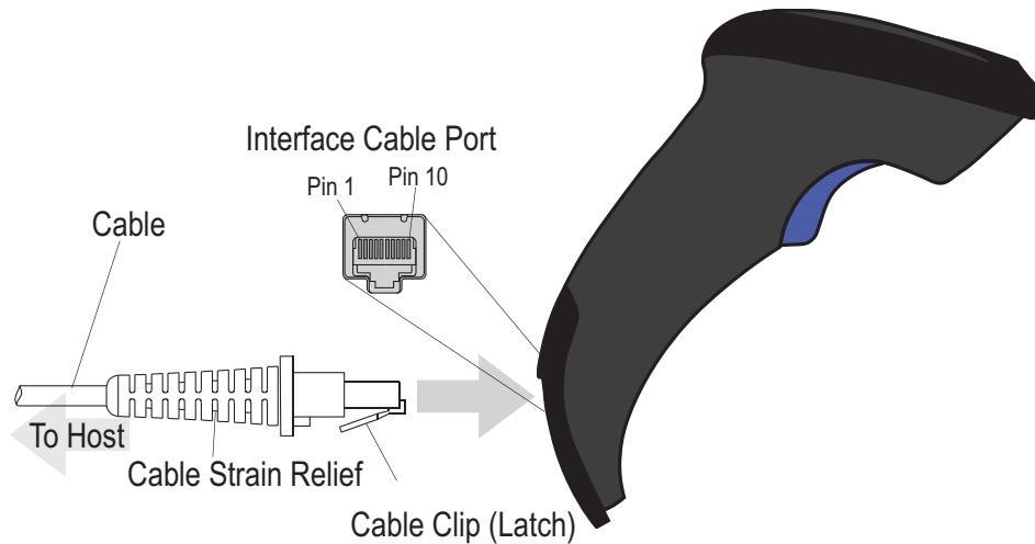
Figure 11. Standard Cable Pinouts
