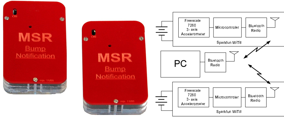
Fig. 4. (left) Photo of the encased prototype devices used in the experiments. (right) Block diagram showing two portable devices and an intermediate PC for processing.
