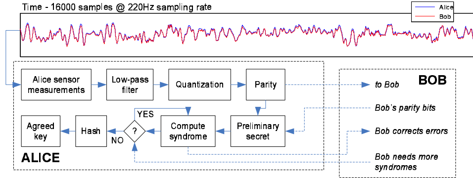
Fig. 2. Block diagram of the Martini Synch protocol. An example of sensor measurements taken from two devices during a 72.7 second Martini Synch at a sampling rate of 220Hz.
