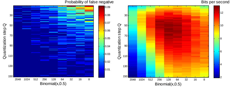
Fig. 6. (left) Color-coded plot of the probability of a false negative \varepsilon_{FN} . (right) Color-coded diagram of the entropy per second for correctly resolved shared secrets.
