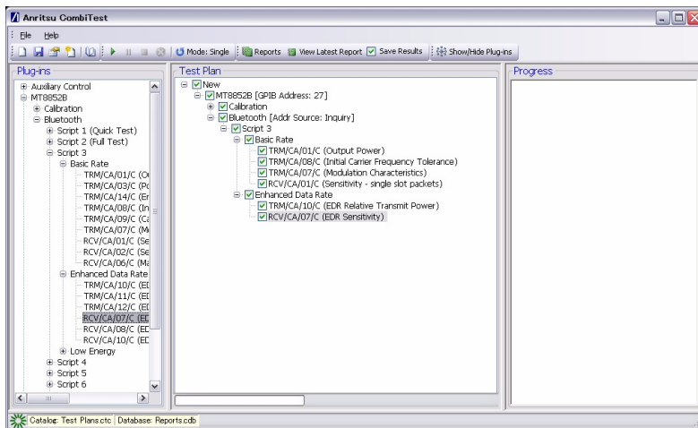
Figure 6-3. Test Plan with Two EDR Tests
