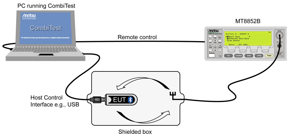
Figure 2-1. Equipment Configuration
