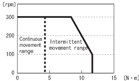
*This graph shows the characteristics under 3 phase AC200V
