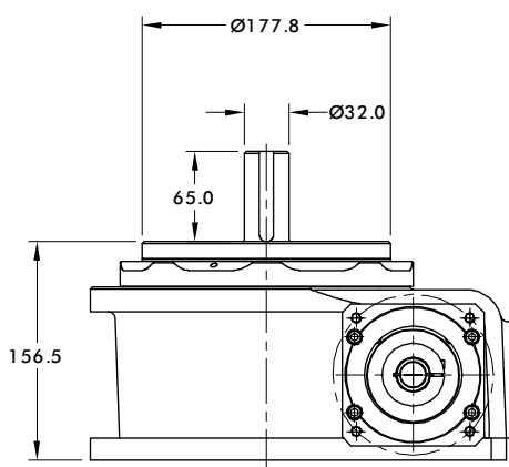
Shaft Output
