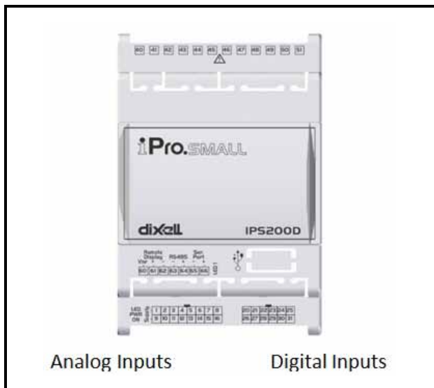
Figure 4-1 - Pump Skid Controller Input Locations
