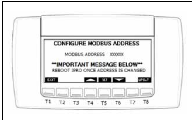
Figure 3-5 - Configure Modbus Address
