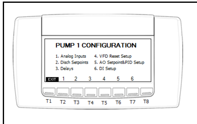
Figure 9-4 - Pump 1 Configuration
