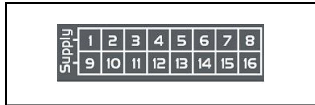
Figure 4-10 - Analog Output Connectors
