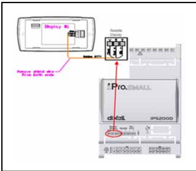
Figure 3-2 - Visograph connection
