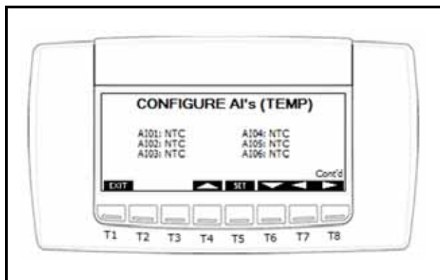
Figure 9-6 - Configure Analog Input's Temperature
