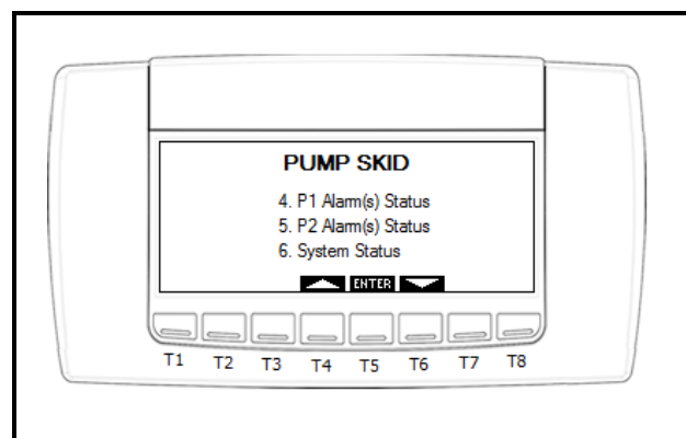
Figure 9-2 - Main Menu Page 2
