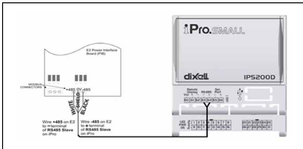
Figure 3-1 - MODBUS Networking
