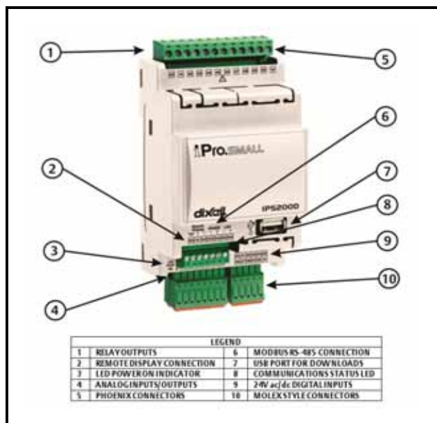
Figure 5-1 - Pump Skid Controller Status LED Locations
