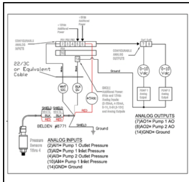
Figure 4-11 - Analog Output Wiring
