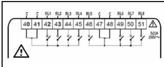
Figure 4-9 - Relay Output Wiring
