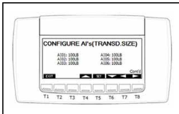
Figure 9-7 - Configure Analog Input's Transducer Size
