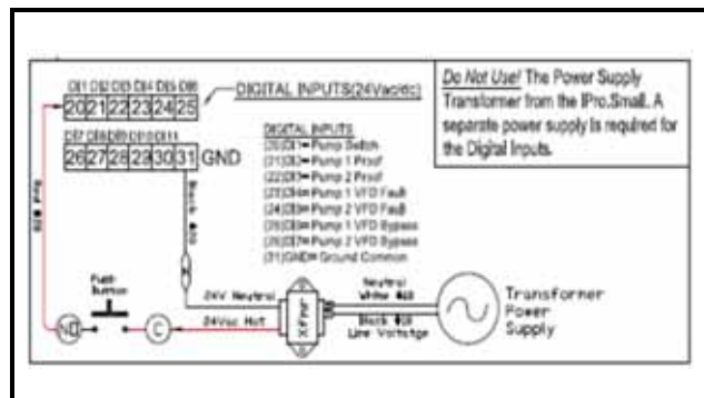
Figure 4-6 - Digital Input Wiring - 31 GND is Digital Common -
