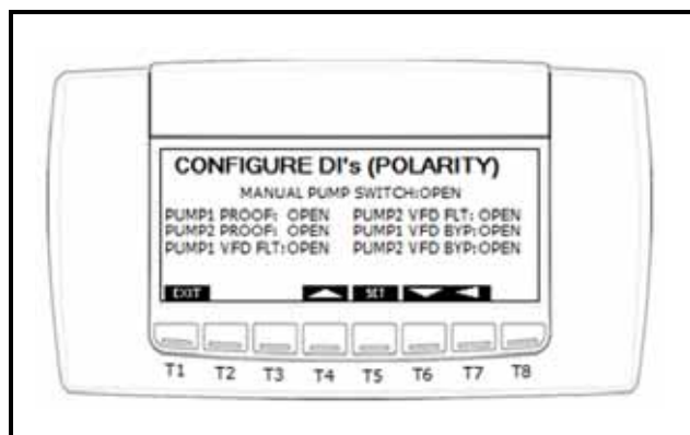
Figure 9-10 - Configure Digital Input's Polarity
