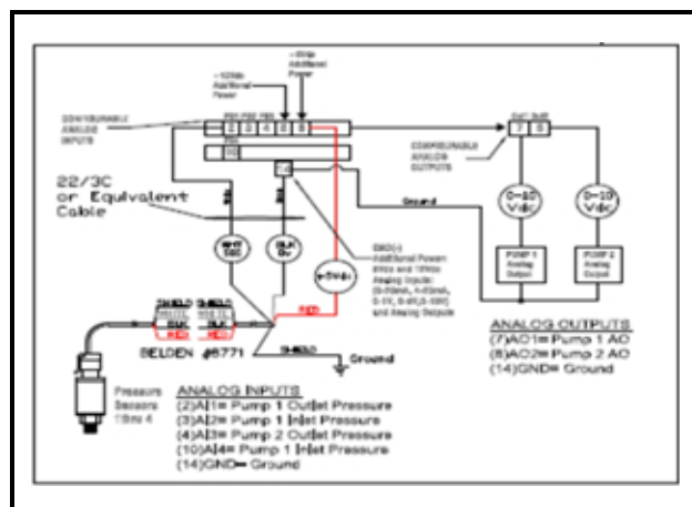
Figure 4-4 - Transducer Wiring for +5V Powered Devices and Analog Output Wiring
