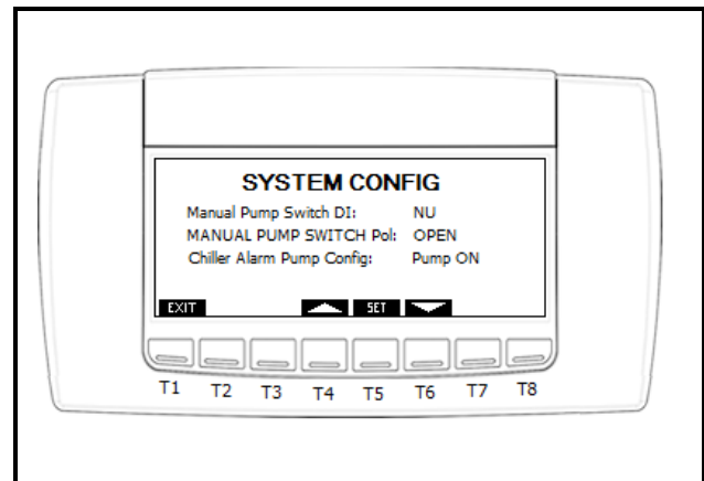
Figure 9-18 - System Configuration Page 3
