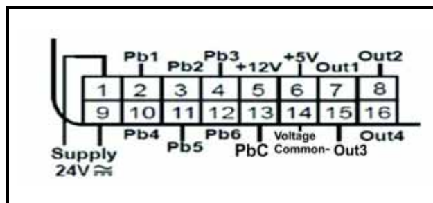
Figure 4-3 - Analog Inputs
