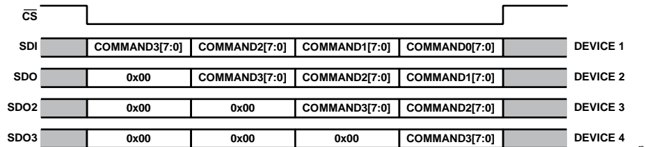
Figure 44. Example of an SPI Frame Where Four ADGS1414D Devices Connect in Daisy-Chain Mode
