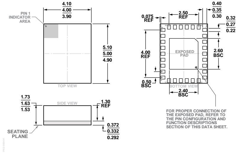
Figure 49. 30-Terminal Land Grid Array [LGA] (CC-30-3) 4 mm x 5 mm Body and 1.63 mm Package Height Dimensions shown in millimeters
