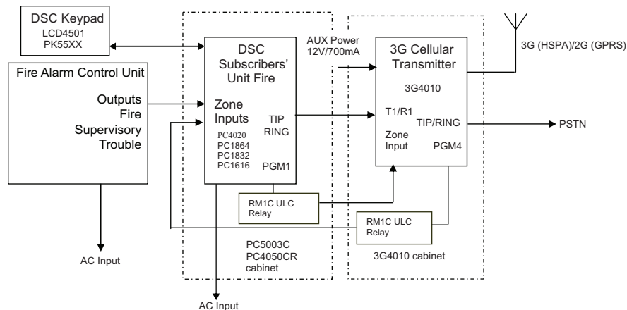
Figure 12-5 DSC Subscribers' Unit Fire and Cellular Transmitter Mounted in the Same Room
