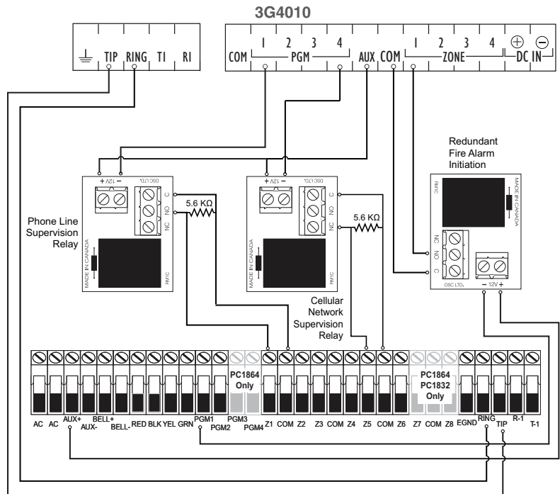
Figure 12-10 Connection Details for Cellular Network Supervision Relay, Phone Line Supervision Relay and Redundant Fire Alarm Transmission
