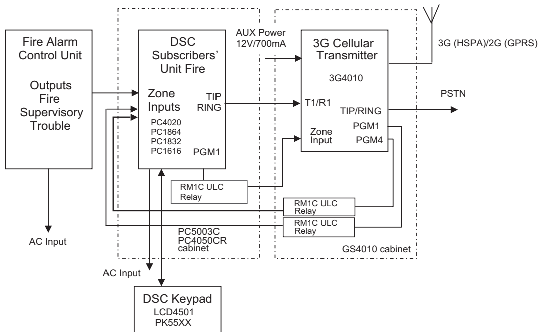
Figure 12-6 DSC Subscribers' Unit Fire and 3G Cellular Transmitter Mounted Remotely Alternate Wiring Diagram for DSC Subscribers' Unit Fire and Cellular Transmitter Passive Communication System - Using Phone Line Supervision Relay
