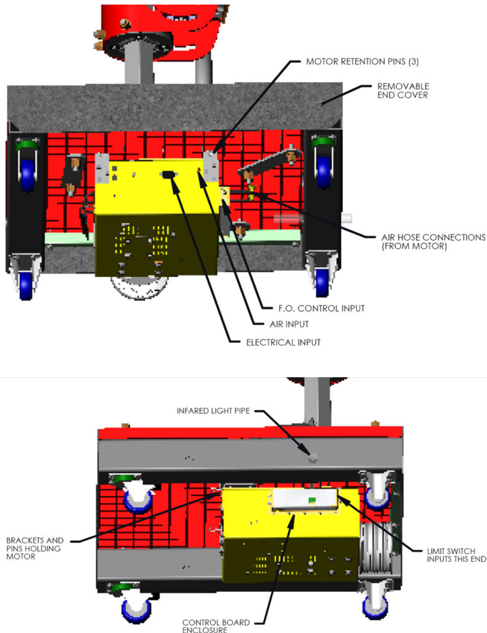
Figure 8: Location of Connections
