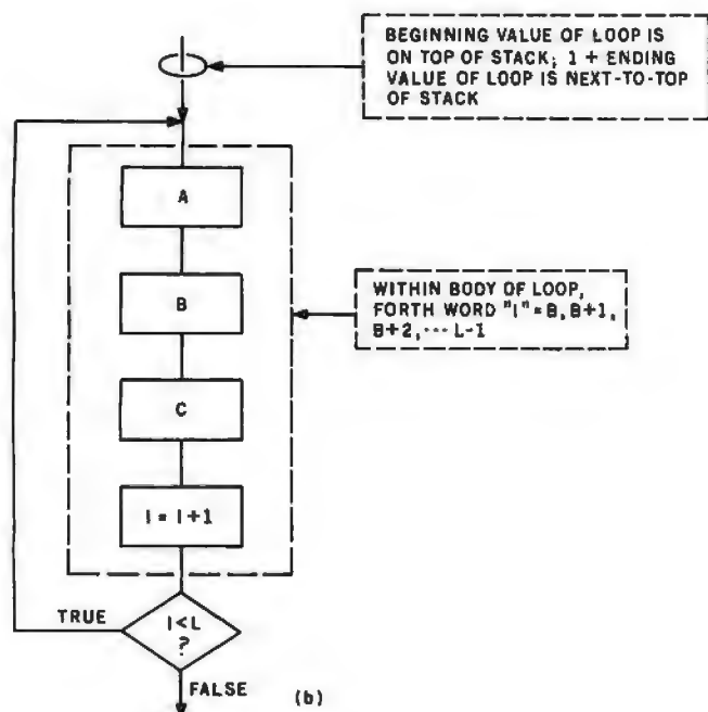
Figure 3: An explanation of the DO ... LOOP construct. As shown in figure 3a, the top number on the stack is taken to be the lower limit of the loop variable, I, and the next-to-top number on the stack is the upper limit of the loop variable + 1. The body of the loop is shaded, and the loop variable is incremented and tested after the body of the loop is executed. Figure 3b gives the equivalent construct in conventional flowchart notation.
