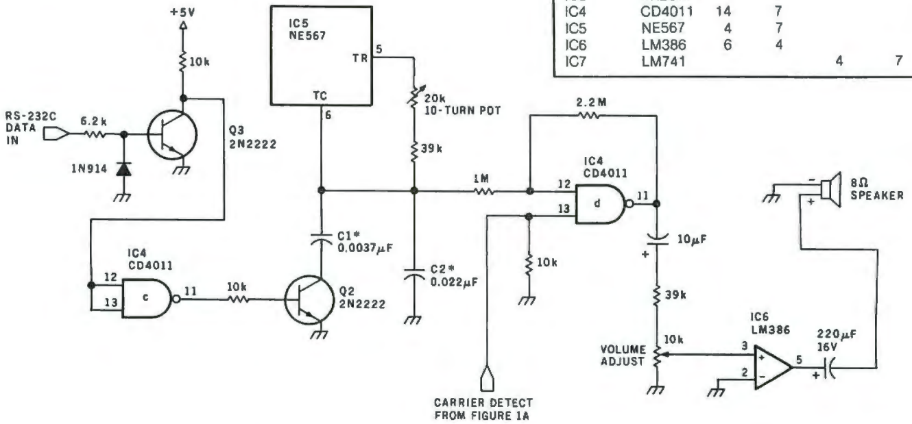
Figure 1b: Modulator section of the modem circuit in schematic form. The tone frequency for a mark (1270 Hz) is set up by choosing the proper values for capacitor C2 and adjusting the 20 k-ohm potentiometer. When transistor Q2 gates capacitor C1 in parallel with C2, the oscillator frequency changes to 1070 Hz.
