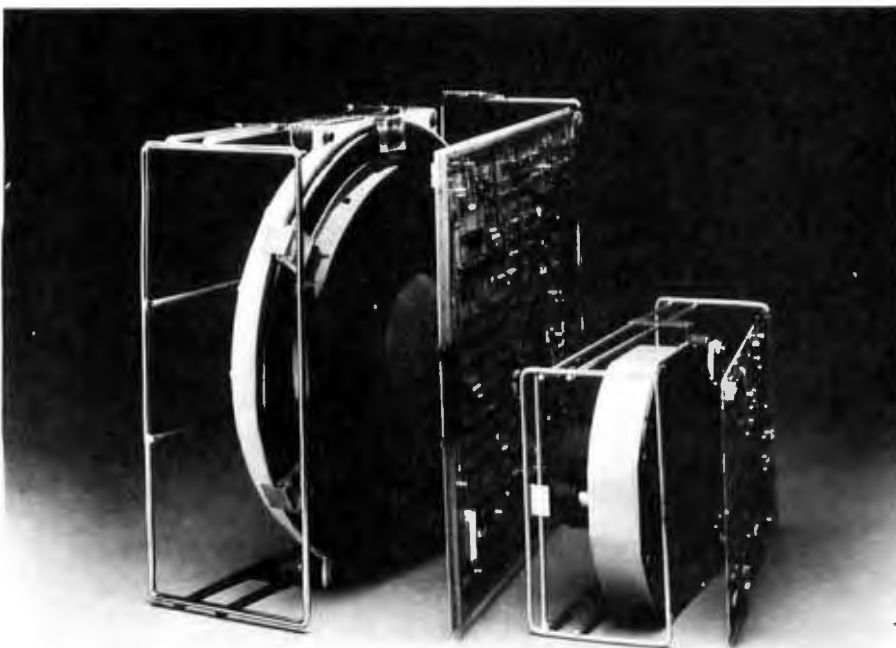
Photo 4: BASF Systems' 6170 Series 8-inch, fixed hard-disk drive, available in 8- and 24-megabyte versions. (Photo courtesy of BASF.)
