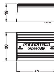
Crossover 2V2A
