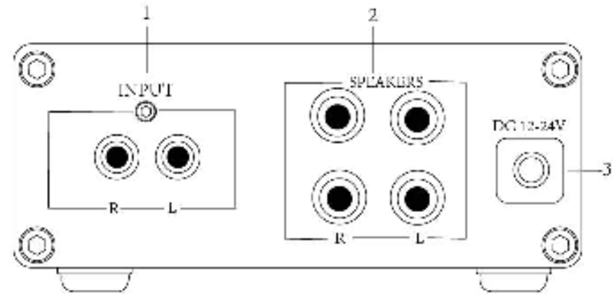
1..... 3.5mm AUX Input 3..... DC 12-24V Input 2..... Speaker Output
