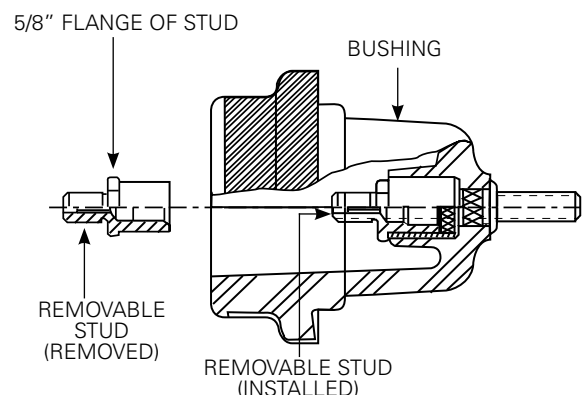
Figure 1. Removable stud bushing well shown with the removable stud both installed and removed.
