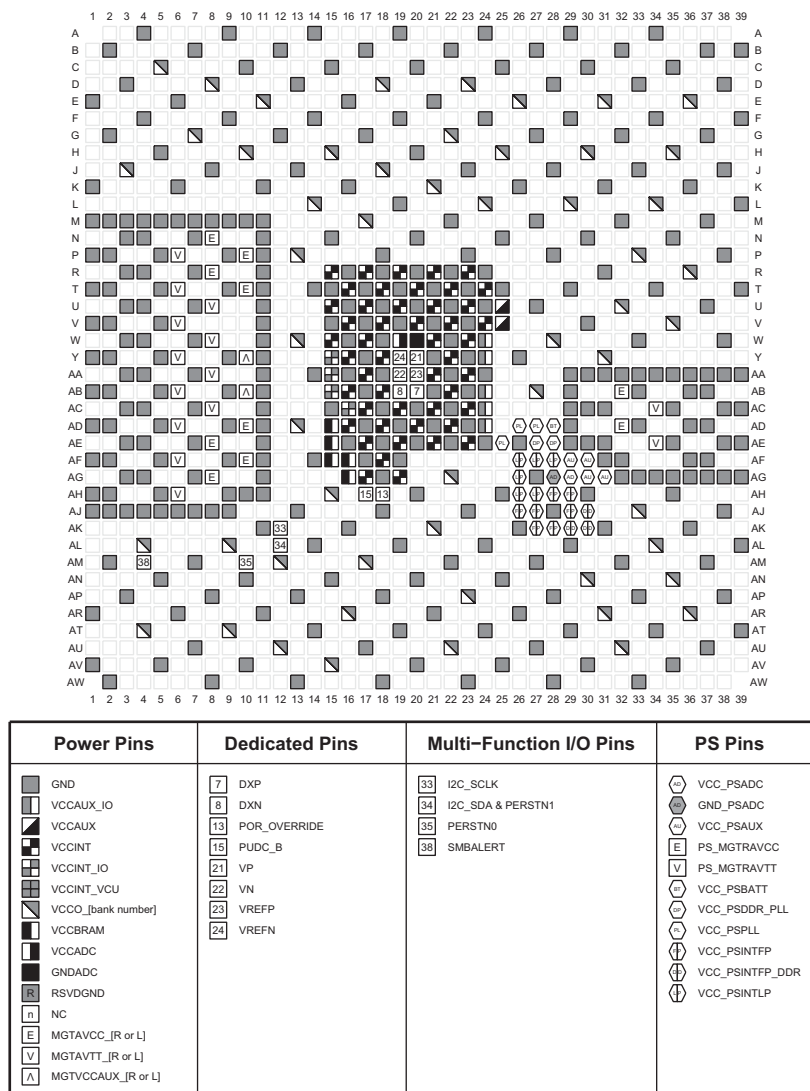
Figure 4-44: FFVB1517 Package—XCZU17EG and XCZU19EG Power, Dedicated, and Multi-function Pin Diagram
