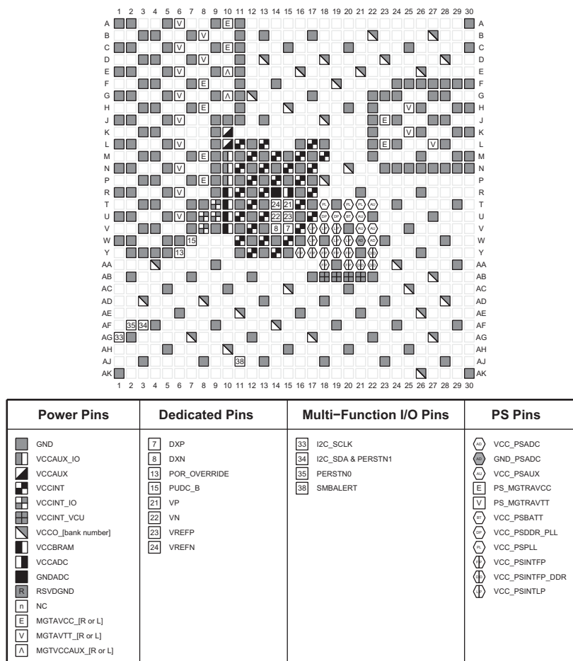
Figure 4-18: FBVB900 Package—XCZU7EV Power, Dedicated, and Multi-function Pin Diagram
