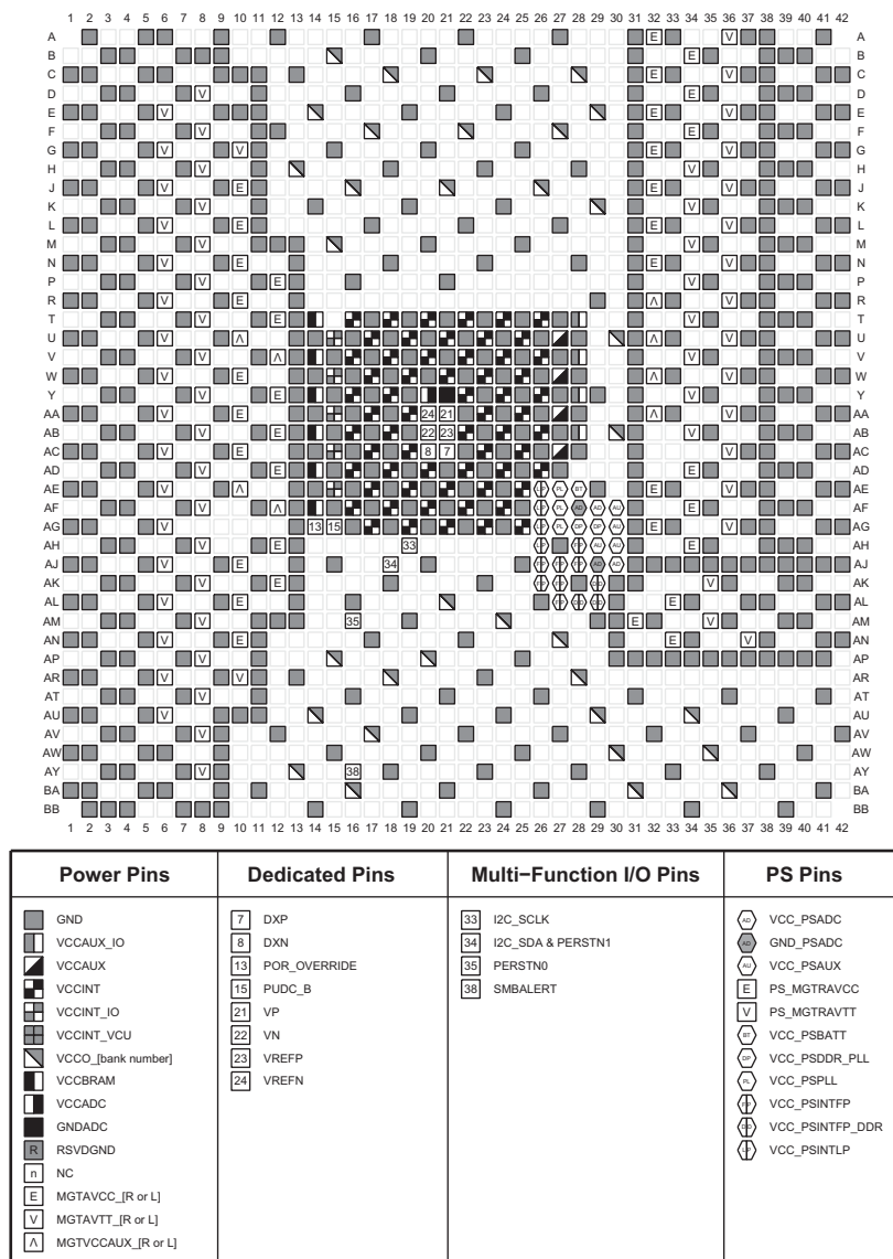
Figure 4-66: FFVD1760 Package—XCZU17EG and XCZU19EG Power, Dedicated, and Multi-function Pin Diagram
