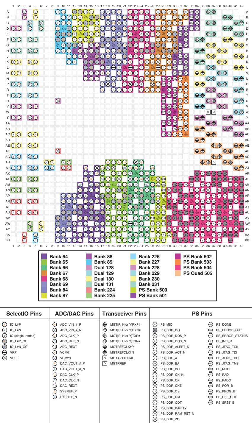
Figure 4-69: FFVF1760 and FSVF1760 Packages—XCZU49DR I/O Bank Diagram
