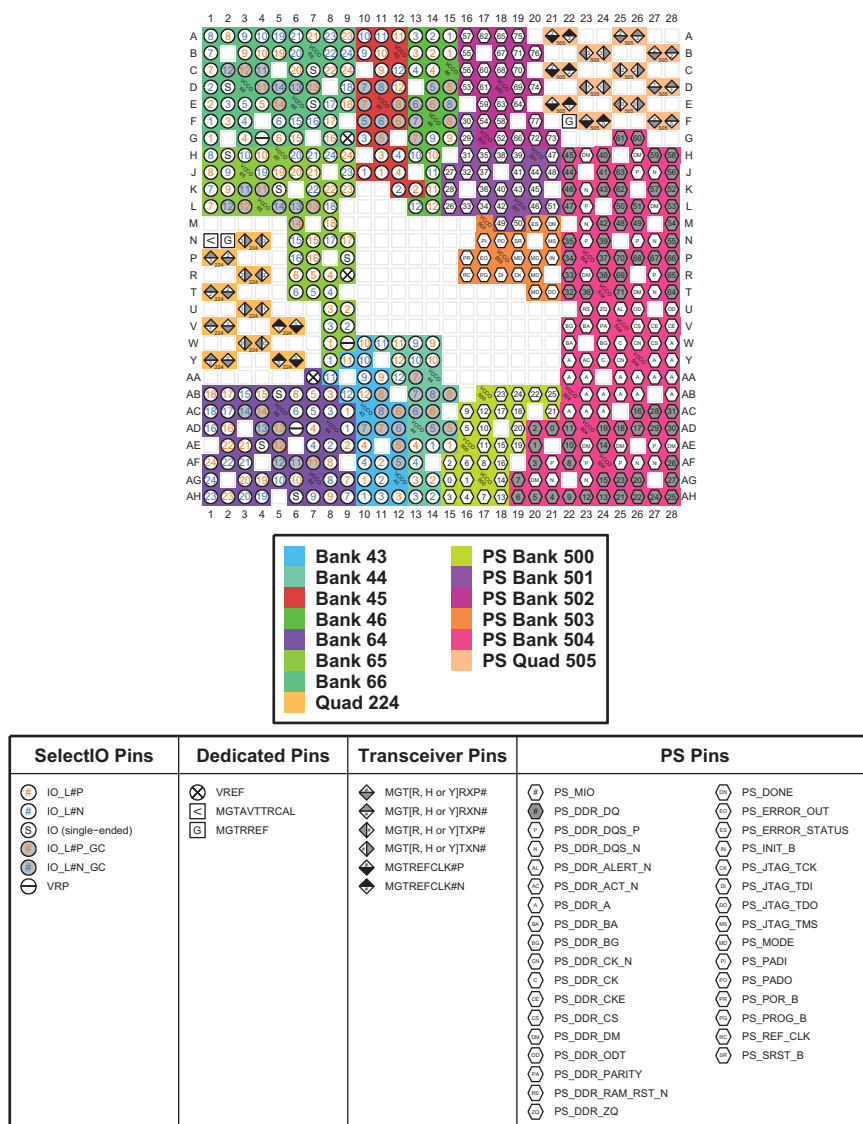
Figure 4-9: SFVC784 Package—XCZU4EV, XCZU5EV, XAZU4EV, and XAZU5EV I/O Bank Diagram
