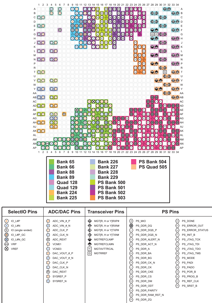
Figure 4-31: FFVE1156 and FSVE1156 Packages—XCZU25DR I/O Bank Diagram
