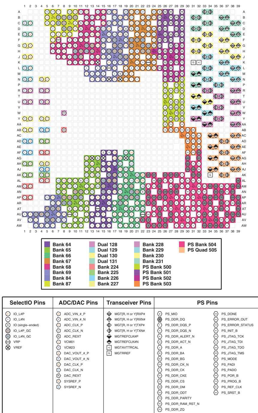
Figure 4-59: FFVG1517 and FSVG1517 Packages—XCZU48DR I/O Bank Diagram
