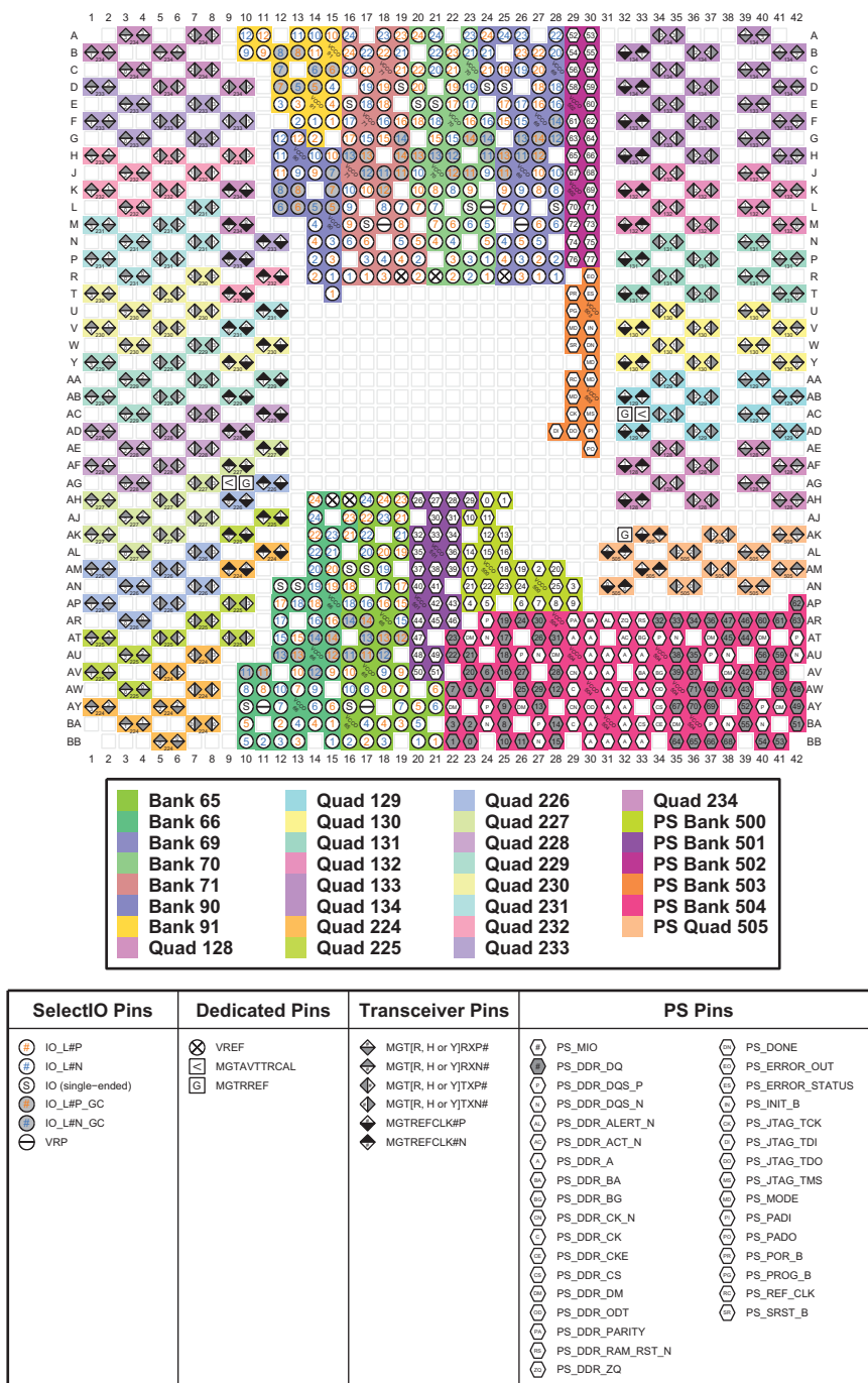
Figure 4-65: FFVD1760 Package—XCZU17EG and XCZU19EG I/O Bank Diagram
