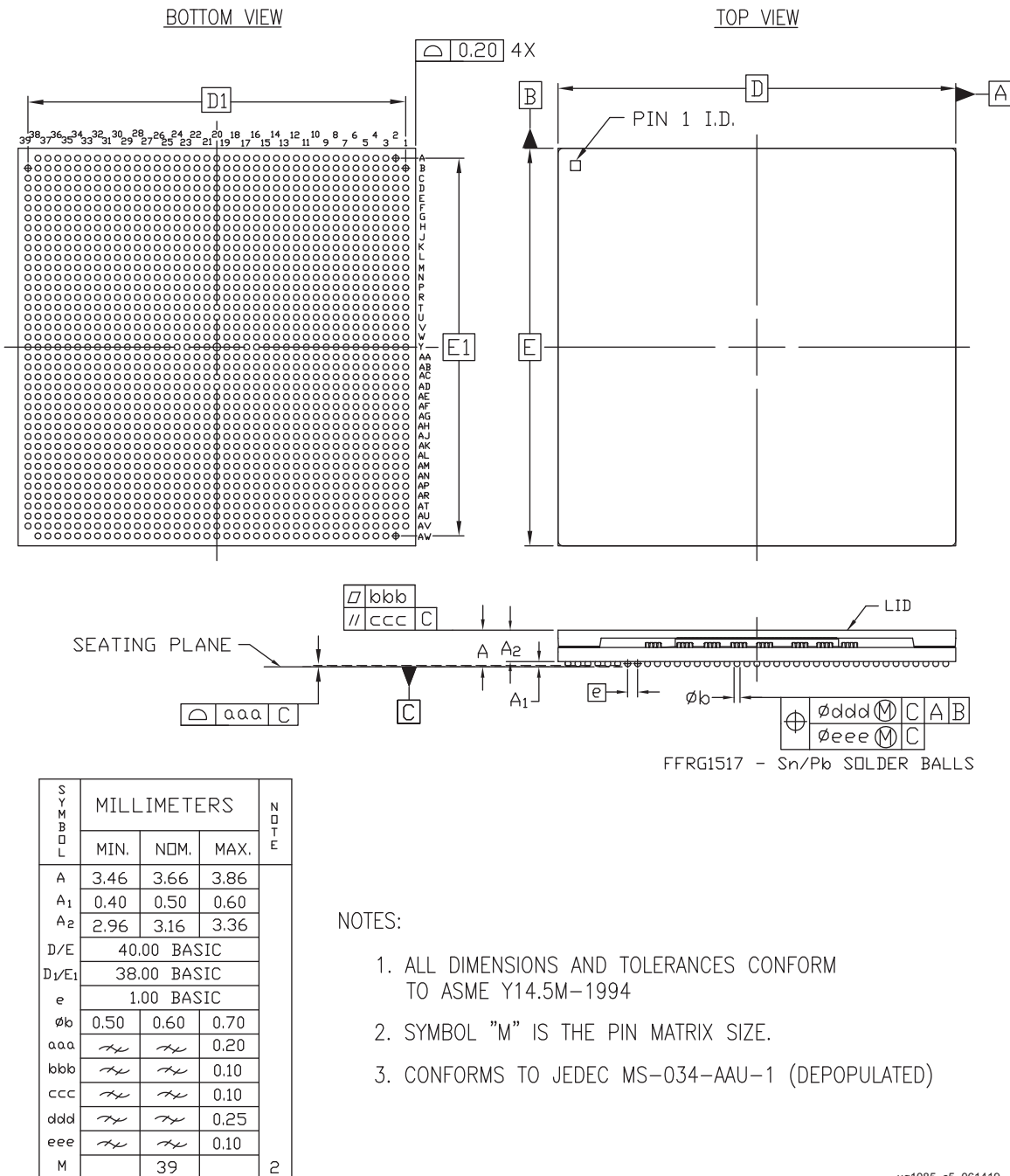
Figure 5-21: Package Dimensions for FFRG1517 (XQZU28DR)
