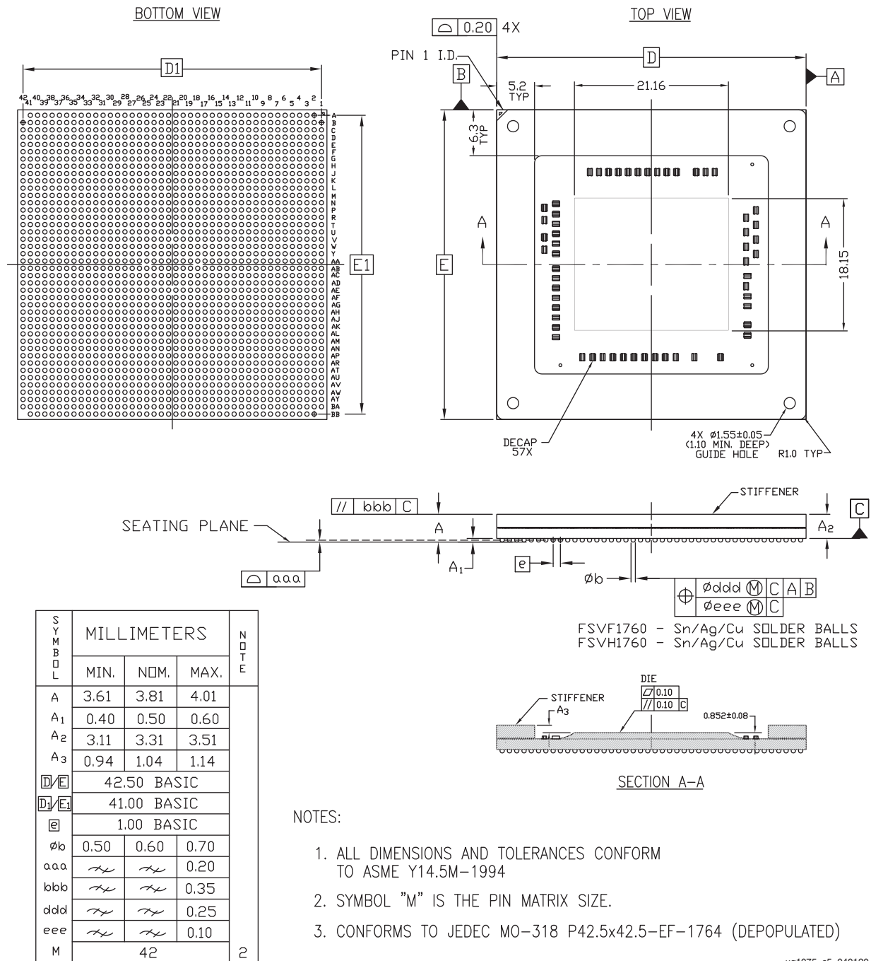
Figure 5-28: Package Dimensions for FSVF1760 (XCZU29DR, XCZU39DR, XCZU49DR) and FSVH1760 (XCZU46DR)
