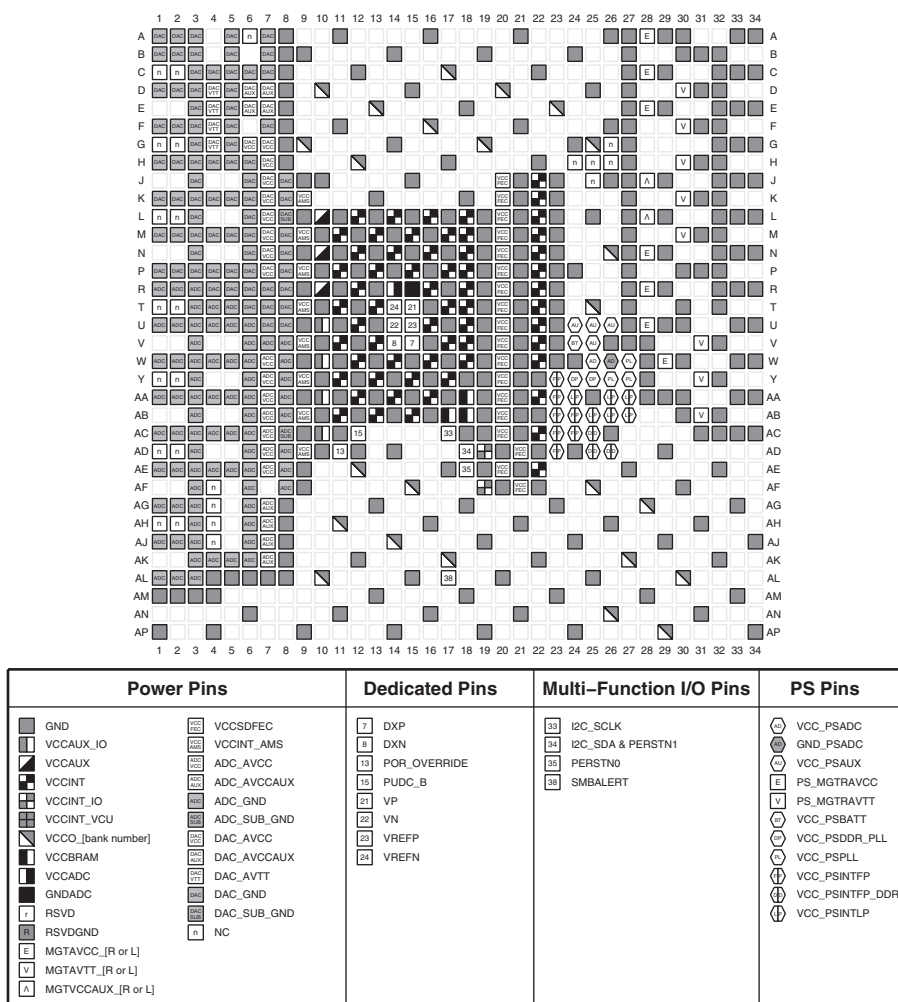
Figure 4-36: FFVE1156 and FSVE1156 Packages—XCZU43DR Power, Dedicated, and Multi-function Pin Diagram
