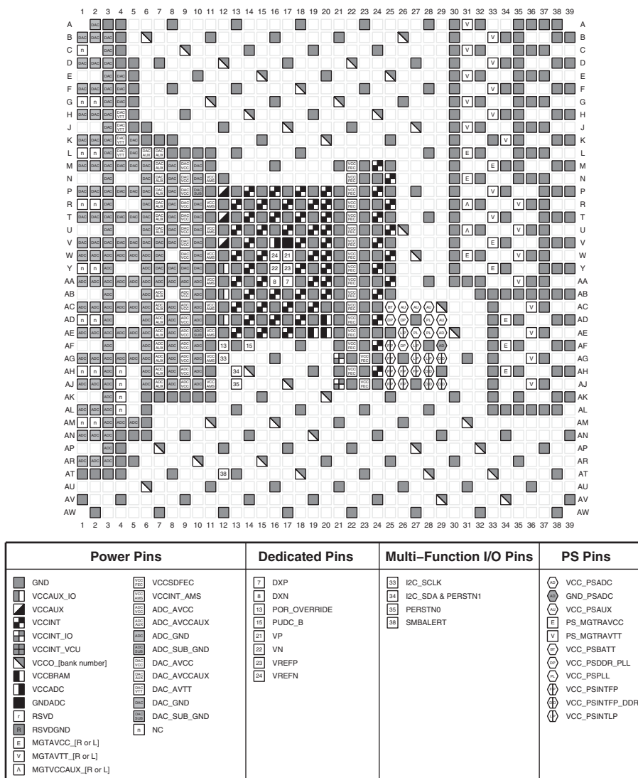
Figure 4-56: FFVG1517 and FSVG1517 Packages—XCZU43DR Power, Dedicated, and Multi-function Pin Diagram
