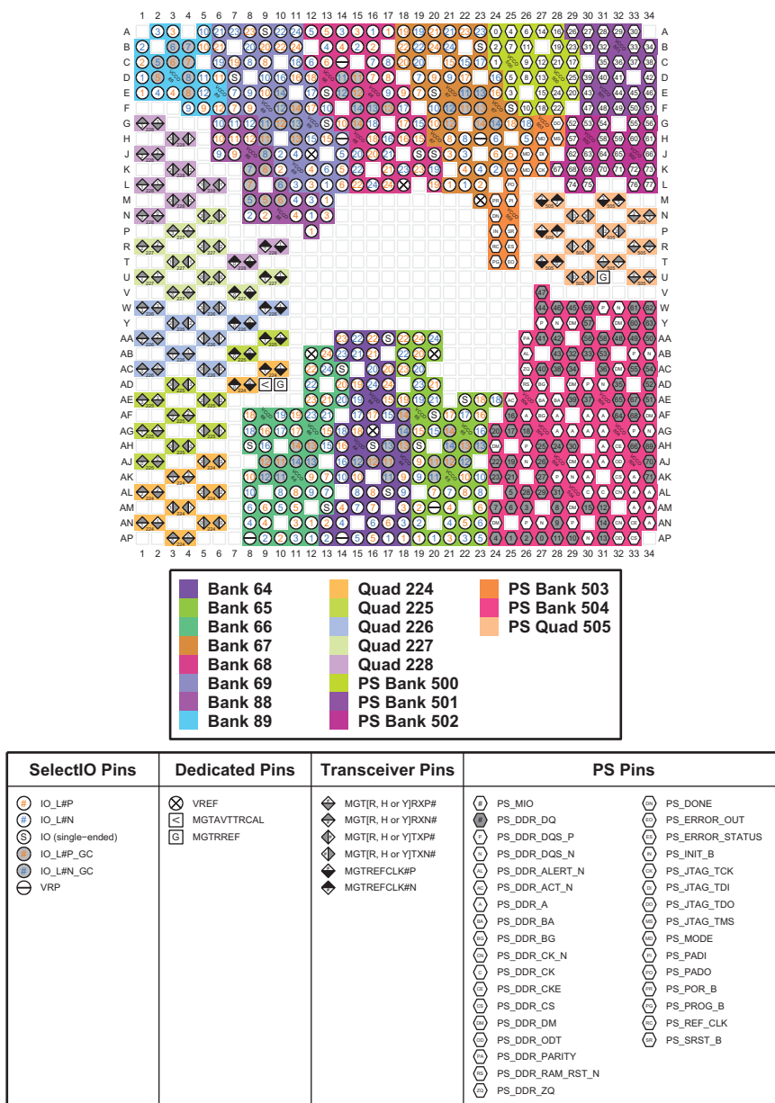
Figure 4-27: FFVC1156 Package—XCZU11EG I/O Bank Diagram
