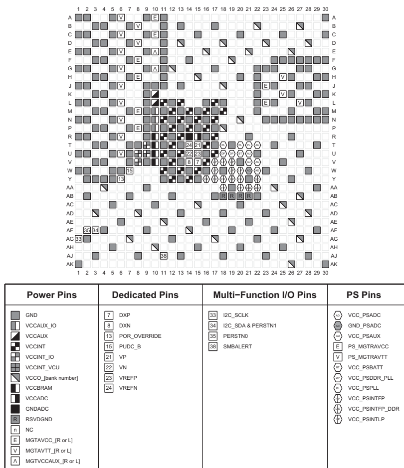
Figure 4-12: FBVB900 Package—XCZU4CG, XCZU4EG, XCZU5CG, and XCZU5EG Power, Dedicated, and Multi-function Pin Diagram
