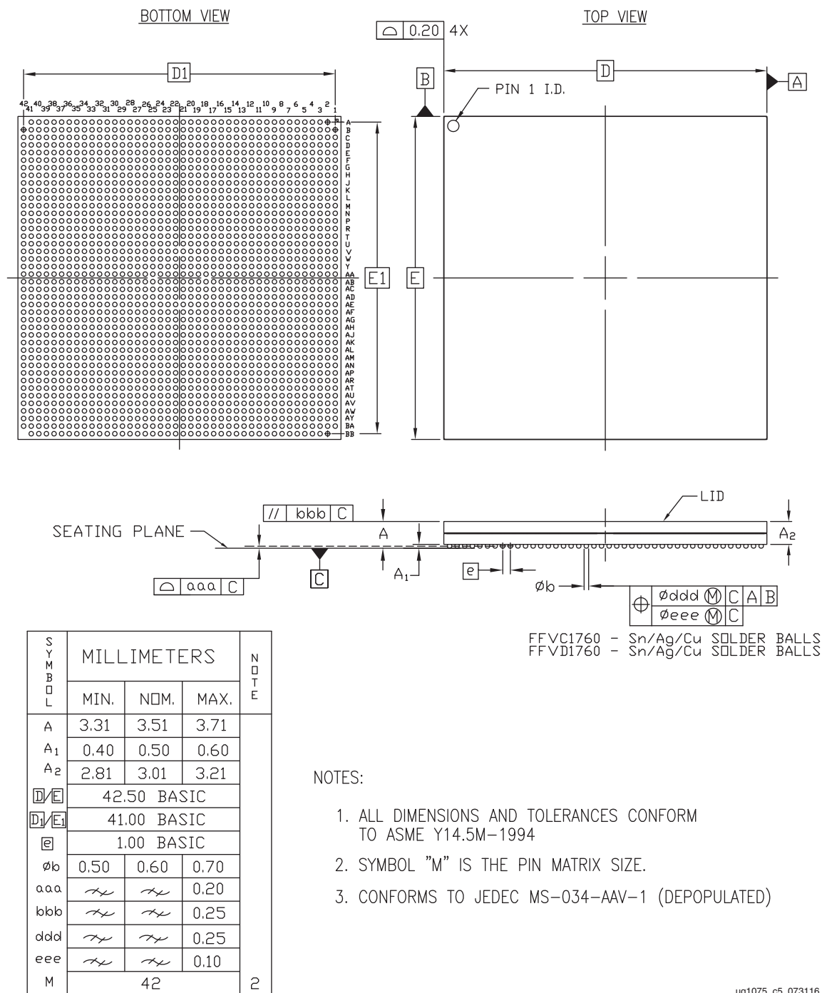
Figure 5-24: Package Dimensions for FFVC1760 and FFVD1760 (XCZU11EG, XCZU17EG, and XCZU19EG)
