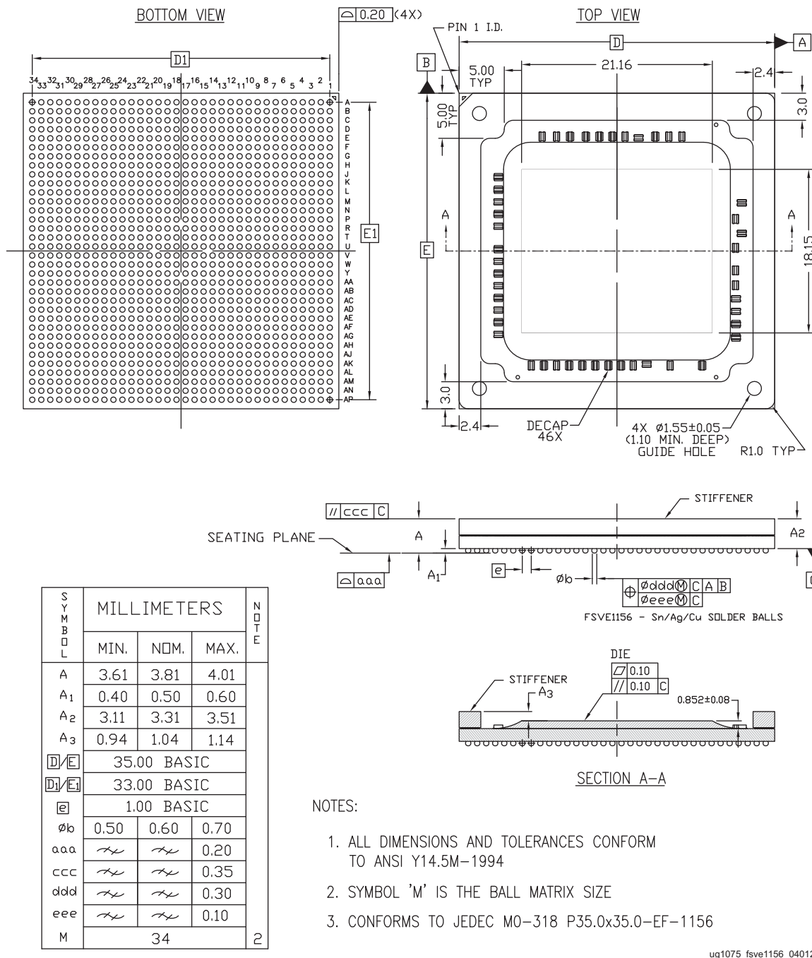
Figure 5-18: Package Dimensions for FSVE1156 (XCZU25DR, XCZU27DR, XCZU28DR, XCZU43DR, XCZU47DR, XCZU48DR)
