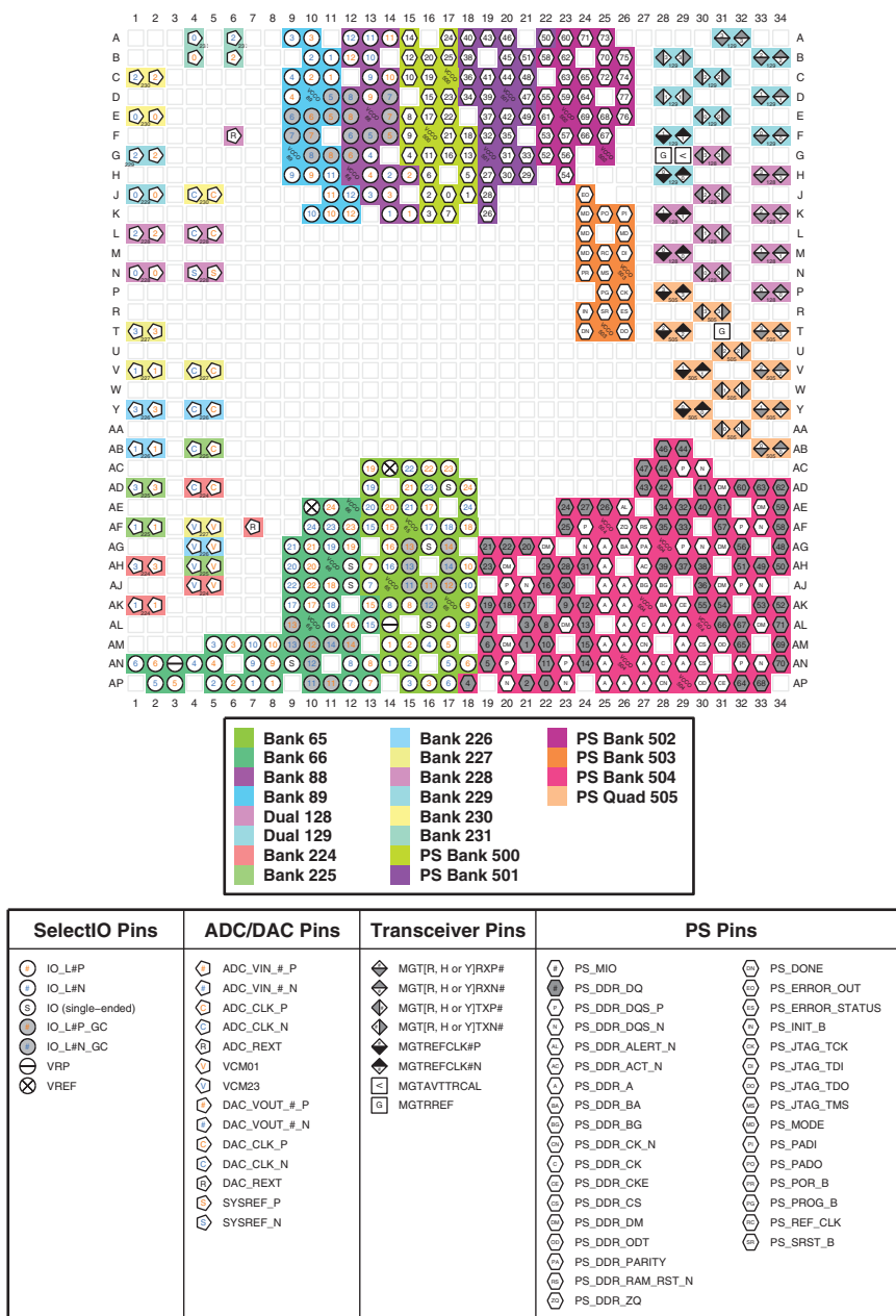
Figure 4-37: FFVE1156 and FSVE1156 Packages—XCZU47DR I/O Bank Diagram
