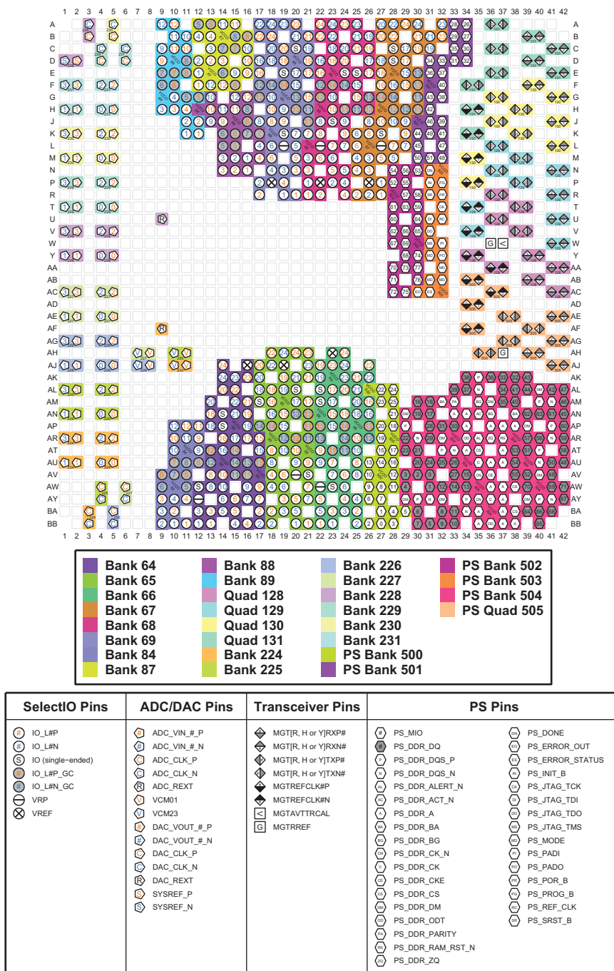
Figure 4-67: FFVF1760 and FSVF1760 Packages—XCZU29DR and XCZU39DR I/O Bank Diagram
