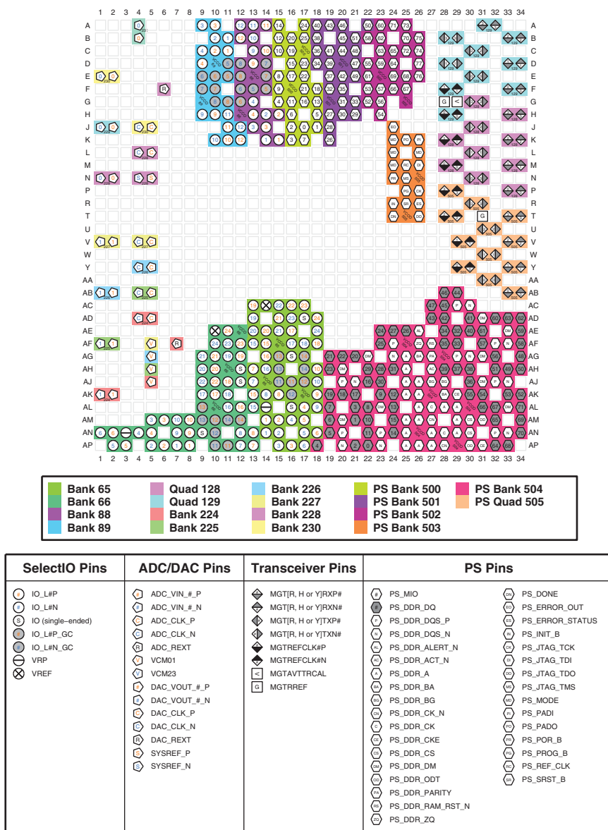
Figure 4-35: FFVE1156 and FSVE1156 Packages—XCZU43DR I/O Bank Diagram
