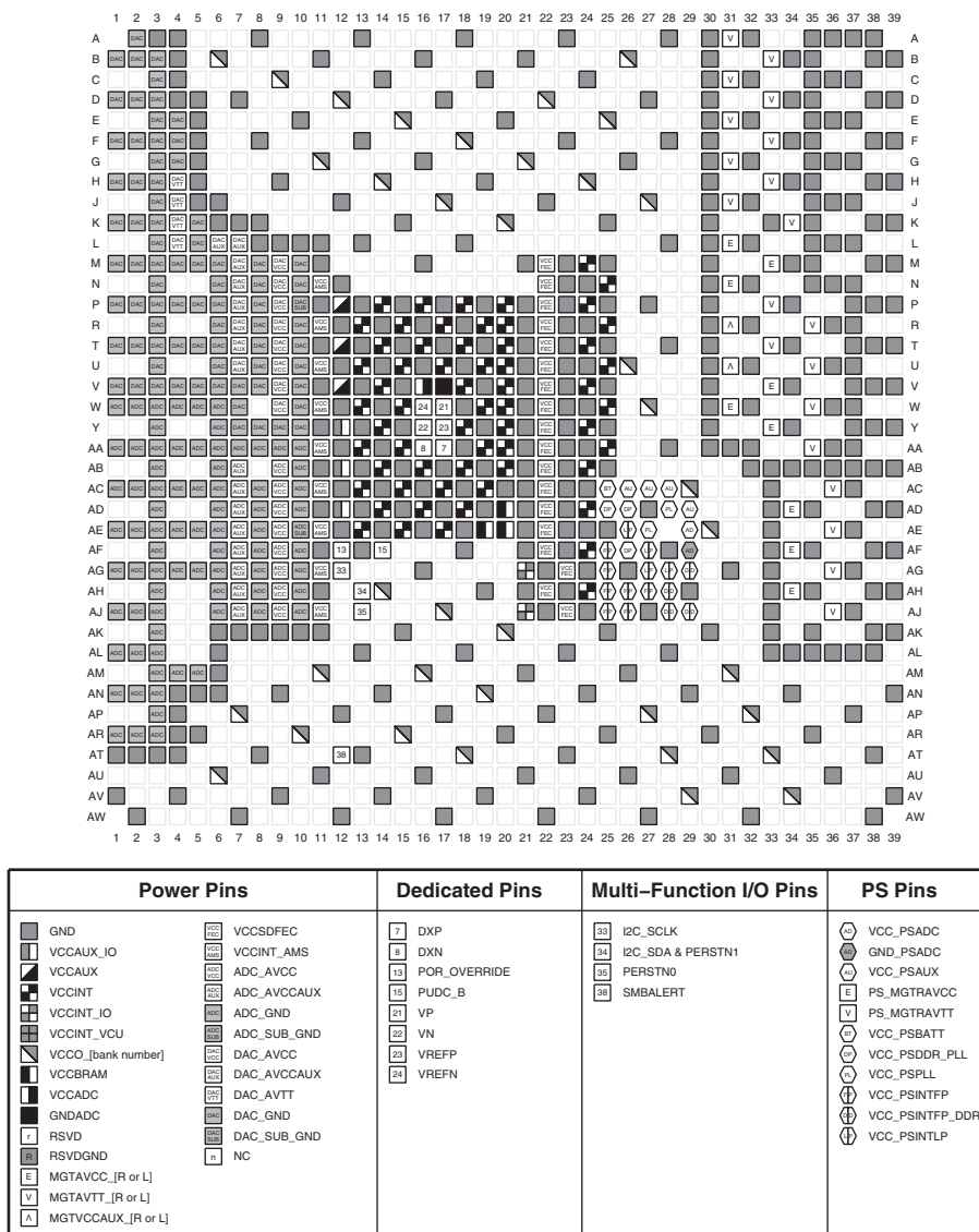
Figure 4-60: FFG1517 and FSVG1517 Packages—XCZU48DR Power, Dedicated, and Multi-function Pin Diagram
