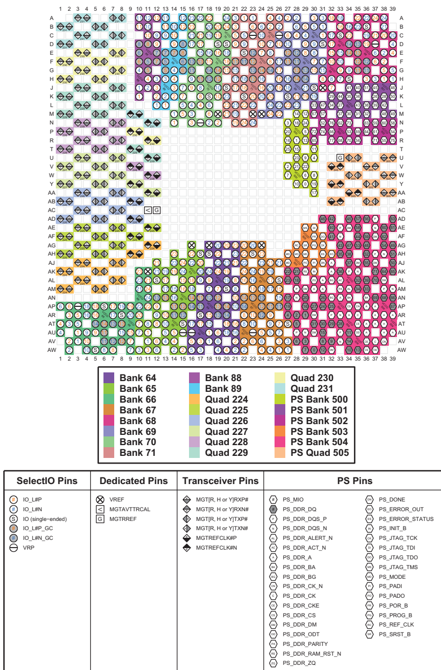
Figure 4-49: FFVF1517 Package—XCZU11EG I/O Bank Diagram
