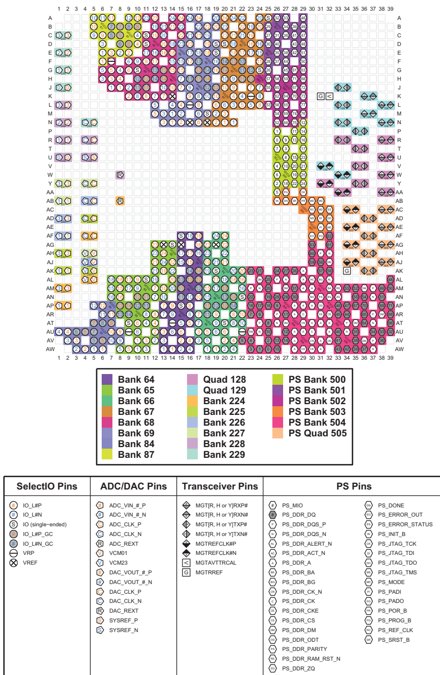
Figure 4-51: FFVG1517 and FSVG1517 Packages—XCZU25DR I/O Bank Diagram
