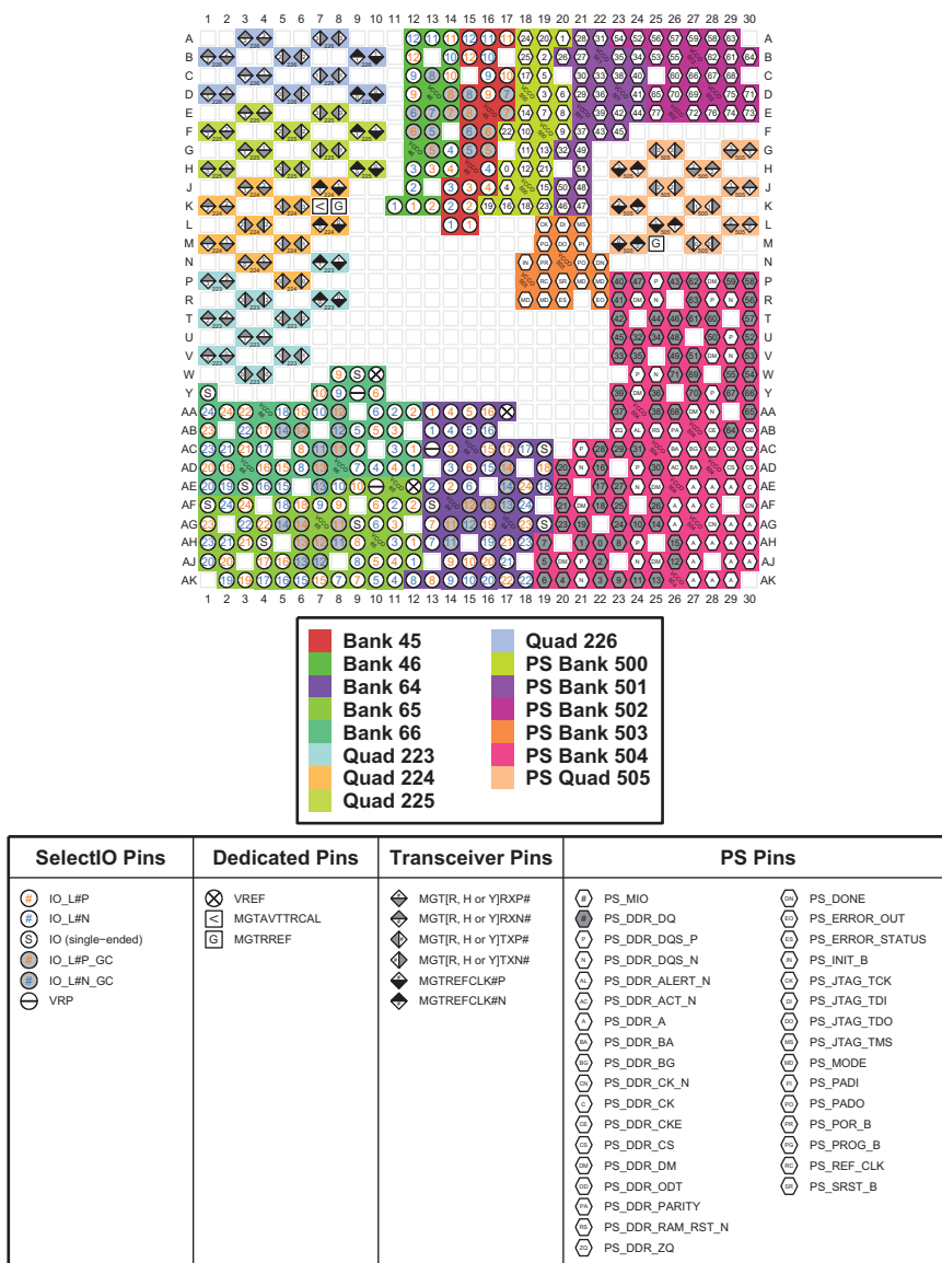
Figure 4-13: FBVB900 Package—XCZU4EV and XCZU5EV I/O Bank Diagram
