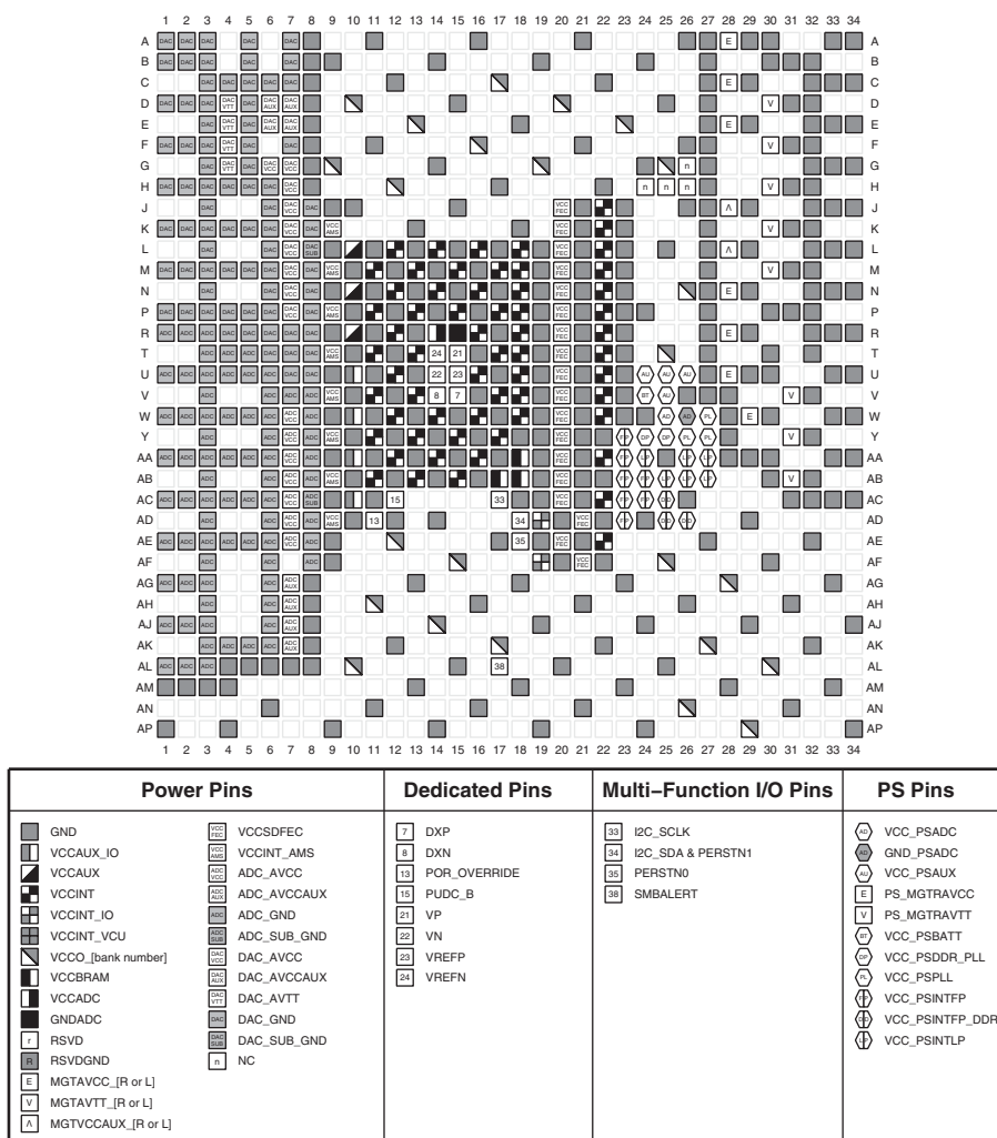
Figure 4-40: FFVE1156 and FSVE1156 Packages—XCZU48DR Power, Dedicated, and Multi-function Pin Diagram
