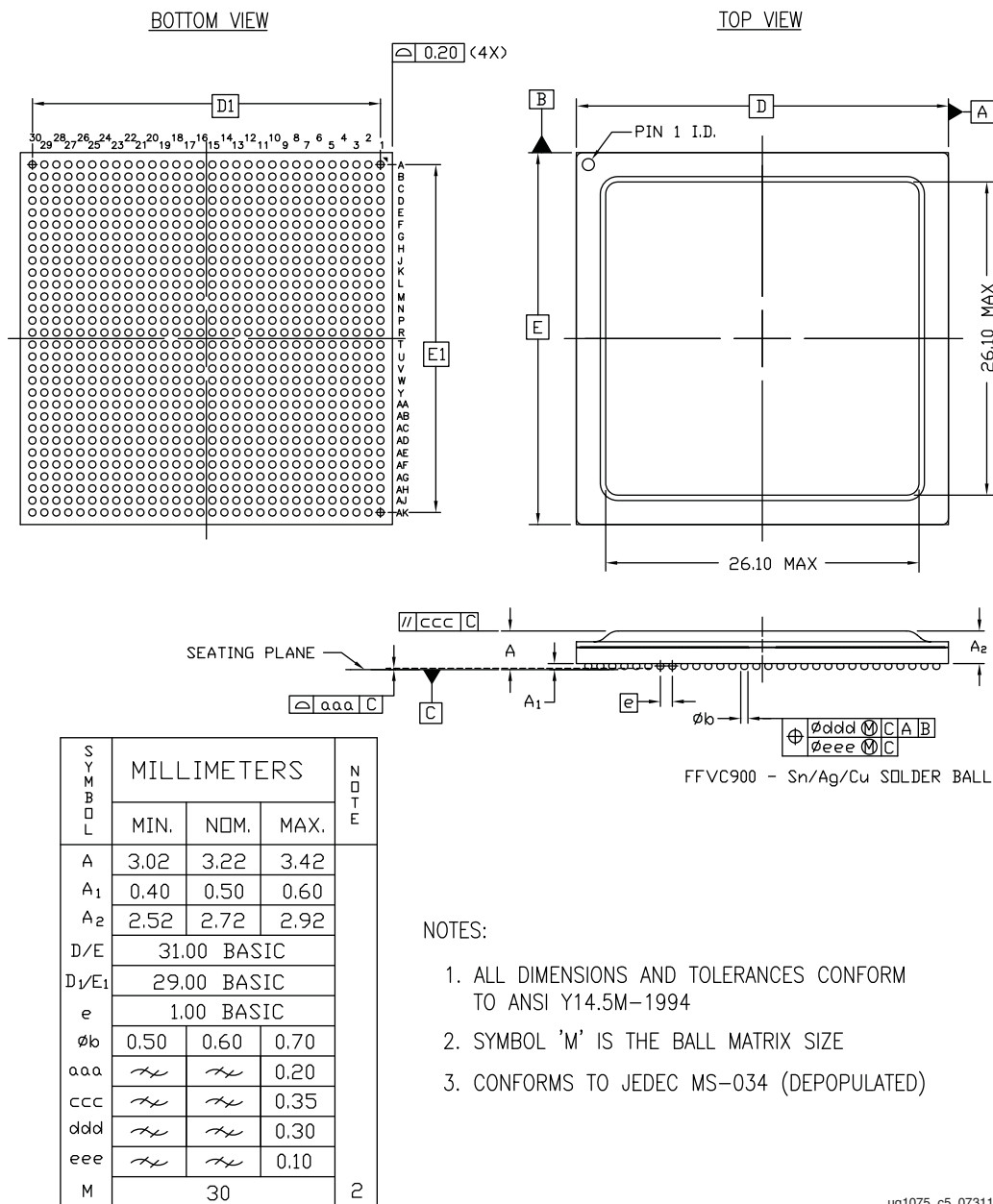
Figure 5-10: Package Dimensions for FFVC900 (XCZU6CG, XCZU6EG, XCZU9CG, XCZU9EG, and XCZU15EG)
