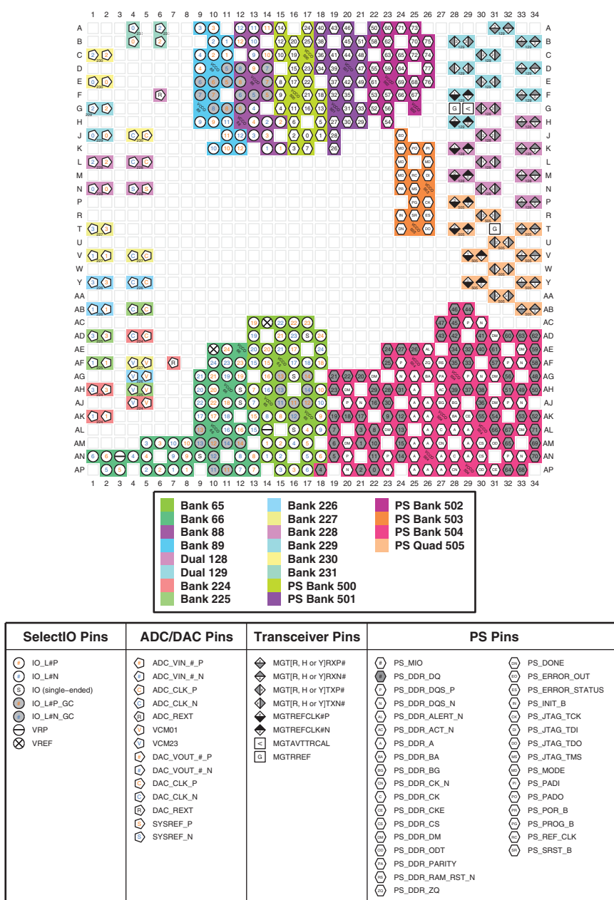
Figure 4-39: FFVE1156 and FSVE1156 Packages—XCZU48DR I/O Bank Diagram
