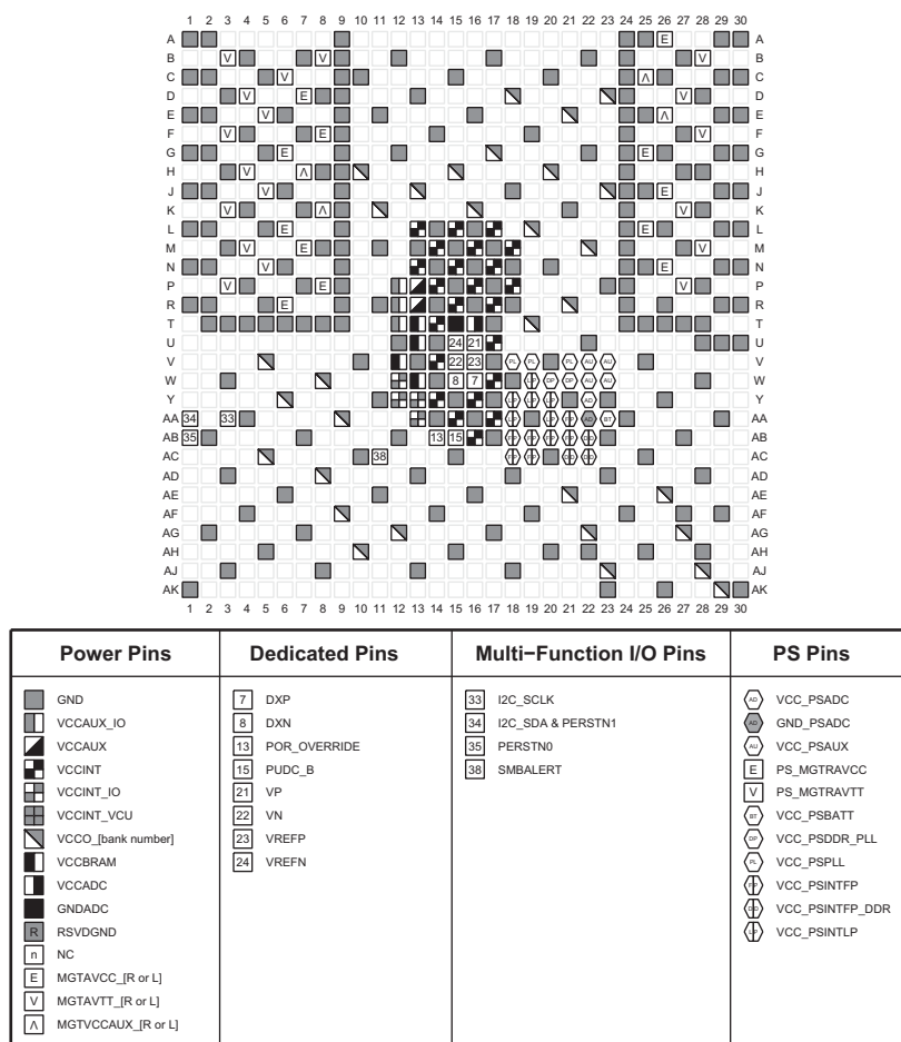
Figure 4-20: FVC900 Package—XCZU6EG, XCZU9EG, and XCZU15EG Power, Dedicated, and Multi-function Pin Diagram
