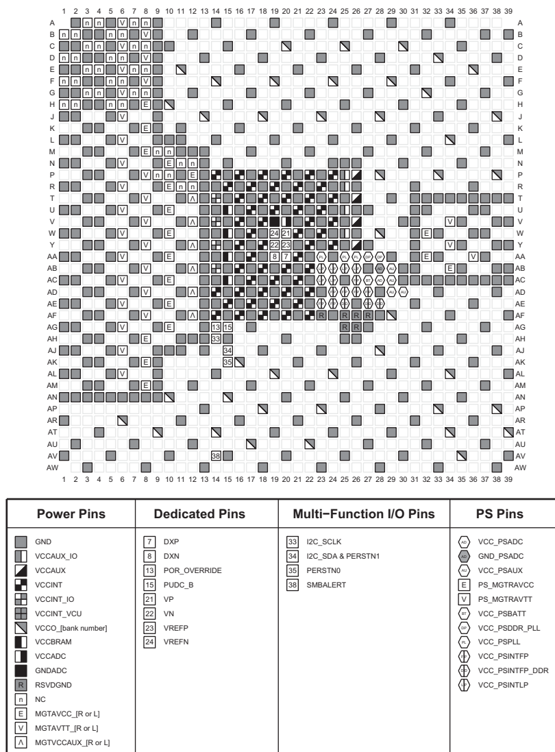
Figure 4-46: FFVF1517 Package—XCZU7CG and XCZU7EG Power, Dedicated, and Multi-function Pin Diagram
