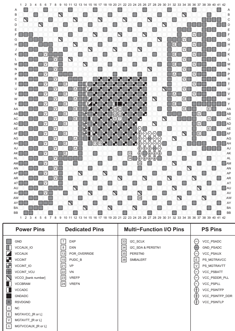
Figure 4-64: FFVC1760 Package—XCZU17EG and XCZU19EG Power, Dedicated, and Multi-function Pin Diagram
