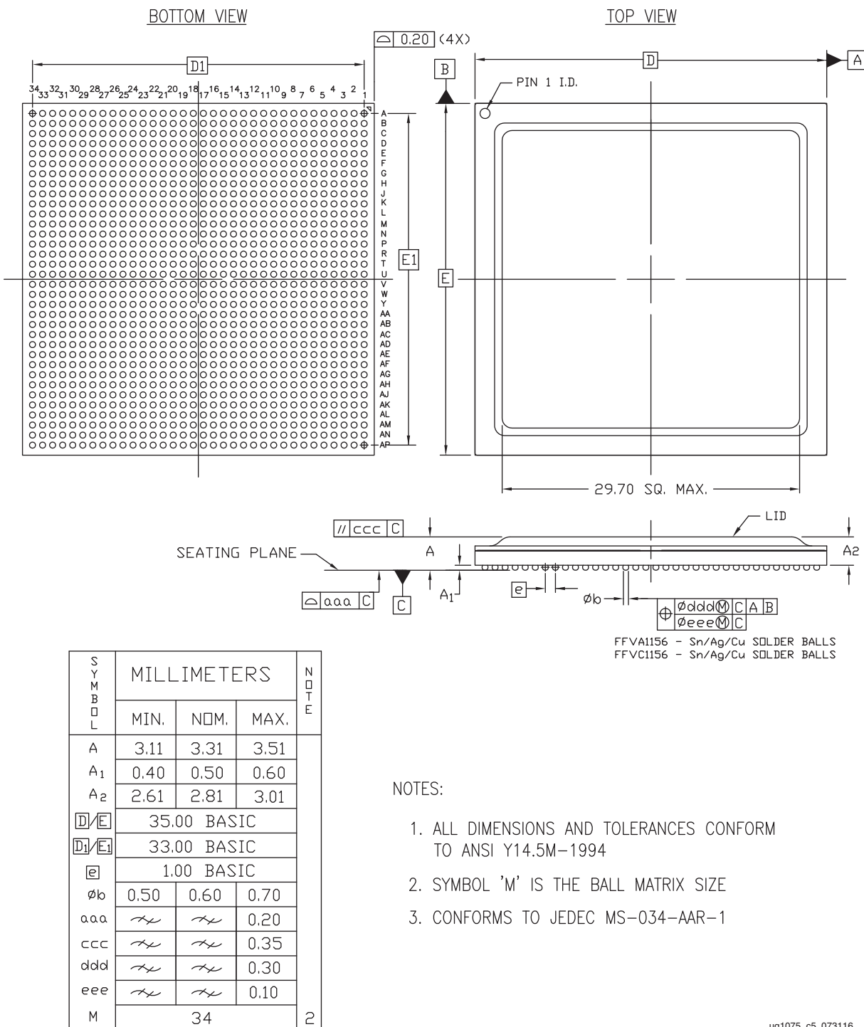
Figure 5-14: Package Dimensions for FFVC1156 (XCZU7CG, XCZU7EG, XCZU7EV, and XCZU11EG)
