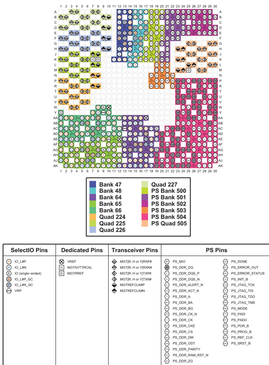
Figure 4-15: FBVB900 Package—I/O Bank Diagram
