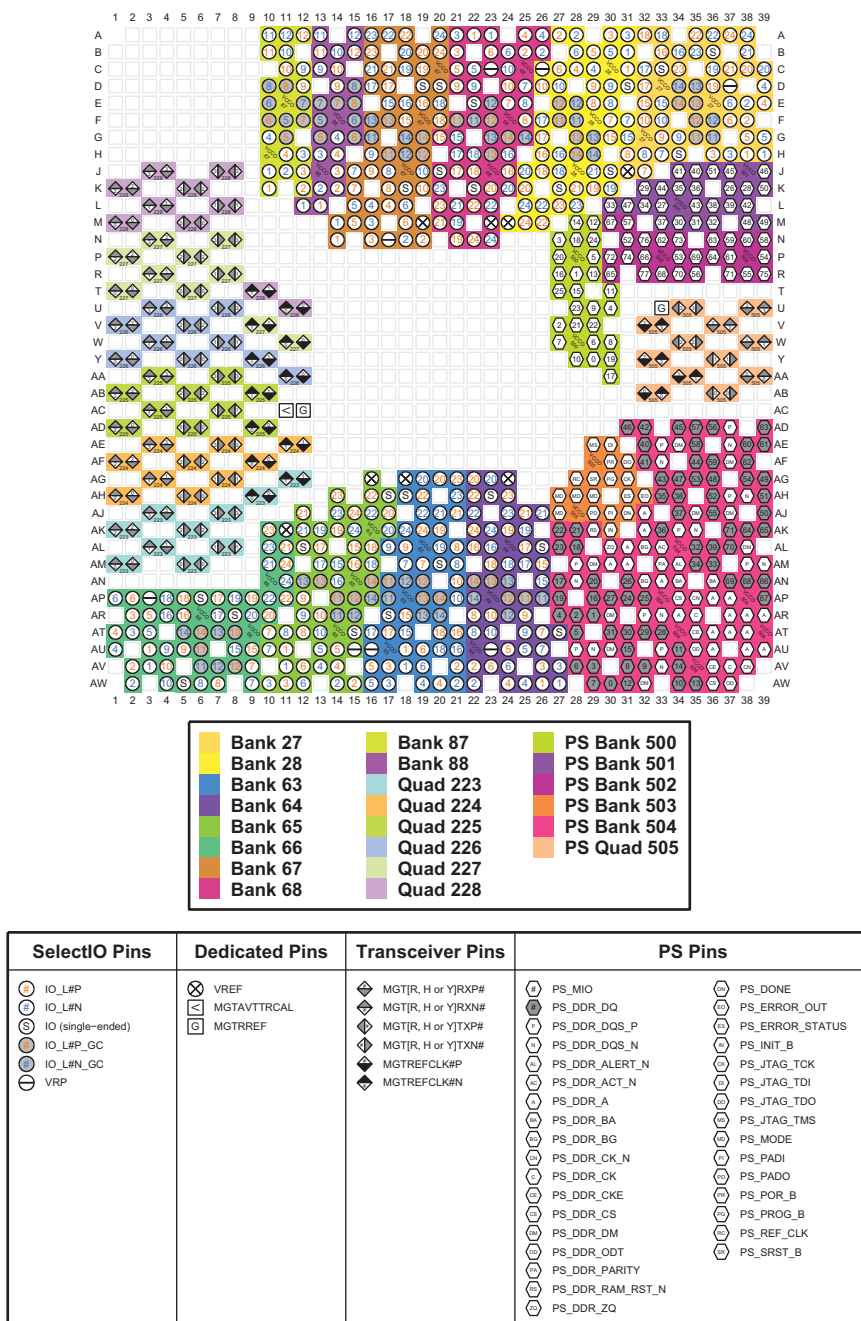
Figure 4-45: FFVF1517 Package—XCZU7CG and XCZU7EG I/O Bank Diagram
