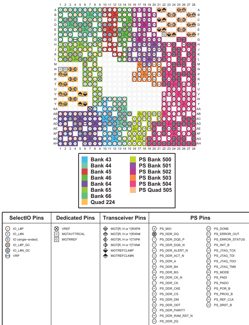
Figure 4-7: SFVC784 Package—XCZU4CG, XCZU4EG, XCZU5CG, and XCZU5EG I/O Bank Diagram
