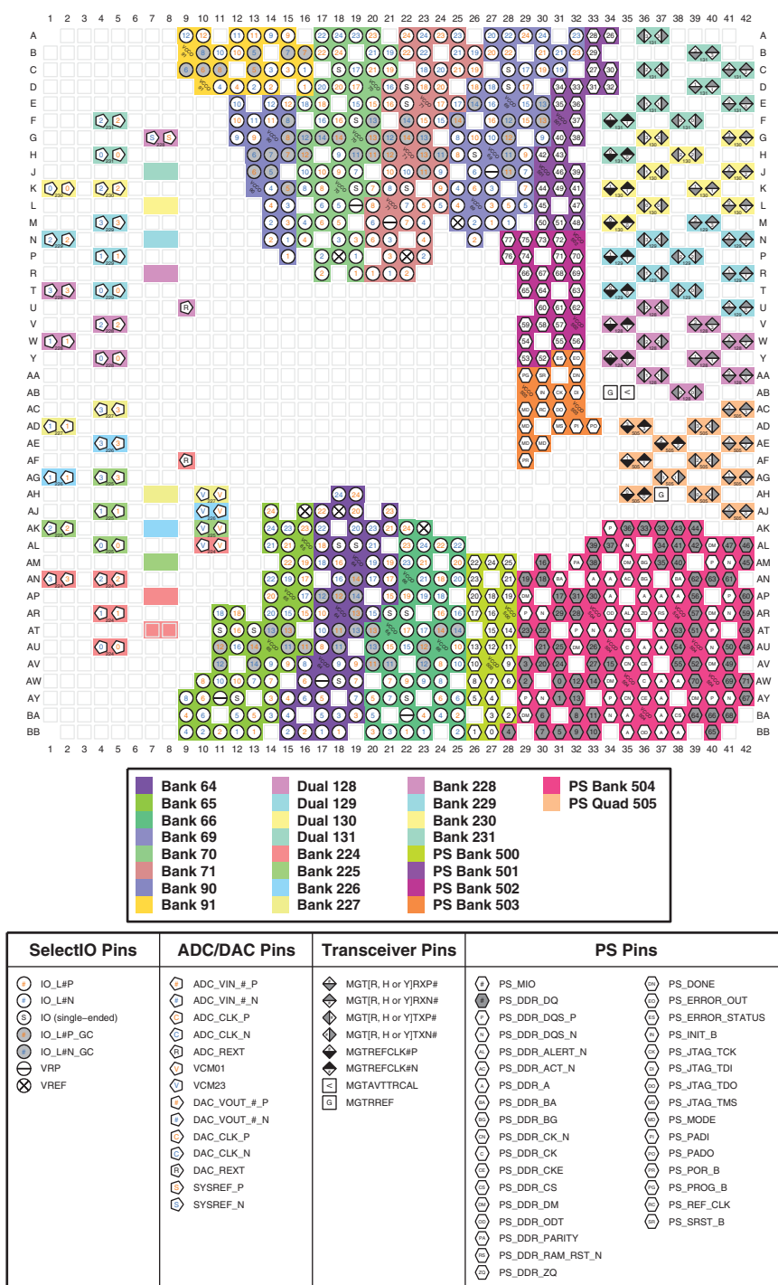
Figure 4-71: FFVH1760 and FSVH1760 Packages—XCZU49DR I/O Bank Diagram
