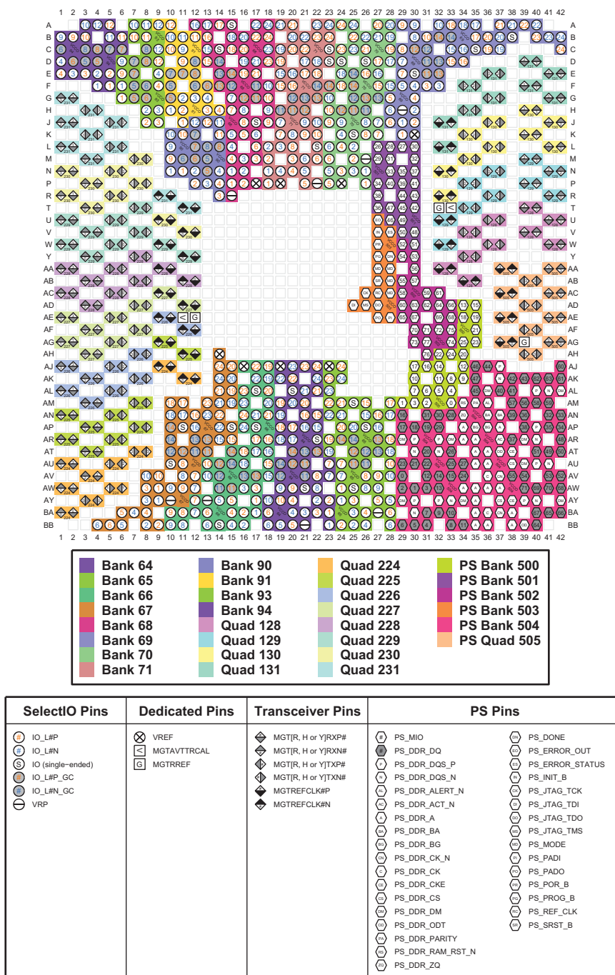
Figure 4-63: FFVC1760 Package—XCZU17EG and XCZU19EG I/O Bank Diagram
