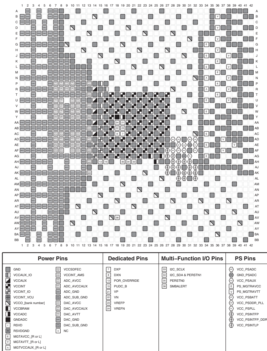
Figure 4-70: FFVF1760 and FSVF1760 Packages—XCZU49DR Power, Dedicated, and Multi-function Pin Diagram
