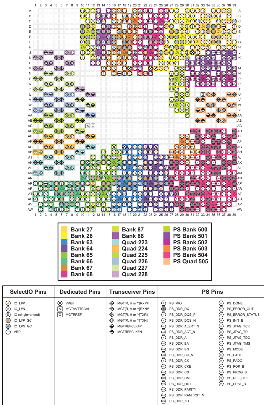
Figure 4-47: FFVF1517 Package—XCZU7EV I/O Bank Diagram
