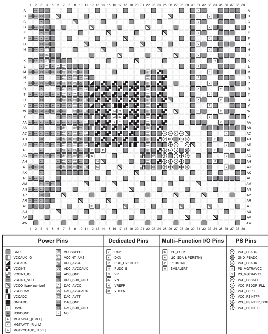
Figure 4-58: FFVG1517 and FSVG1517 Packages—XCZU47DR Power, Dedicated, and Multi-function Pin Diagram
