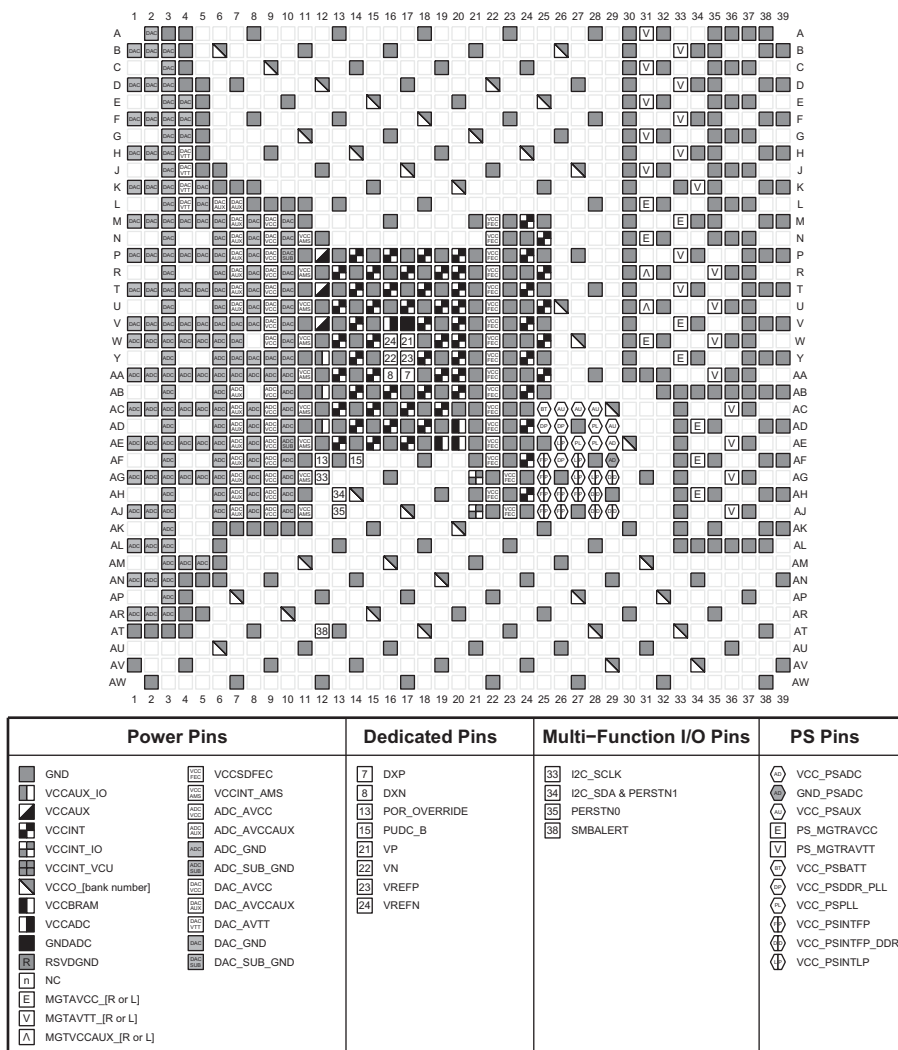
Figure 4-54: FFGV1517 and FSVG1517 Packages—XCZU27DR and XCZU28DR Power, Dedicated, and Multi-function Pin Diagram
