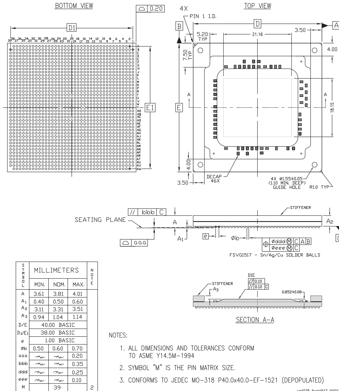
Figure 5-23: Package Dimensions for FSVG1517 (XCZU25DR, XCZU27DR, XCZU28DR, XCZU43DR, XCZU47DR, XCZU48DR)
