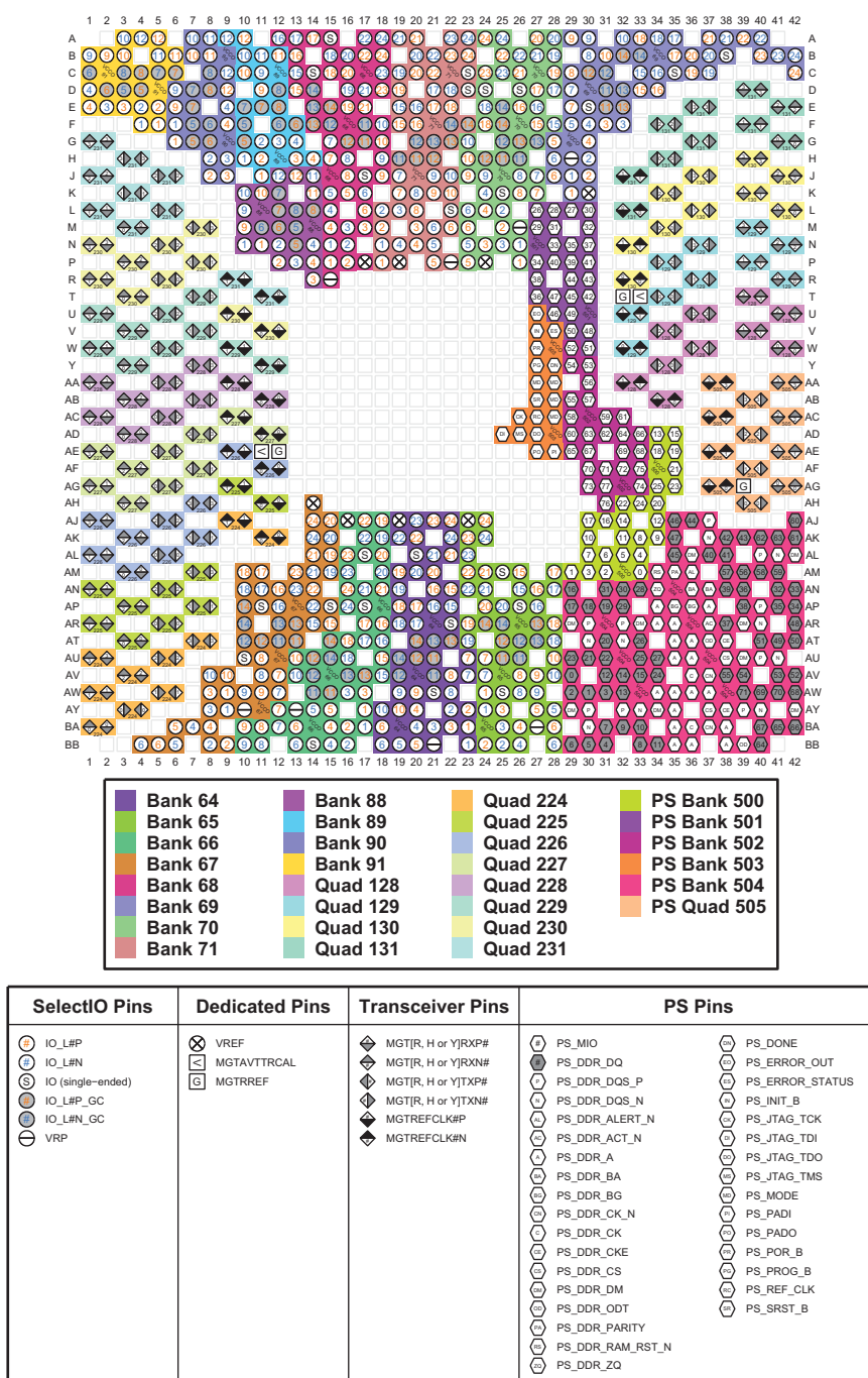
Figure 4-61: FFVC1760 Package—XCZU11EG I/O Bank Diagram
