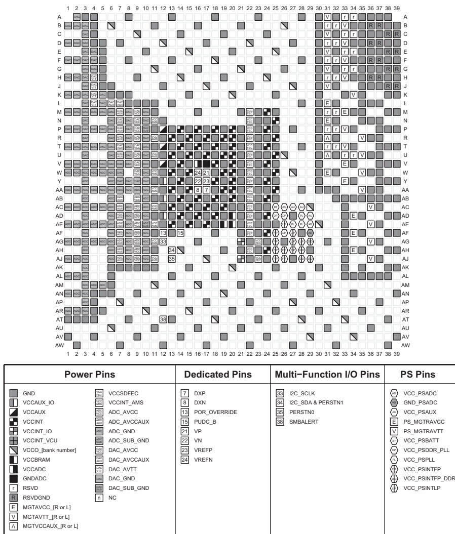
Figure 4-52: FFVG1517 and FSVG1517 Packages—XCZU25DR Power, Dedicated, and Multi-function Pin Diagram
