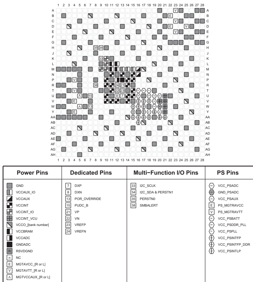
Figure 4-10: SFVC784 Package—XCZU4EV, XCZU5EV, XAZU4EV, and XAZU5EV Power, Dedicated, and Multi-function Pin Diagram
