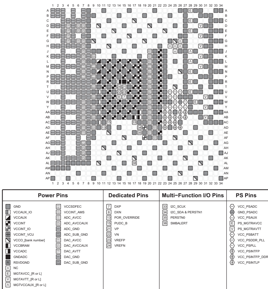
Figure 4-34: FFEV1156 and FSVE1156 Packages—XCZU27DR and XCZU28DR Power, Dedicated, and Multi-function Pin Diagram
