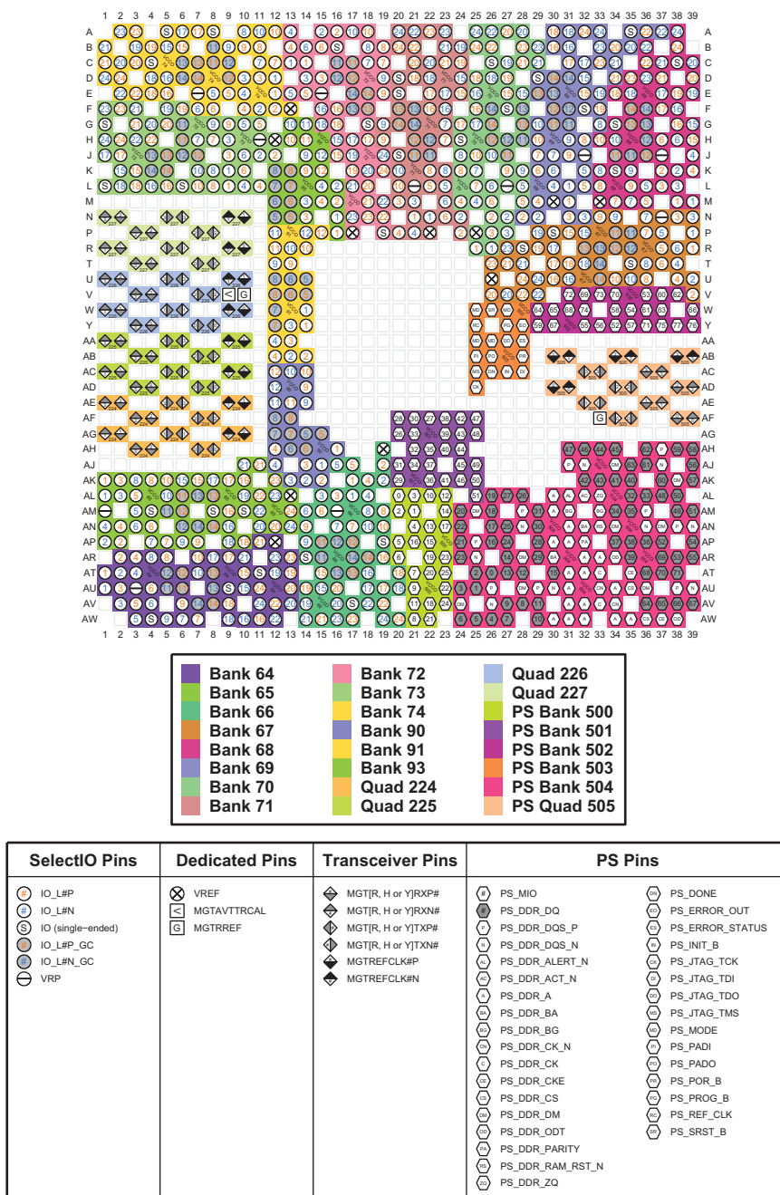
Figure 4-43: FFVB1517 Package—XCZU17EG and XCZU19EG I/O Bank Diagram
