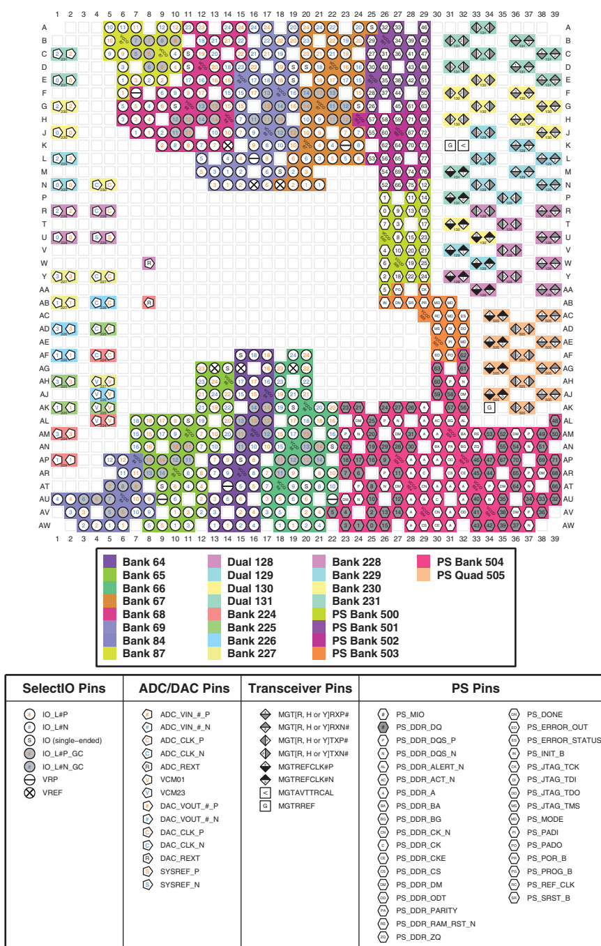
Figure 4-57: FFVG1517 and FSVG1517 Packages—XCZU47DR I/O Bank Diagram
