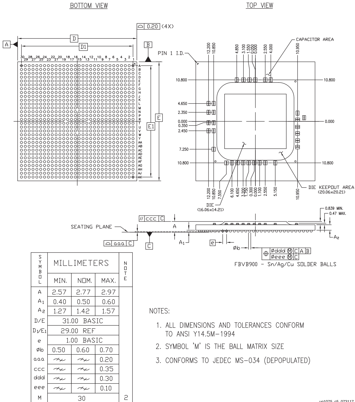
Figure 5-7: Package Dimensions for FBVB900 (XCZU7CG, XCZU7EG, XCZU7EV, and XAZU7EV)
