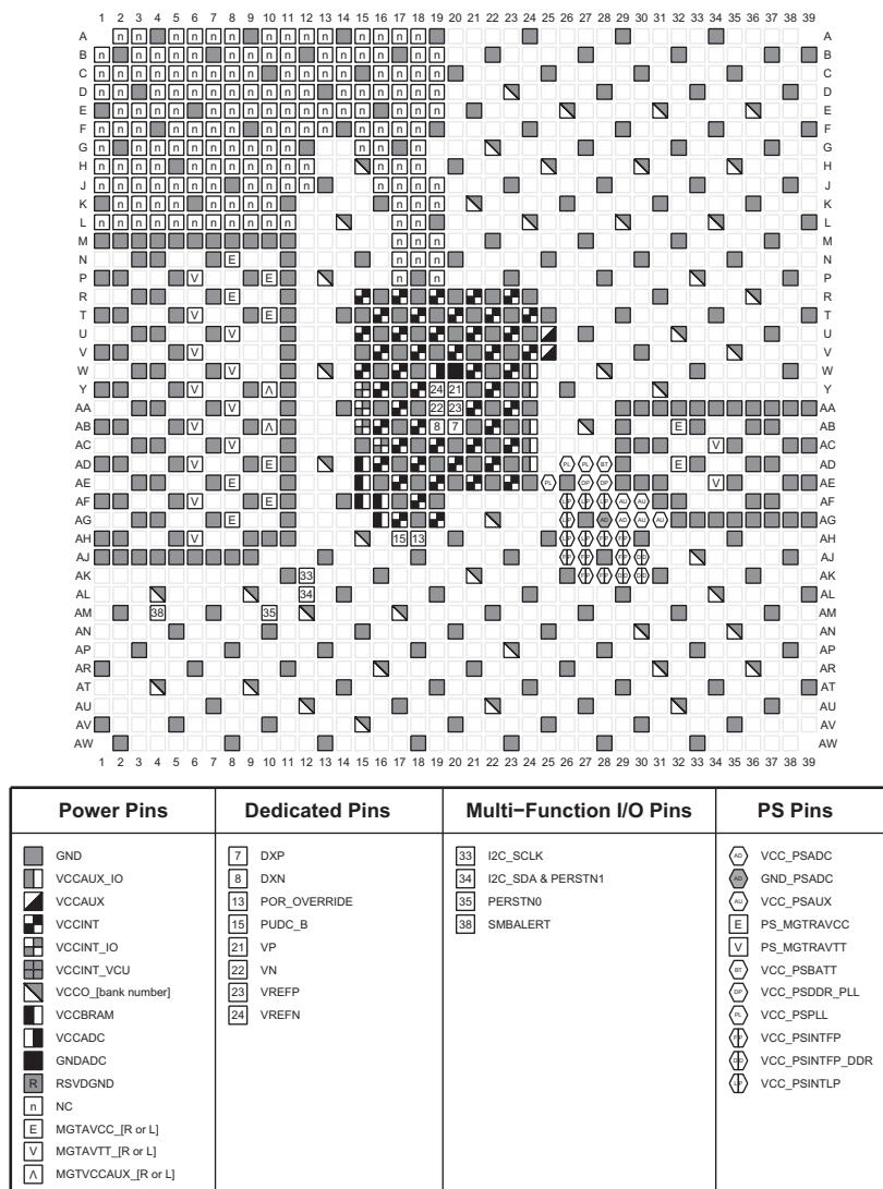
Figure 4-42: FFVB1517 Package—XCZU11EG Power, Dedicated, and Multi-function Pin Diagram
