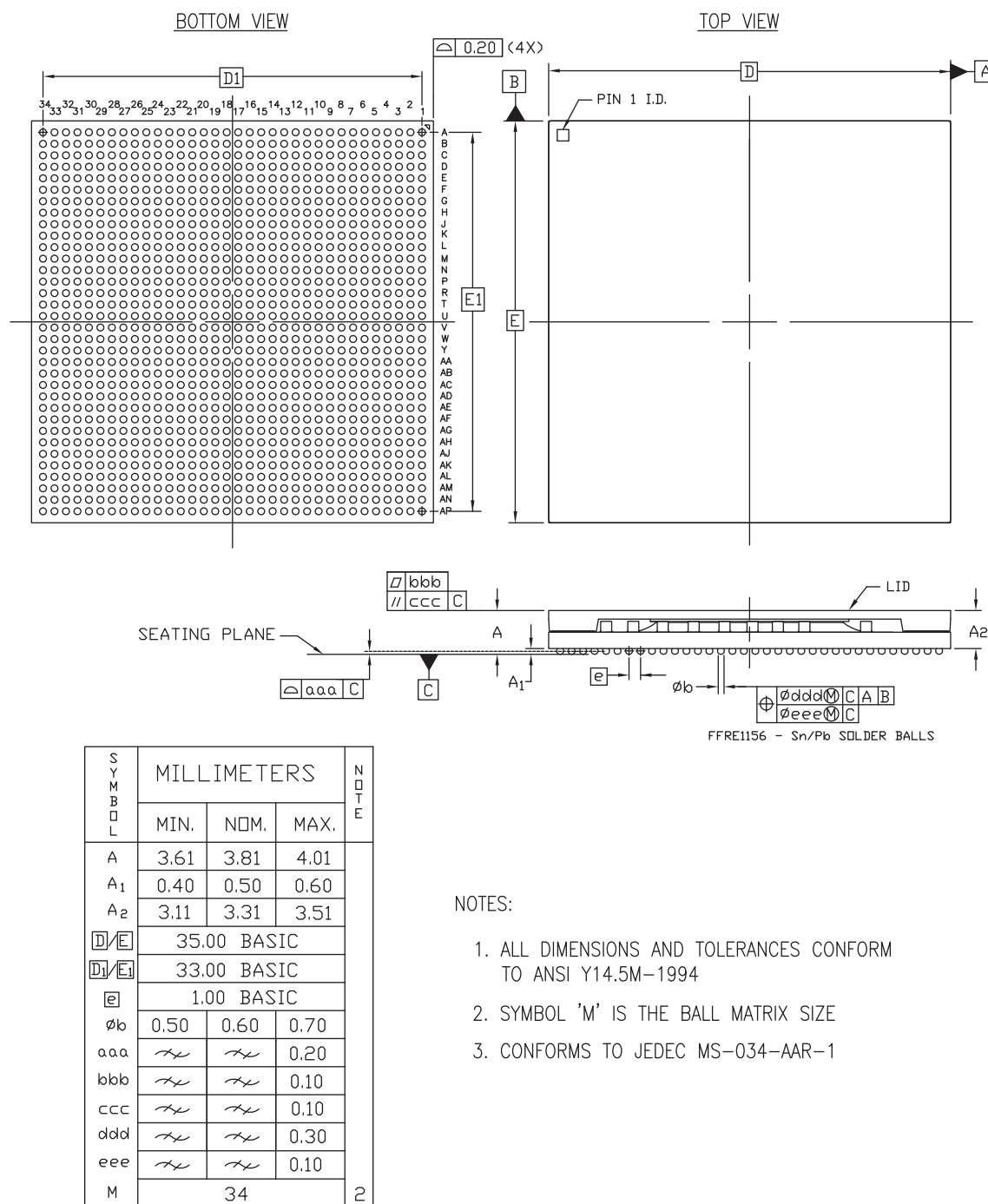
Figure 5-16: Package Dimensions for FFRE1156 (XQZU28DR)
