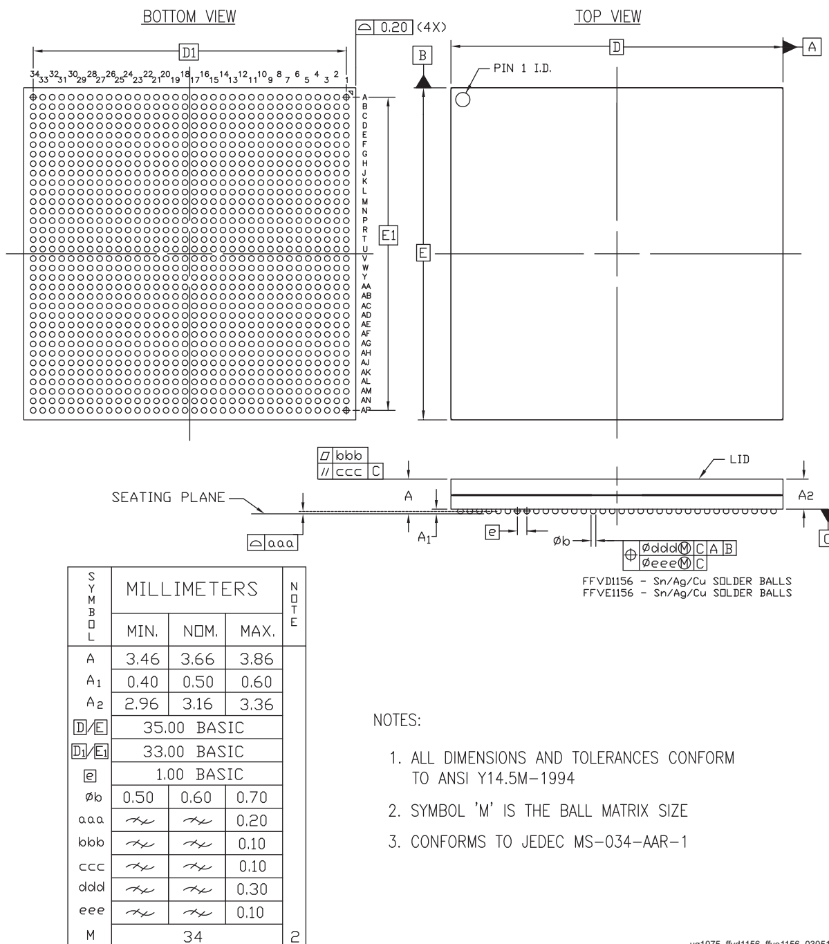
Figure 5-17: Package Dimensions for FFVD1156 (XCZU21DR) and FFVE1156 (XCZU25DR, XCZU27DR, XCZU28DR, XCZU43DR, XCZU47DR, XCZU48DR)
