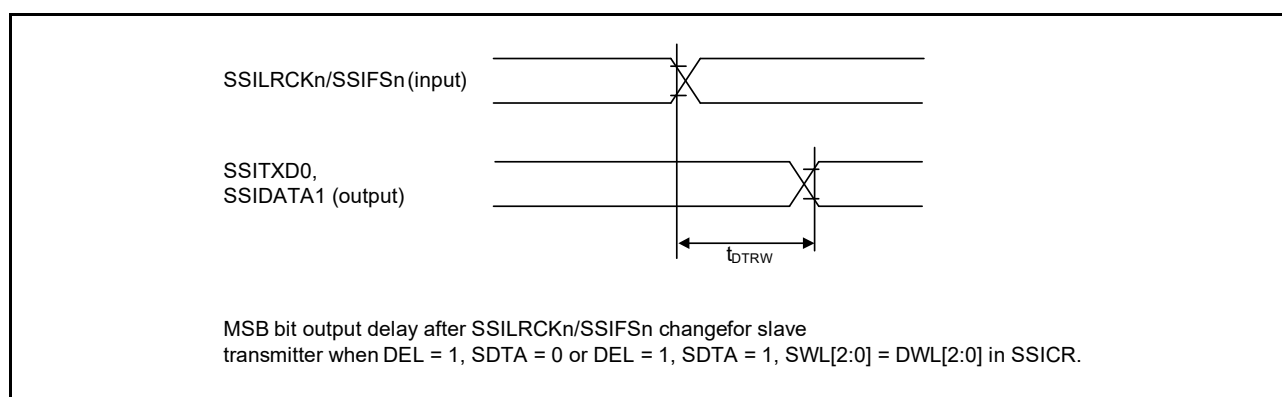
Figure 2.65 SSIE data output delay after SSILRCKn/SSIFSs change
