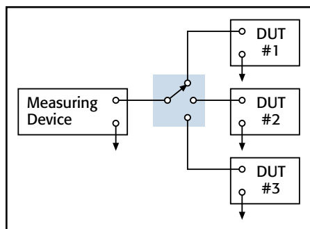
Figure 5. Scanner Switch
