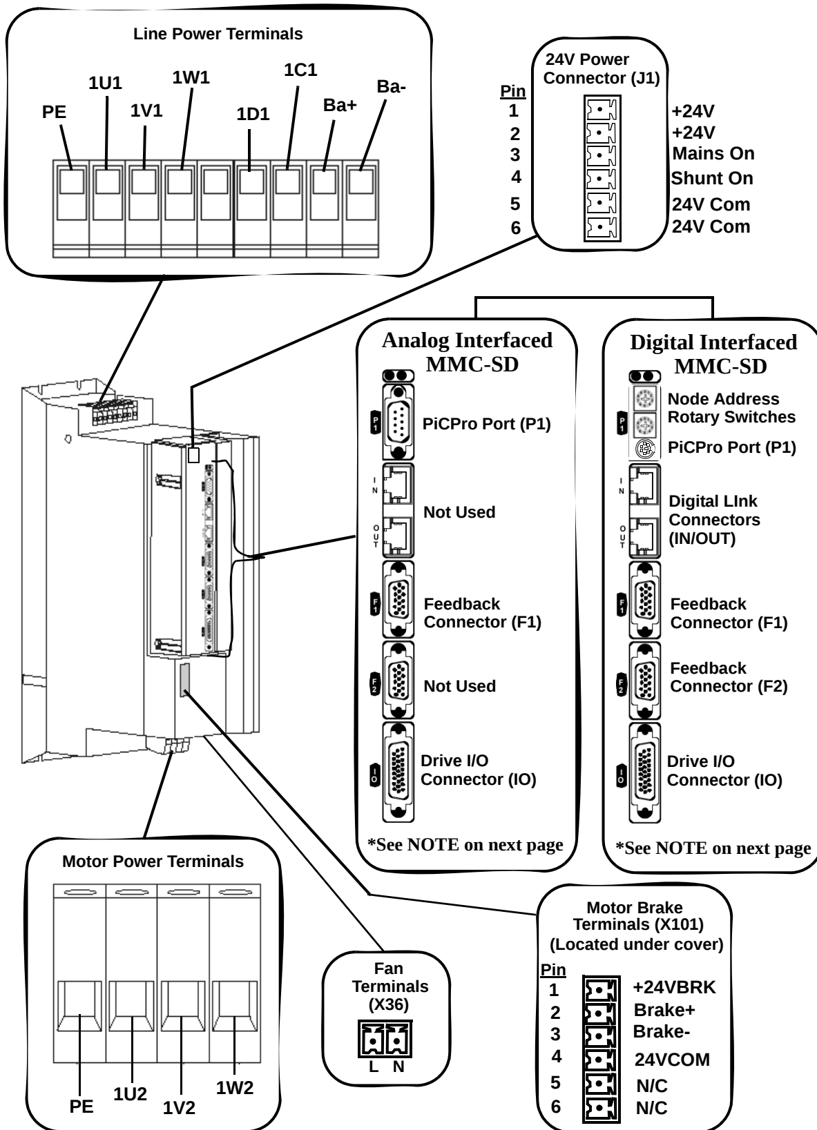
Figure 6-8: Connectors on the Size 4 460V Drive
