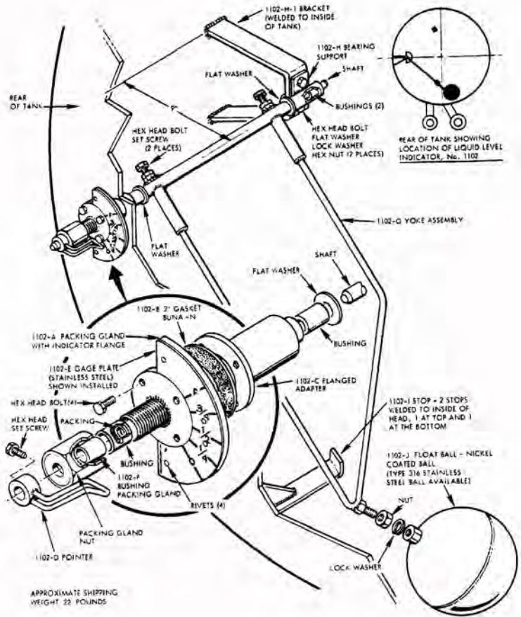
1102 Level Indicator
