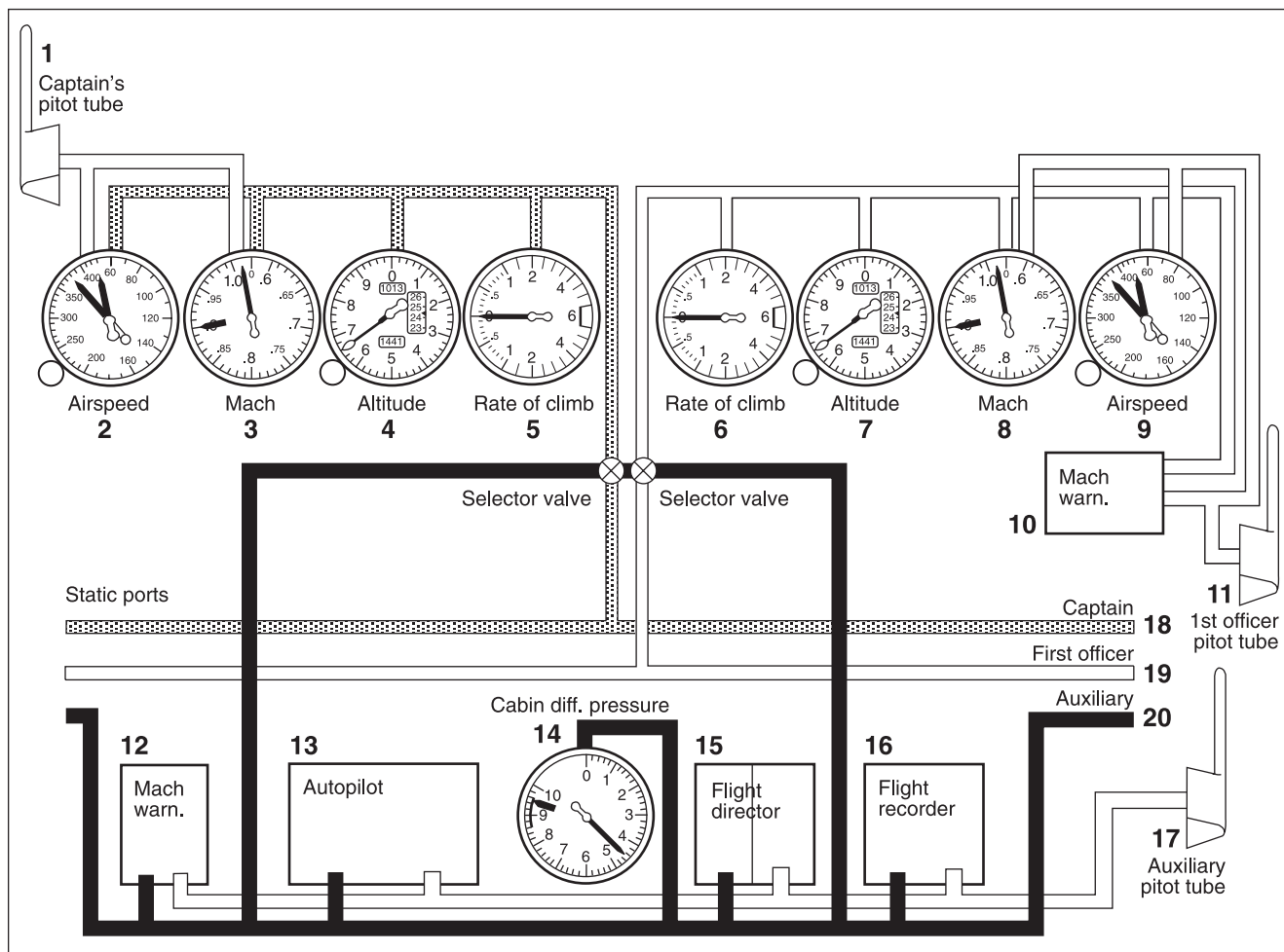
Figure 2-1. Typical pitot-static system
