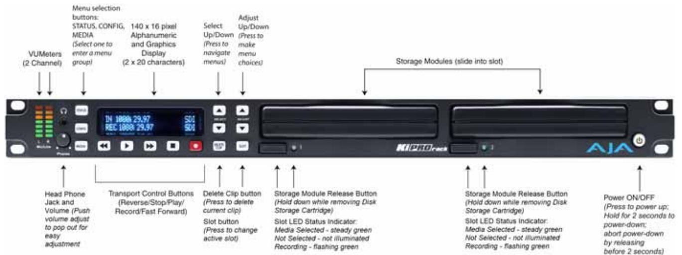
Figure 1. Ki Pro Operator Side (front panel)
