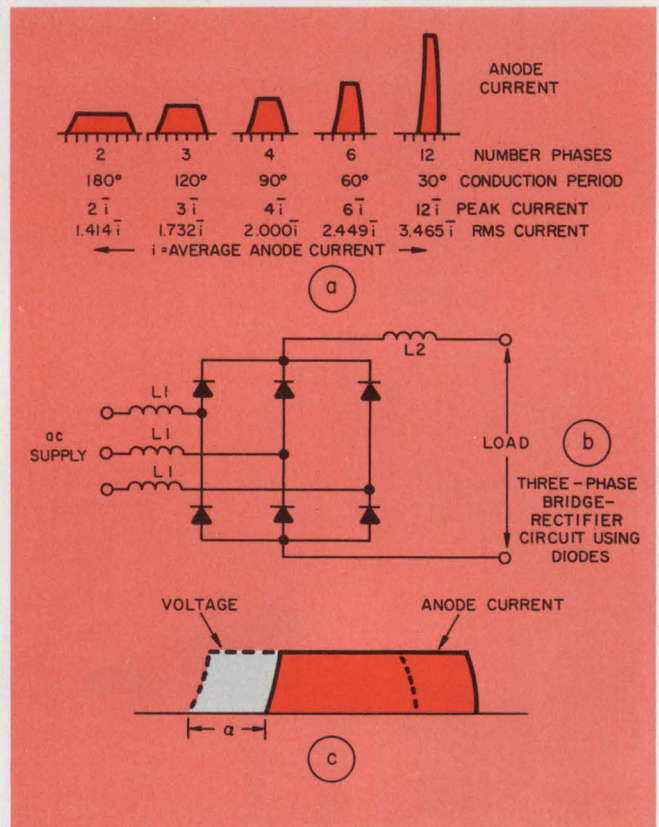
1. Essentially rectangular anode-current waveforms (a) result from rectifier circuits having inductance in the ac supply and load line (b). Replacing the diodes in the circuit with SCRs only causes a shift in the anode current waveform by an amount determined by \alpha , the phase retard angle (c).
