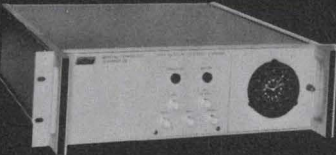
MODEL 304-D RUBIDIUM FREQUENCY STANDARD For general lab and field use. Almost entirely unaffected by environmental factors. Provides stable, accurate source of standard frequencies. Integral time scale selector.
