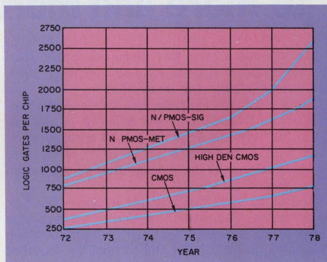
The number of gates per chip is expected to grow as chips get bigger. By 1975 complexity will reach 1200 to 1400 gates.
