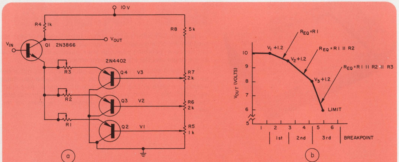
The relation between output and input voltages is a series of straight-line segments. As the input voltage increases, each of transistors Q_2 through Q_4 successively conducts and causes the
