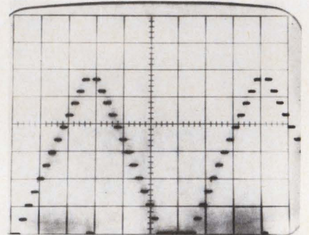
Pseudo-sinusoidal waveform generated by operating a programmable switching chain as a staircase generator. Voltage is switched down as well as up.
