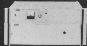
MODEL 6500 VISUAL CARRIER GENERATOR Reduces co-channel interference. Increases TV coverage area. Gives precise frequency separation. Uses the Rubidium Frequency Standard which easily controls the transmitted frequency with the required accuracy. Extremely stable, demonstrated reliability.
