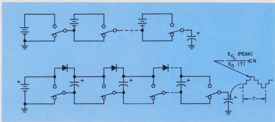
A switched chain of energy storage elements, such as batteries or capacitors, can generate high voltages or a variable high-voltage waveform. The peak voltage output is directly proportional to the number of switched steps.
