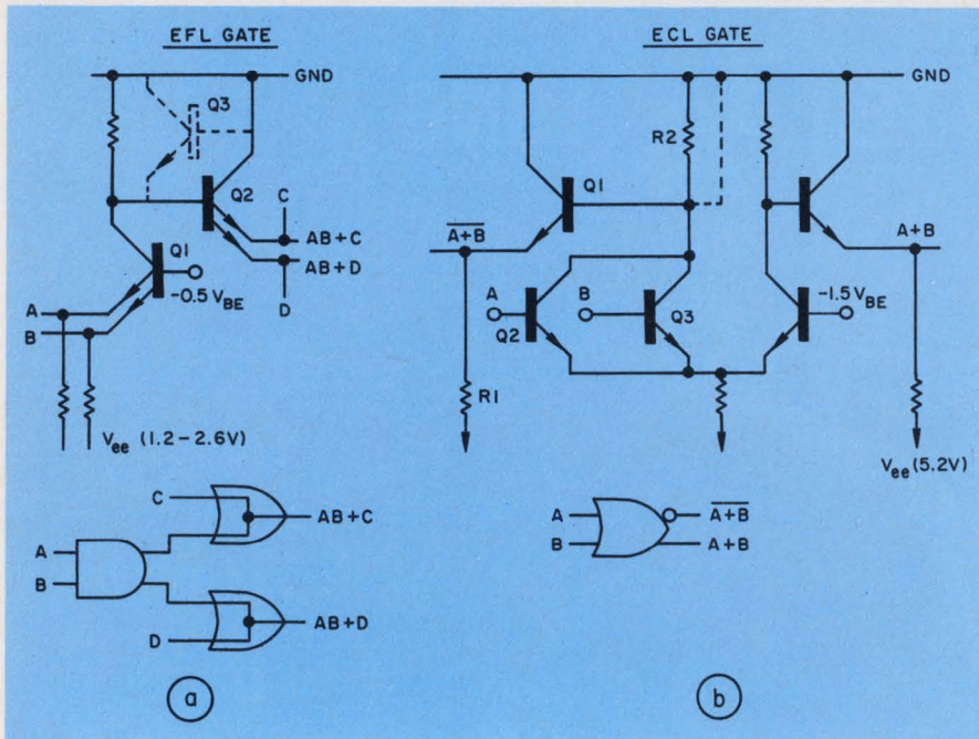
Emitter function logic minimizes the need for inverters. This results in simpler logic design as can be seen above.
