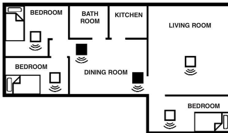
Figure 3: Single storey dwelling with separate sleeping areas
