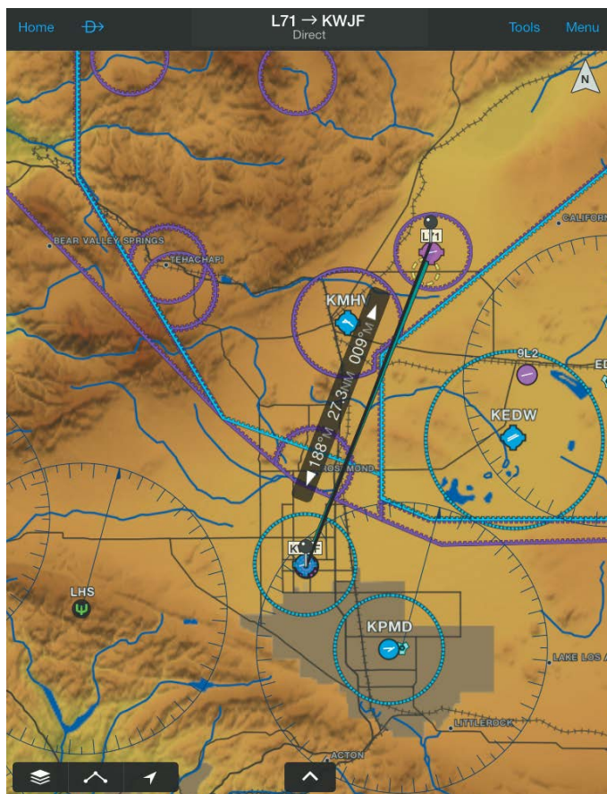
Distance Tool
