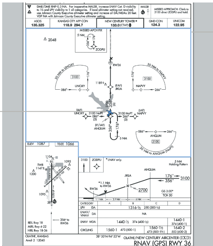
Geo-Referenced FliteCharts
