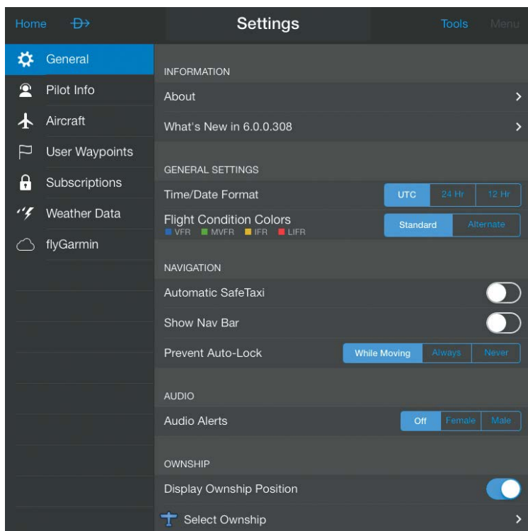
Settings Page
