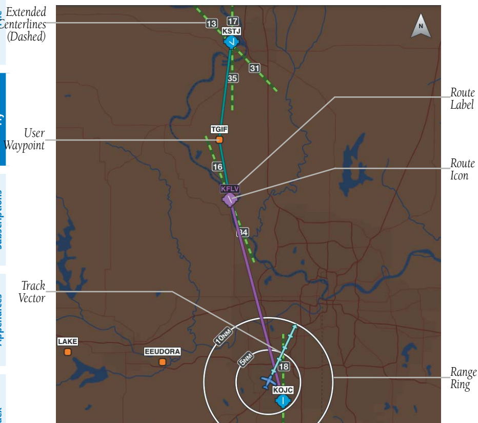
Ownship/Route Settings
