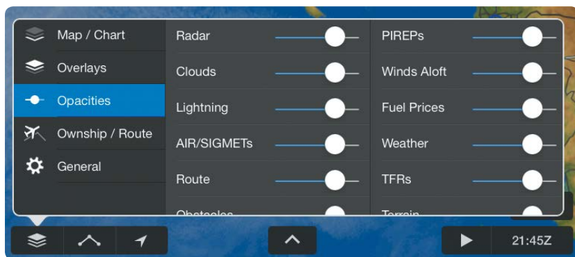
Opacities Menu
