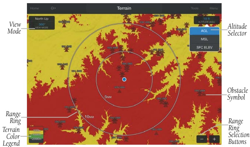
Terrain Page
