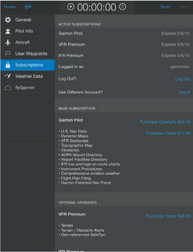
Subscriptions
