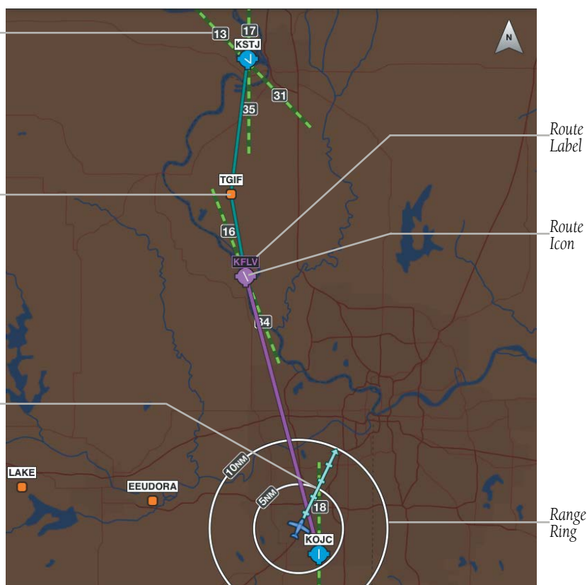
Ownship/Route Settings
