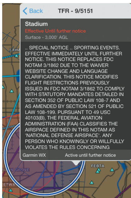
TFR Overlay
