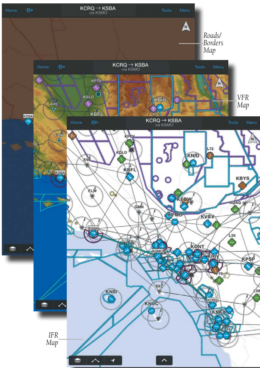
Map Themes
