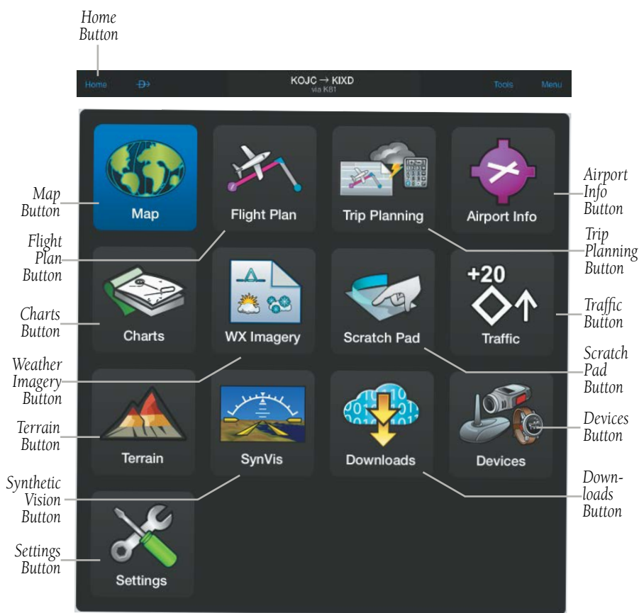
Home Menu
