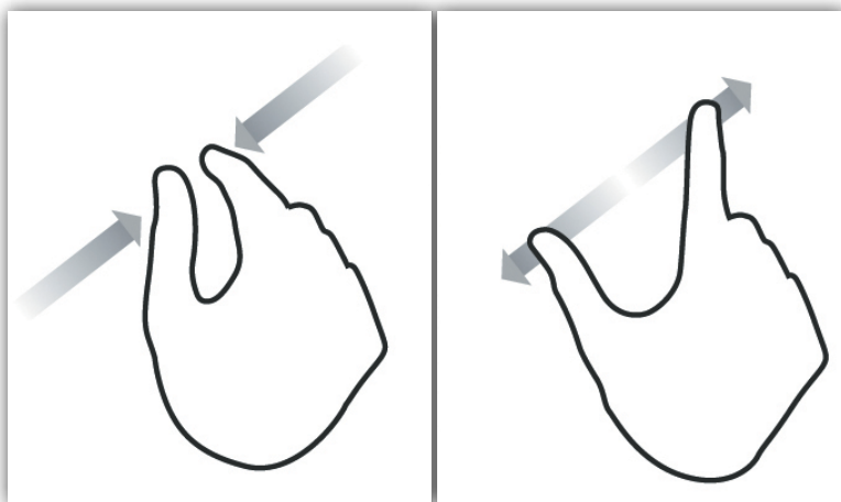
Pinch Zoom
