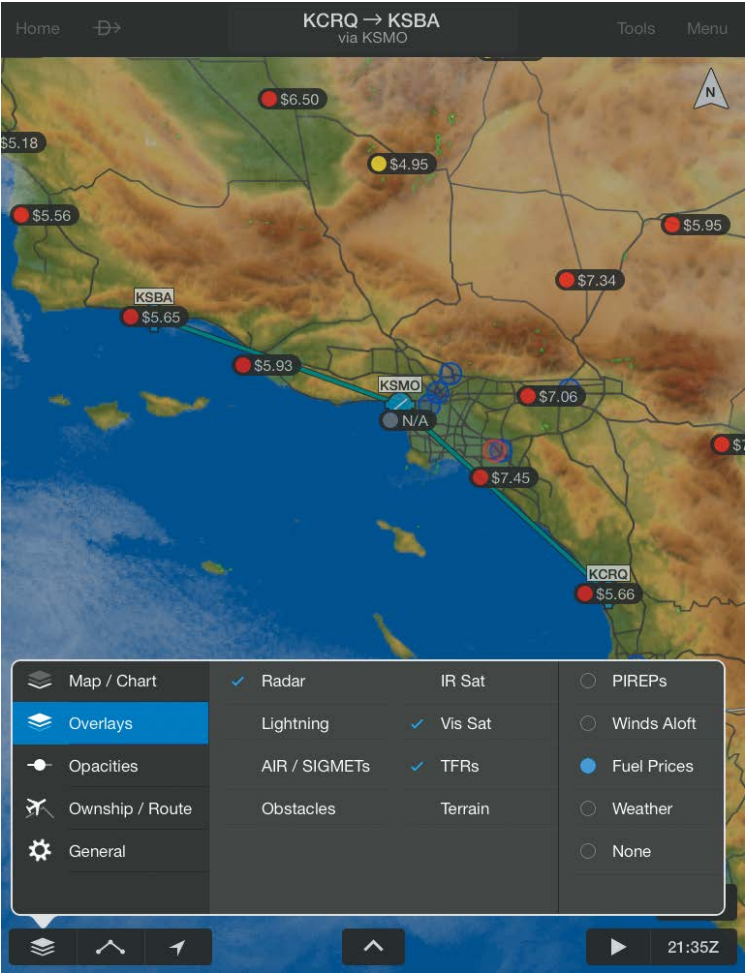
Map Overlays
