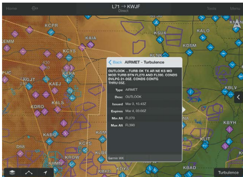
AIRMET/SIGMET Overlay
