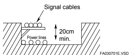
Figure A3.32 Segregation Using Cable Rack
