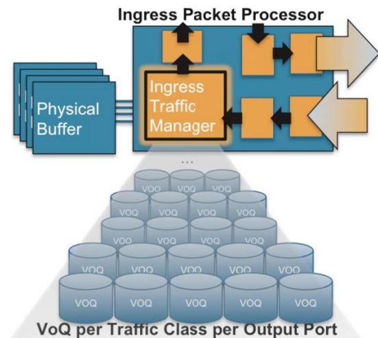
Figure 21: Physical Buffer on Ingress allocated as Virtual Output Queues
