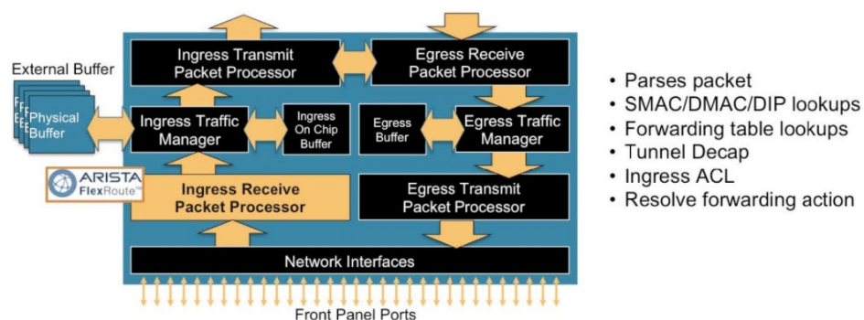
Figure 17: Packet Processor stage 2 (ingress): Ingress Receive Packet Processor
