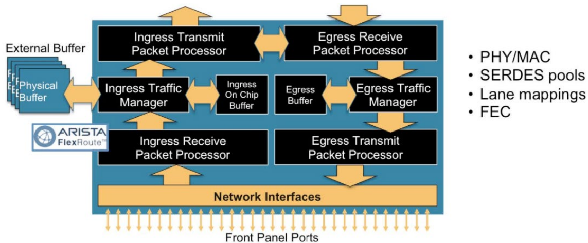
Figure 16: Packet Processor stage 1 (ingress): Network Interface
