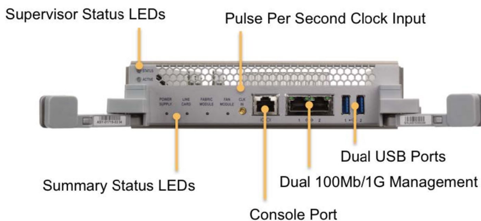
Figure 2: Arista 7500 Series Supervisor 2 Module.
