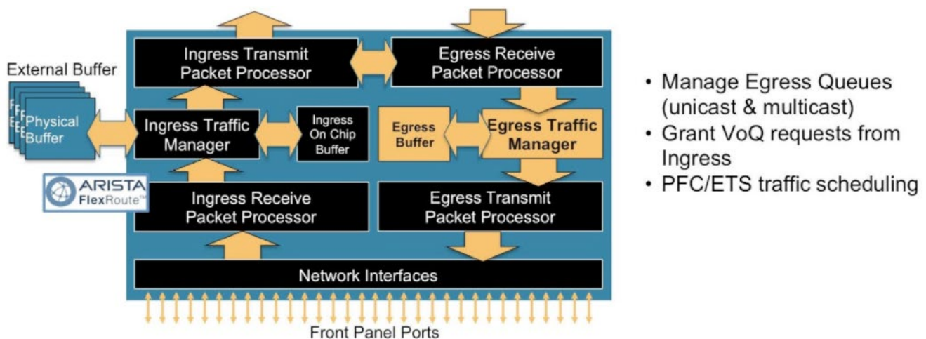
Figure 27: Packet Processor stage 7 (egress): Egress Traffic Manager
