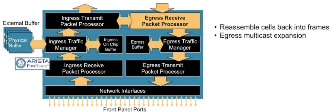
Figure 26: Packet Processor stage 6 (egress): Egress Receive Packet Processor
