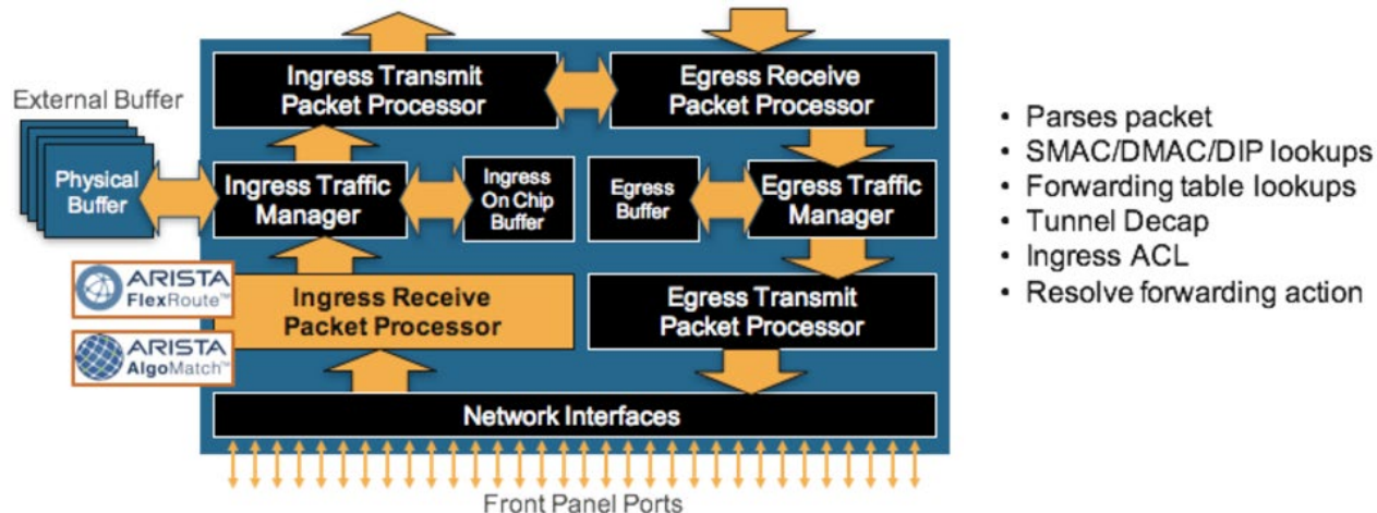
Figure 18: Packet Processor stage 2 (ingress): Ingress Receive Packet Processor with AlgoMatch
