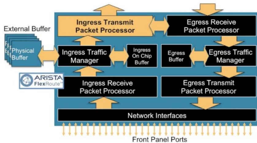
Figure 22: Packet Processor stage 4 (ingress): Ingress Transmit Packet Processor
