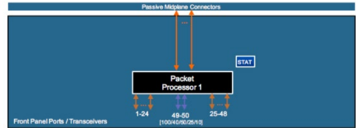
Figure 14: Arista DCS-7500R2AK-48YCQ-LC (36 x 10G, 12 x 25G and 2 x100G)
