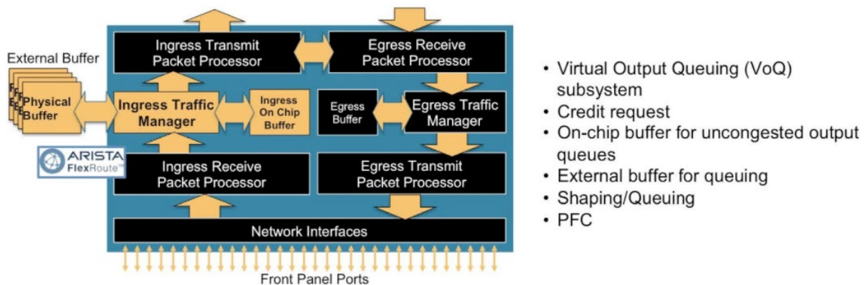
Figure 20: Packet Processor stage 3 (ingress): Ingress Traffic Manager
