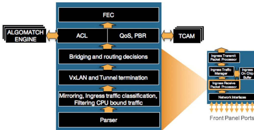
Figure 19: Ingress Receive Packet Processor with AlgoMatch
