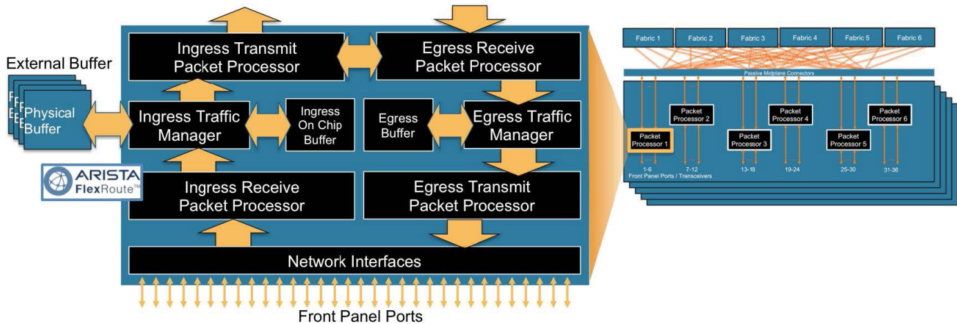
Figure 15: Packet forwarding pipeline stages inside a packet processor on an Arista 7500R line card module
