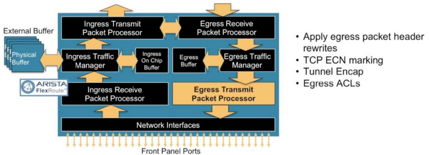
Figure 26: Packet processor stage 8 (egress): Egress Transmit Packet Processor
