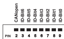
Figure 3.29. J1 – Axis ID pins
