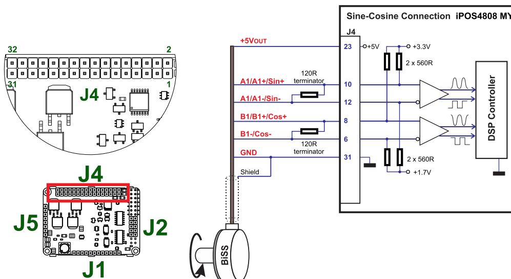
Figure 3.18. Sine-Cosine analogue encoder connection
