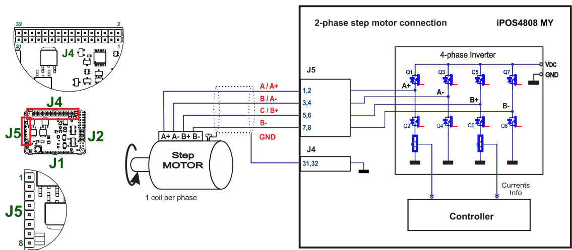
Figure 3.11. 2-phase step motor connection, one coil per phase
