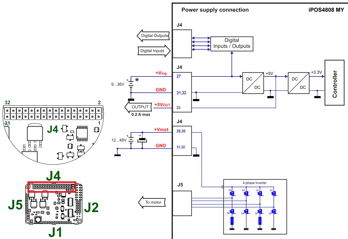
Figure 3.24. Supply connection
