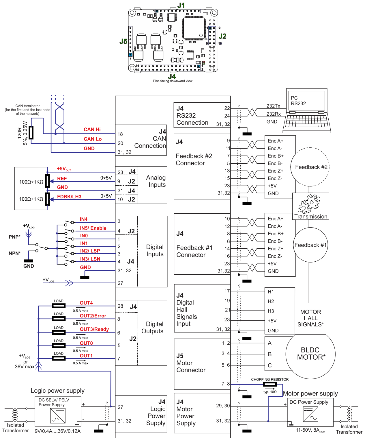
Figure 3.3. iPOS4808 MY-CAN Connection diagram
