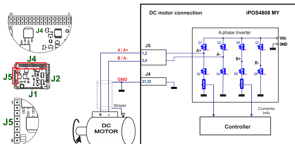
Figure 3.14. DC Motor connection
