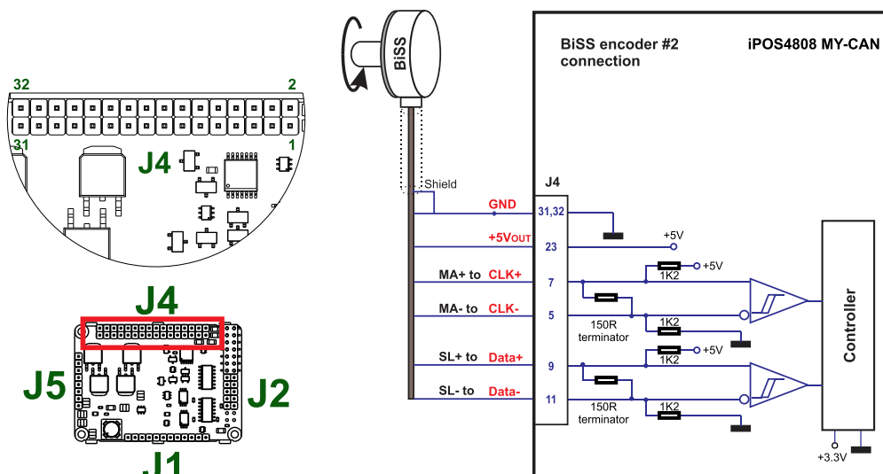
Figure 3.20. BiSS-C encoder #2 connection
