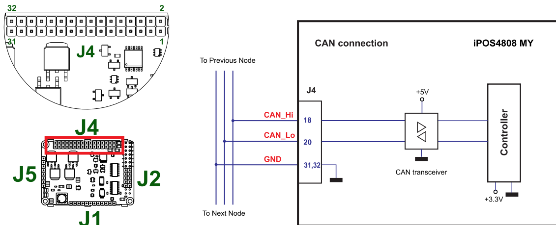
Figure 3.26. CAN connection
