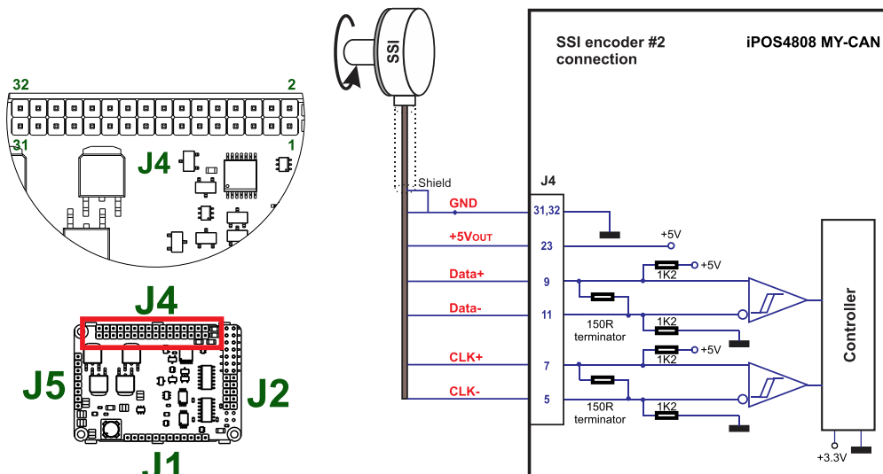
Figure 3.19. SSI encoder #2 connection
