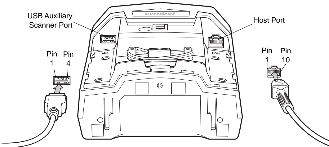
Figure 4-1 Cable Pinouts
