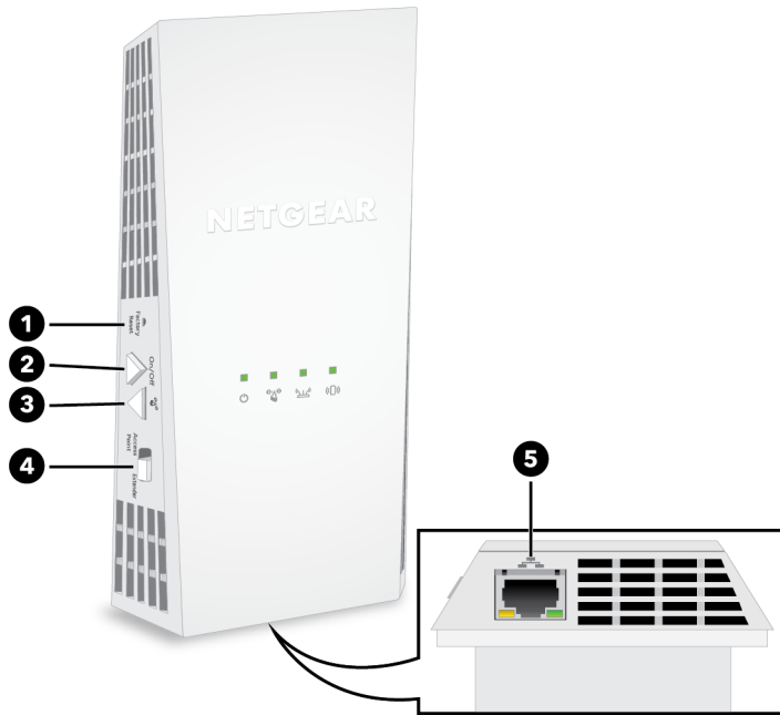
Figure 2. Side and bottom panel
