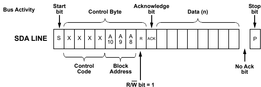
Figure 230: Current Address Read Command, \overline{R/W} = 1
