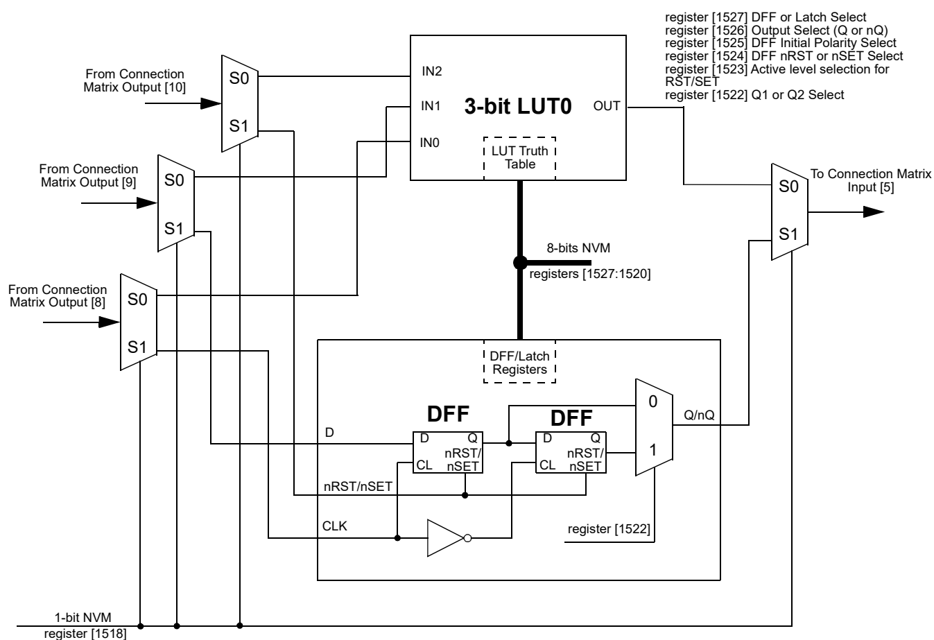
Figure 19: 3-bit LUT0 or DFF3
