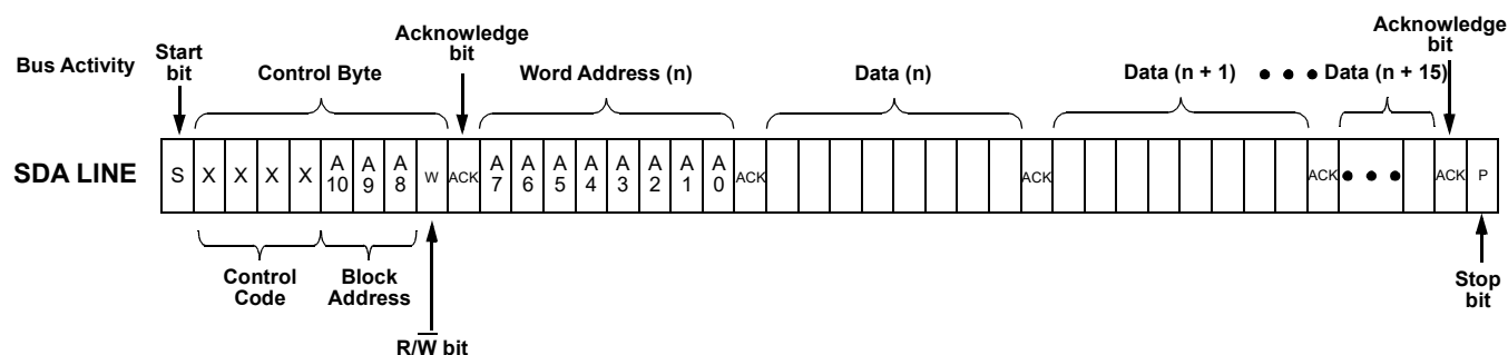
Figure 235: Page Write Command
