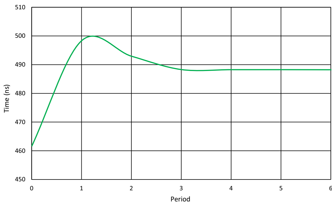
Figure 214: Oscillator1 Settling Time, V_{DD} = 3.3\text{ V} , T = 25\text{ }^{\circ}\text{C} , \text{OSC1} = 2\text{ MHz}
