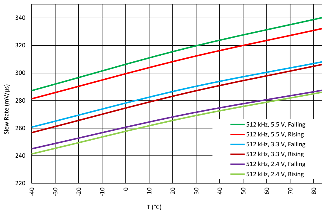
Figure 105: Slew Rate vs. Ambient Temperature G = 1 \text{ V/V} ; R_L = 50 \text{ k}\Omega for BW = 512 \text{ kHz}
