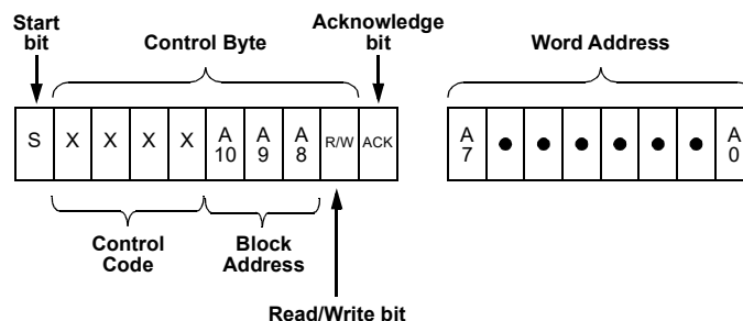
Figure 226: Basic Command Structure
