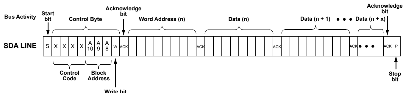
Figure 229: Sequential Write Command
