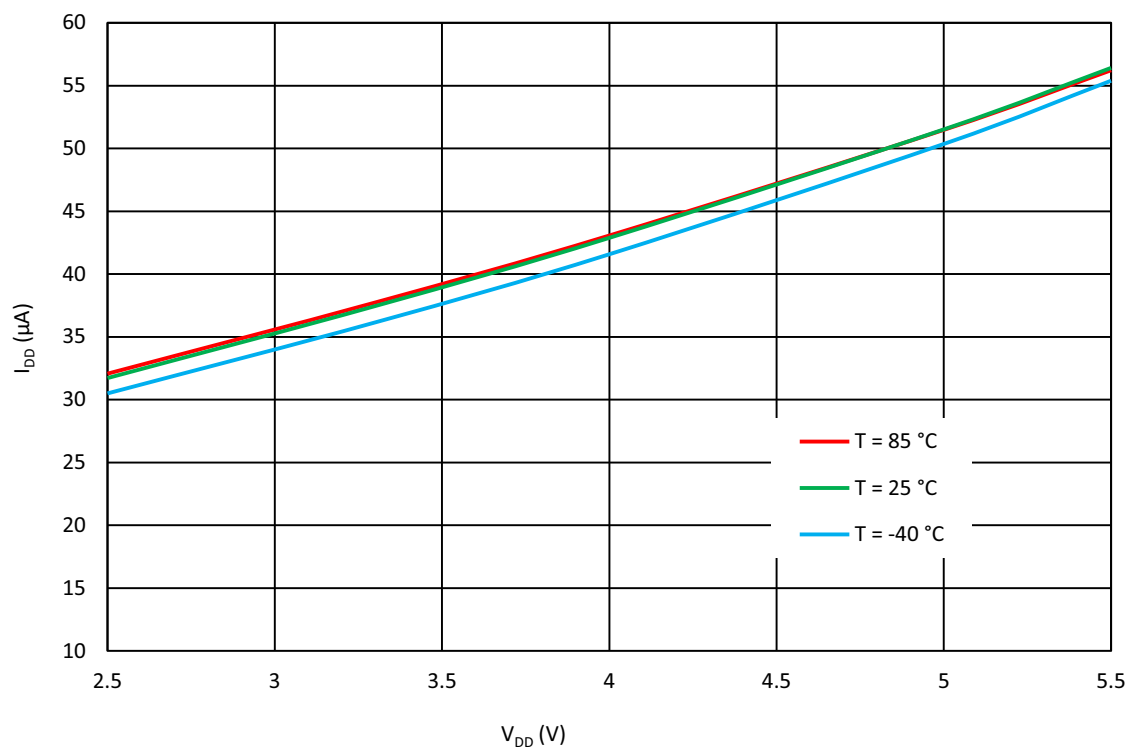
Figure 221: OSC2 Current Consumption vs. V_{DD} (Pre-Divider = 4)
