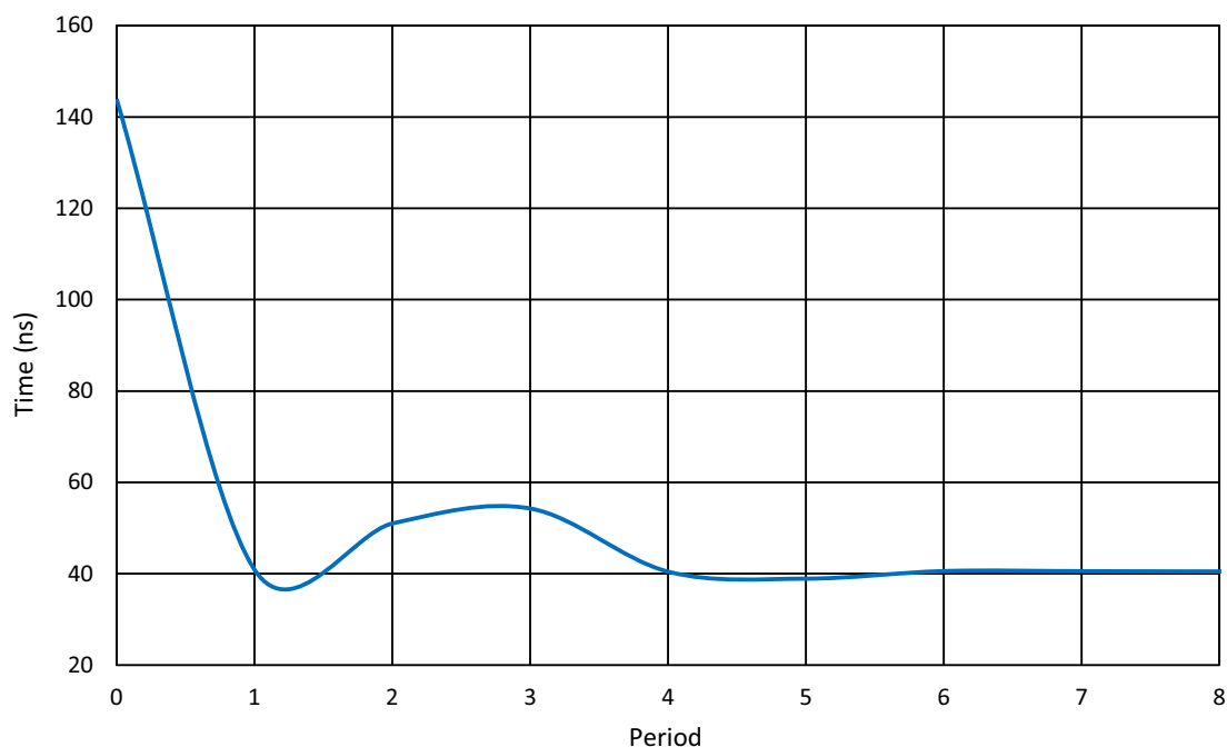
Figure 216: Oscillator2 Settling Time, V_{DD} = 3.3\text{ V} , T = 25\text{ }^{\circ}\text{C} , OSC2 = 25 MHz (Start with Delay)
