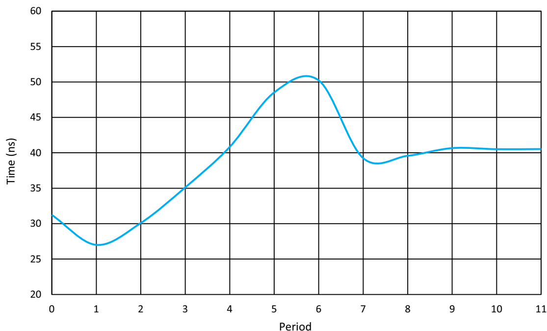
Figure 215: Oscillator2 Settling Time, V_{DD} = 3.3\text{ V} , T = 25\text{ }^{\circ}\text{C} , OSC2 = 25 MHz (Normal Start)
