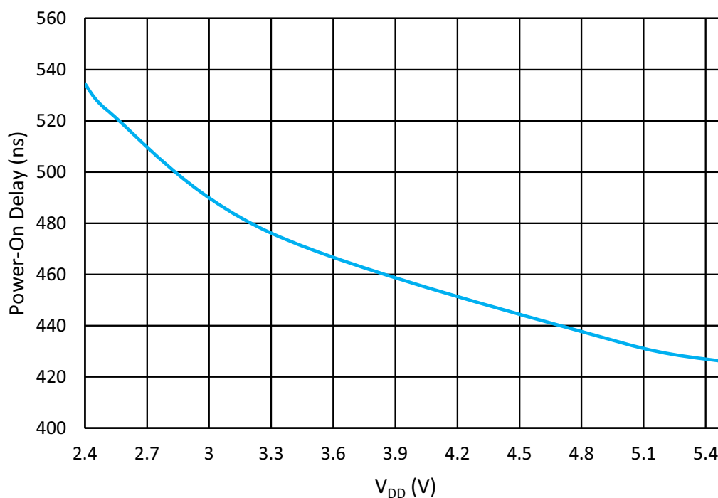
Figure 207: OSC1 Oscillator Maximum Power-On Delay vs. V_{DD} at T = 25^{\circ}\text{C} , OSC1 = 2.048 MHz
