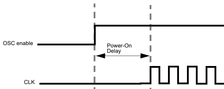
Figure 205: Oscillator Startup Diagram
