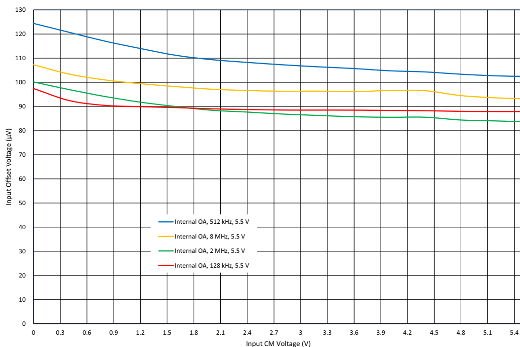
Figure 84: Internal OpAmp Input Offset Voltage vs. Input CM Voltage at T = 25\text{ }^{\circ}\text{C} , V_{\text{DDA}} = 5.5\text{ V}
