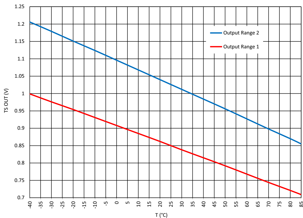
Figure 238: TS Output vs. Temperature, V_{DD} = 3.3\text{ V}
