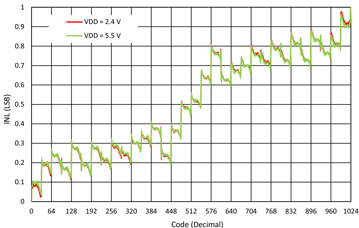
Figure 184: INL vs. Digital Code, Potentiometer Mode ( V_{AB} = 1 V) at T = 25 °C
