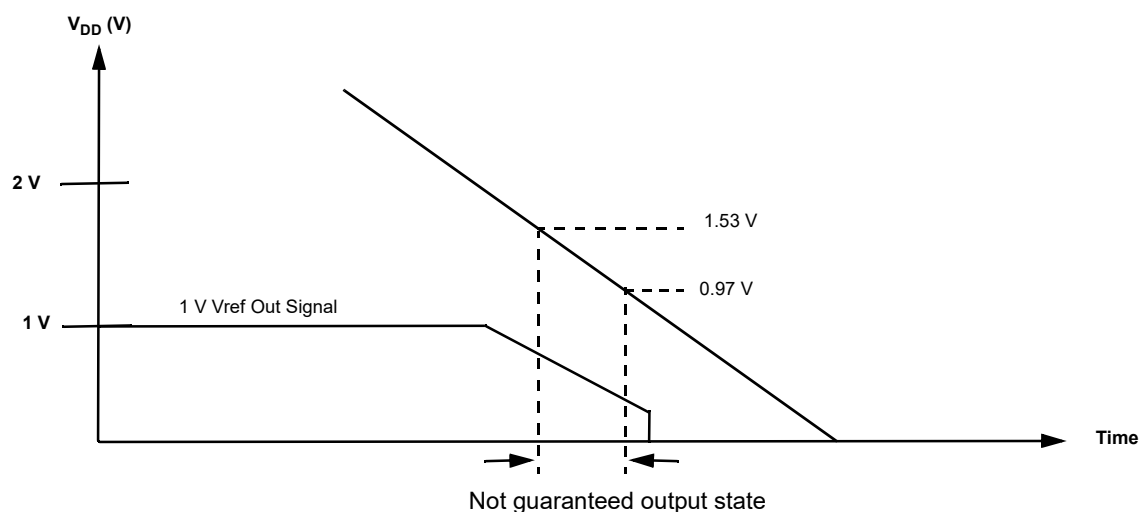
Figure 225: Power-Down
