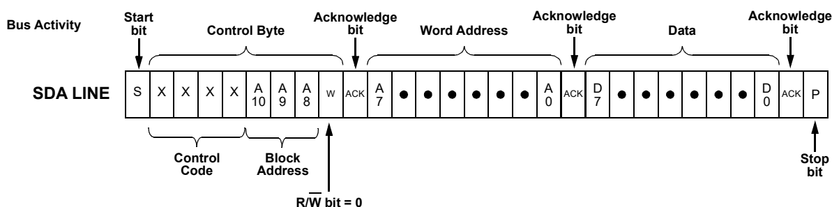
Figure 228: Byte Write Command, \overline{R/W} = 0
