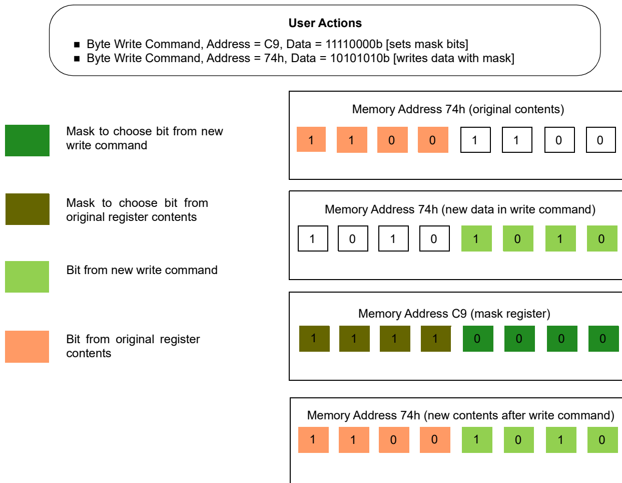
Figure 234: Example of I 2 C Byte Write Bit Masking
