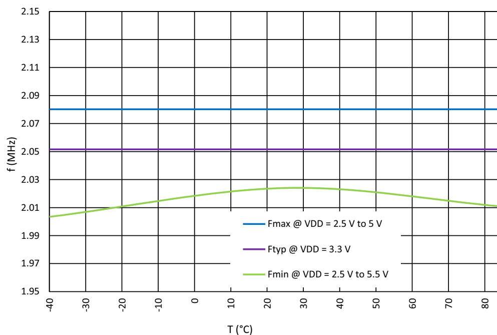
Figure 210: OSC1 Frequency vs. Temperature, OSC1 = 2.048 MHz
