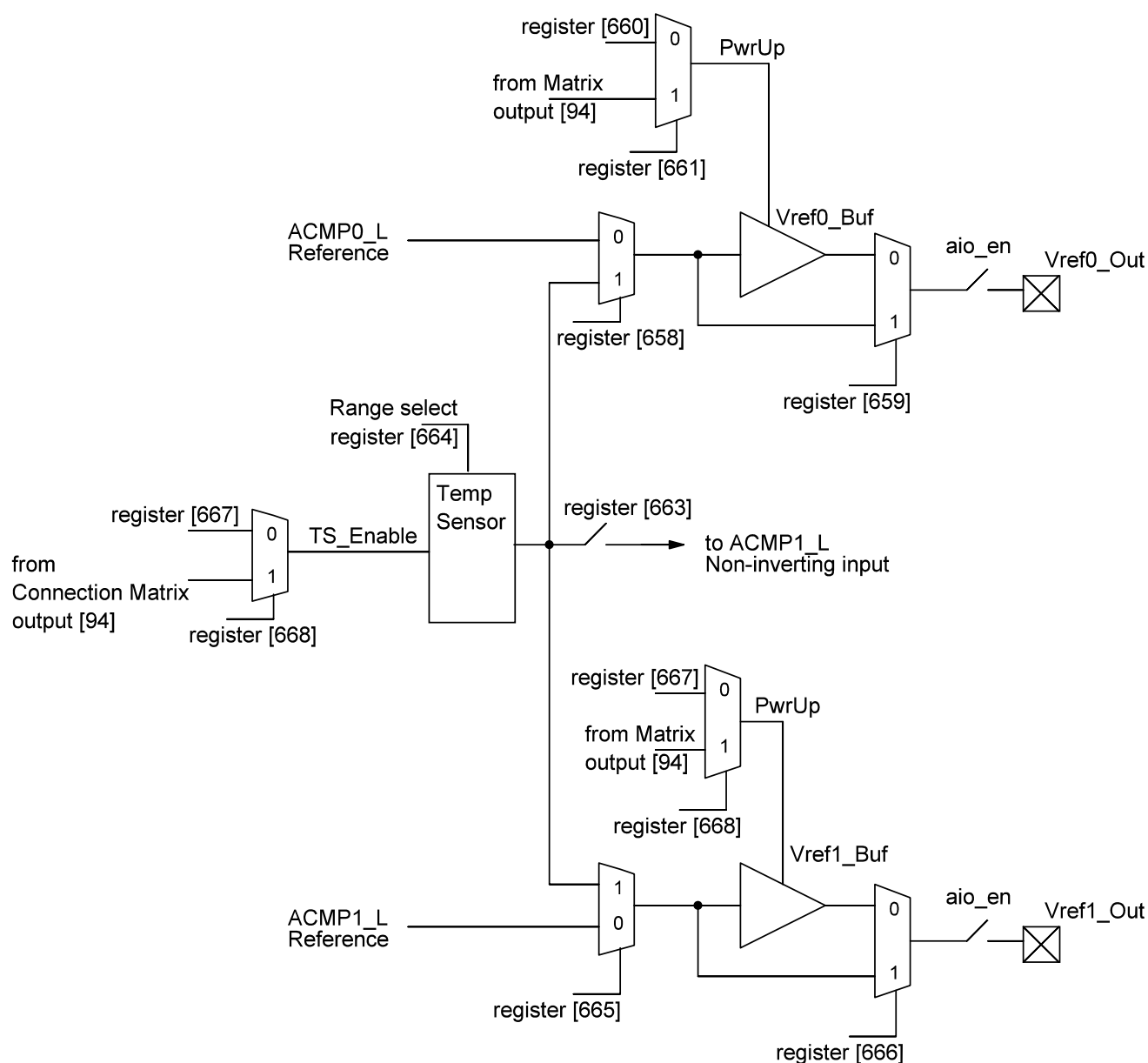
Figure 237: Analog Temperature Sensor Structure Diagram
