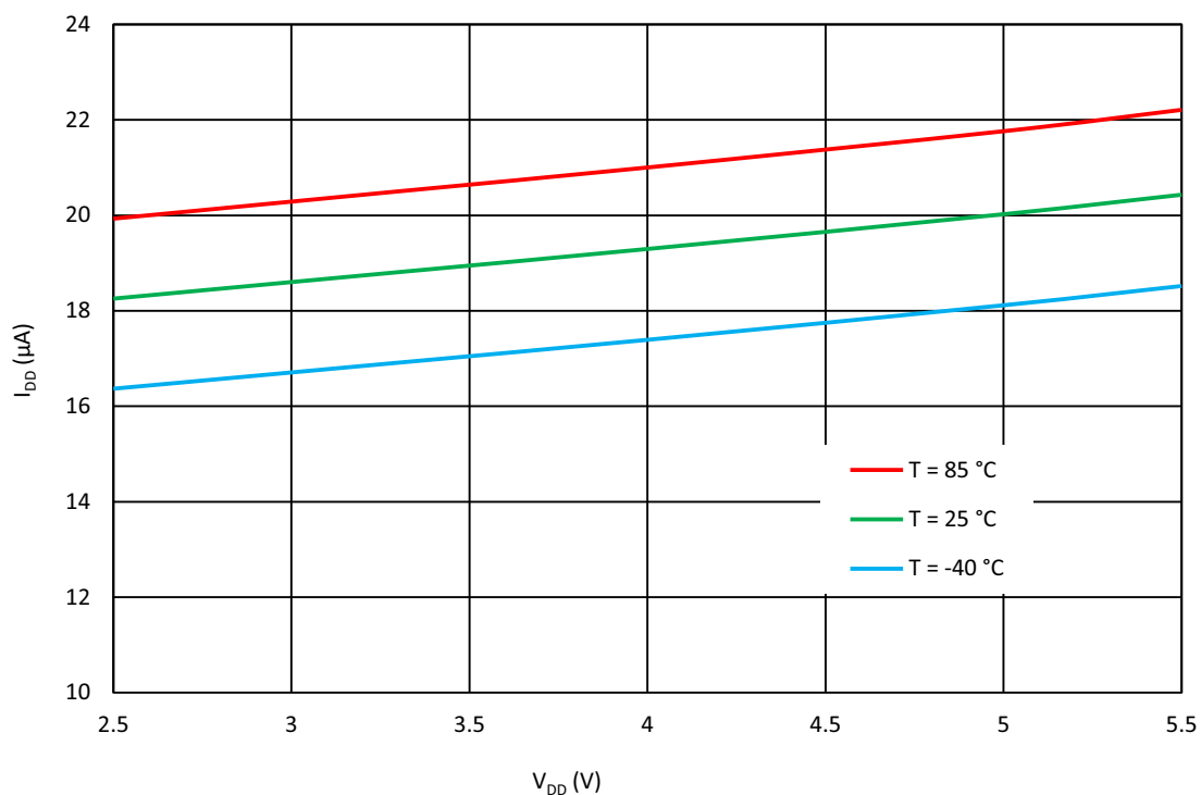
Figure 218: OSC1 Current Consumption vs. V DD (Pre-Divider = 4)
