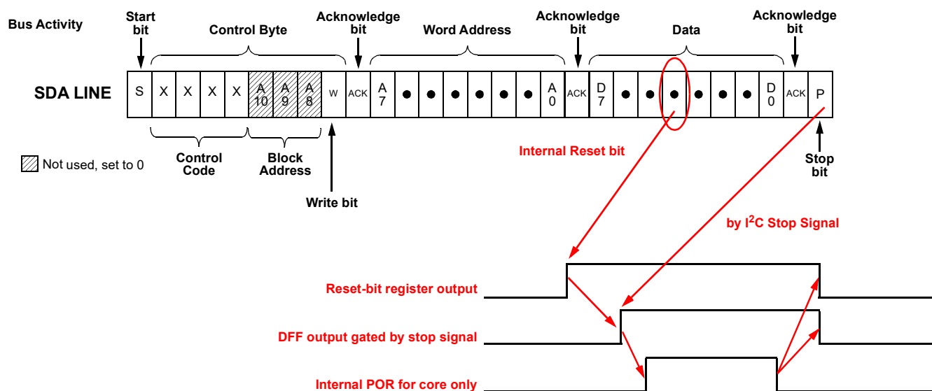
Figure 233: Reset Command Timing
