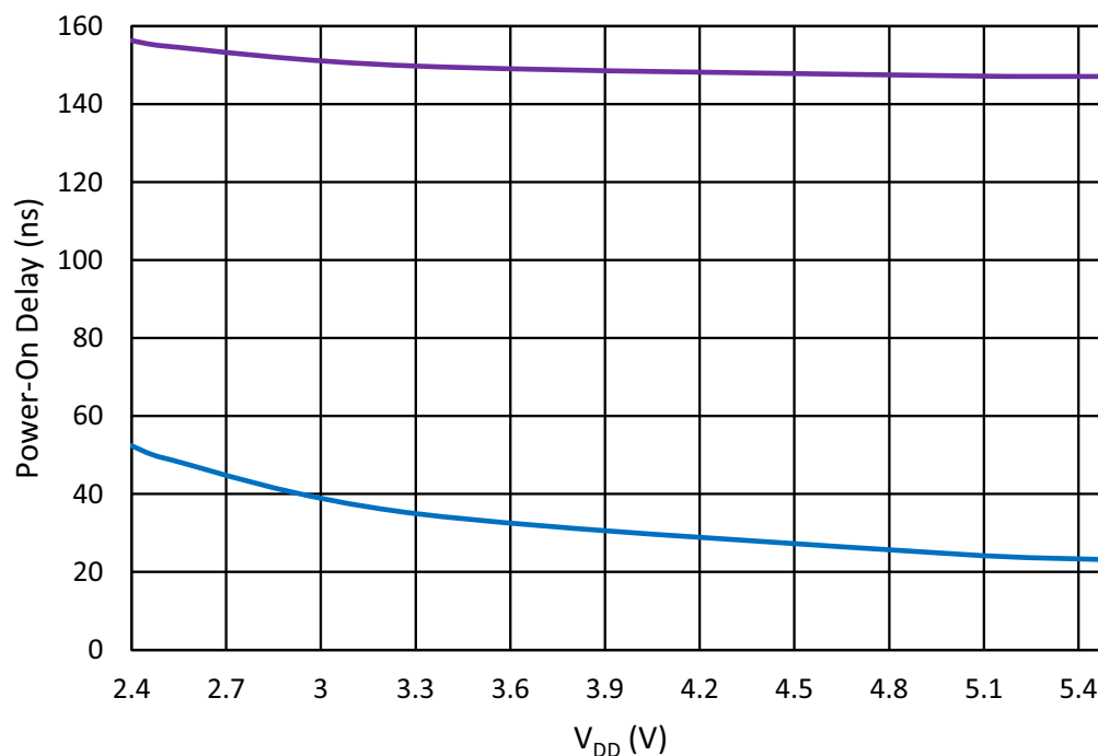
Figure 208: OSC2 Maximum Power-On Delay vs. V_{DD} at T = 25^{\circ}\text{C} , OSC2 = 25 MHz
