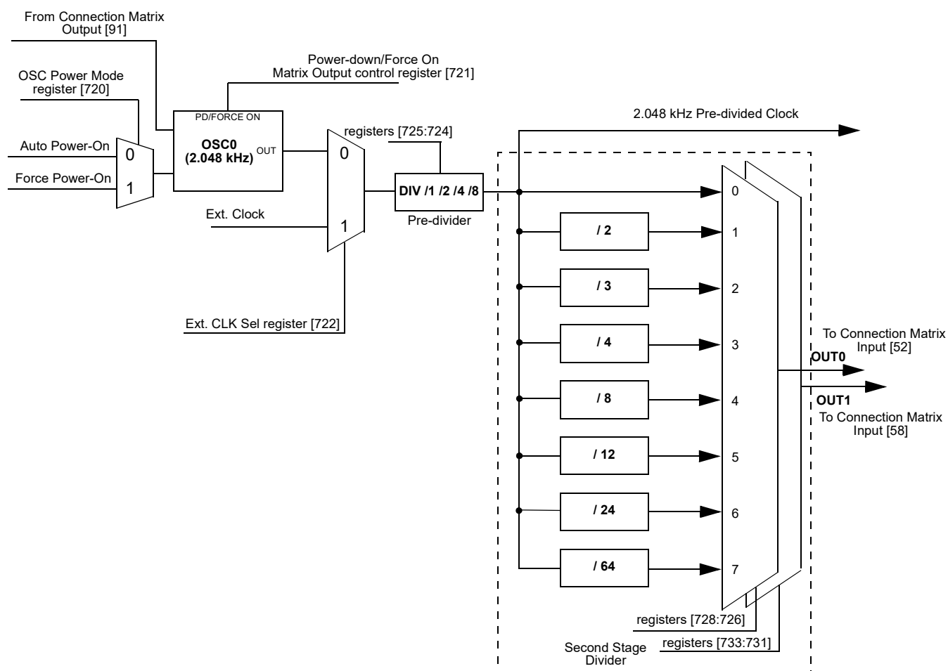
Figure 201: Oscillator0 Block Diagram
