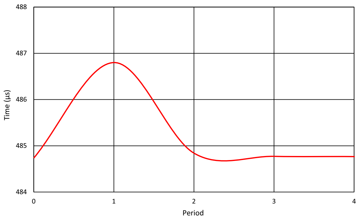
Figure 213: Oscillator0 Settling Time, V_{DD} = 3.3\text{ V} , T = 25\text{ }^{\circ}\text{C} , \text{OSC0} = 2\text{ kHz}
