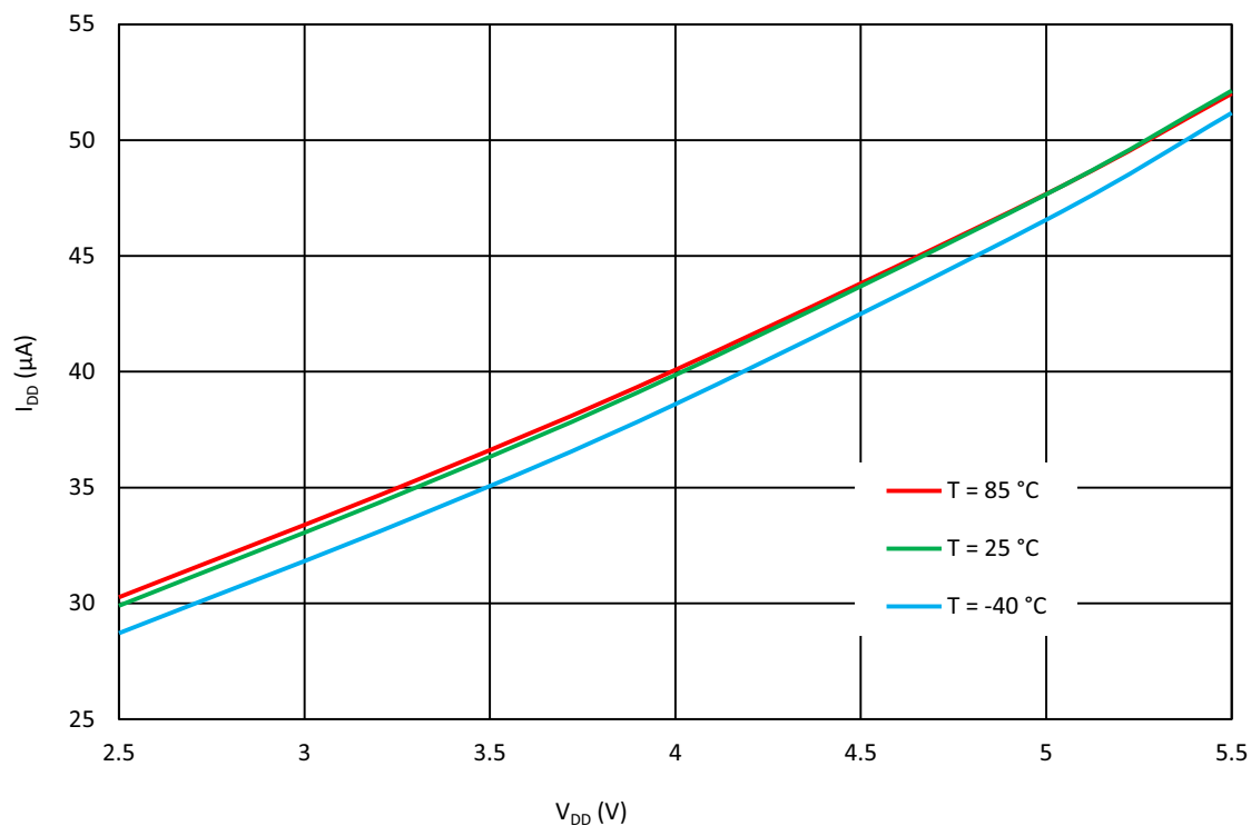
Figure 222: OSC2 Current Consumption vs. V_{DD} (Pre-Divider = 8)
