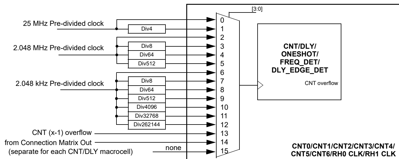
Figure 204: Clock Scheme
