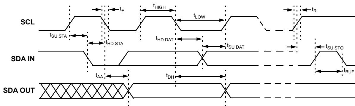
Figure 227: I 2 C General Timing Characteristics
