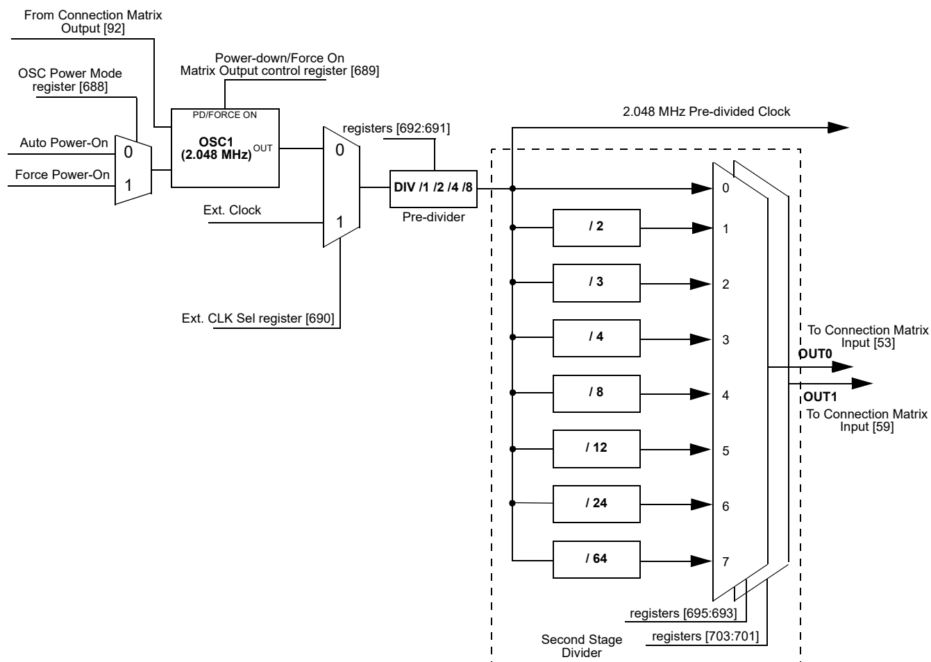
Figure 202: Oscillator1 Block Diagram
