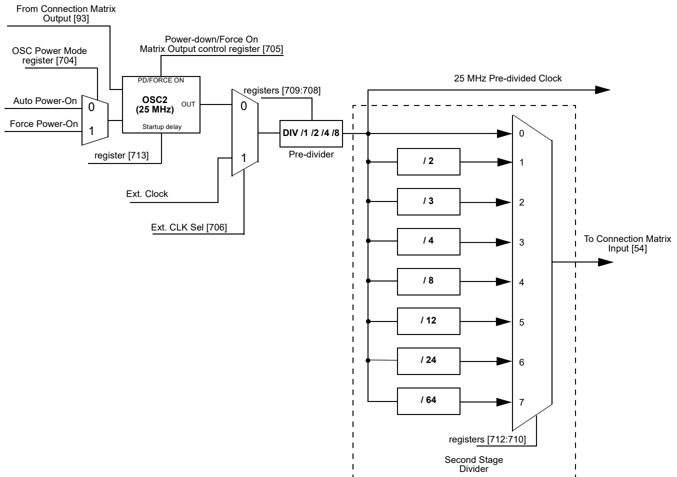
Figure 203: Oscillator2 Block Diagram
