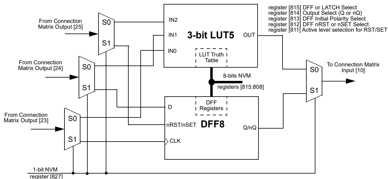
Figure 24: 3-bit LUT5 or DFF8
