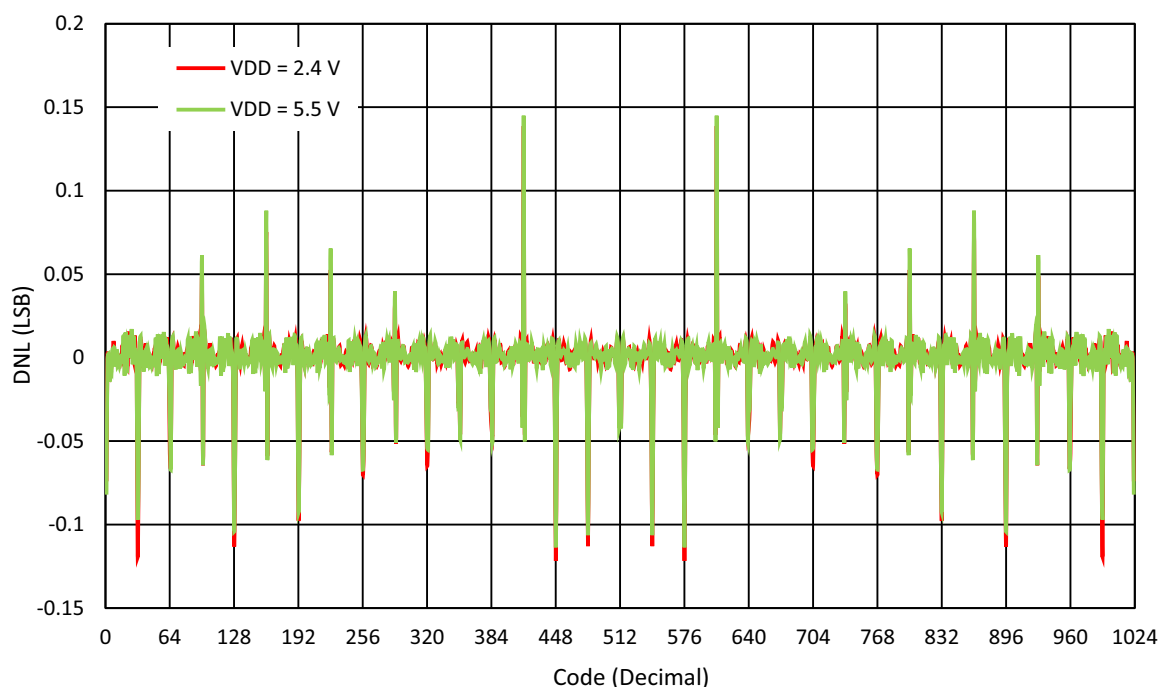
Figure 183: DNL vs. Digital Code, Potentiometer Mode ( V_{AB} = 1 V) at T = 25 °C
