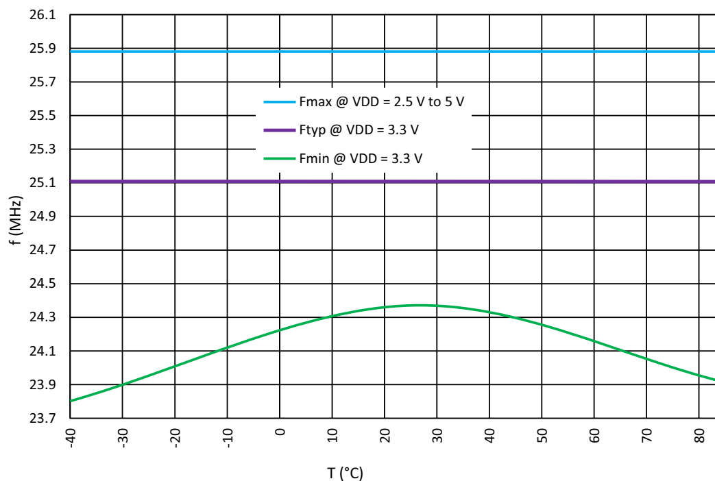
Figure 211: OSC2 Frequency vs. Temperature, OSC2 = 25 MHz
