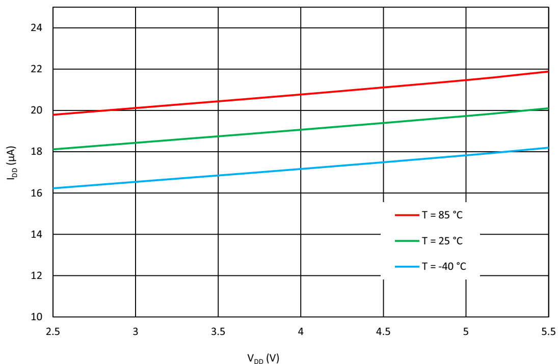
Figure 219: OSC1 Current Consumption vs. V DD (Pre-Divider = 8)
