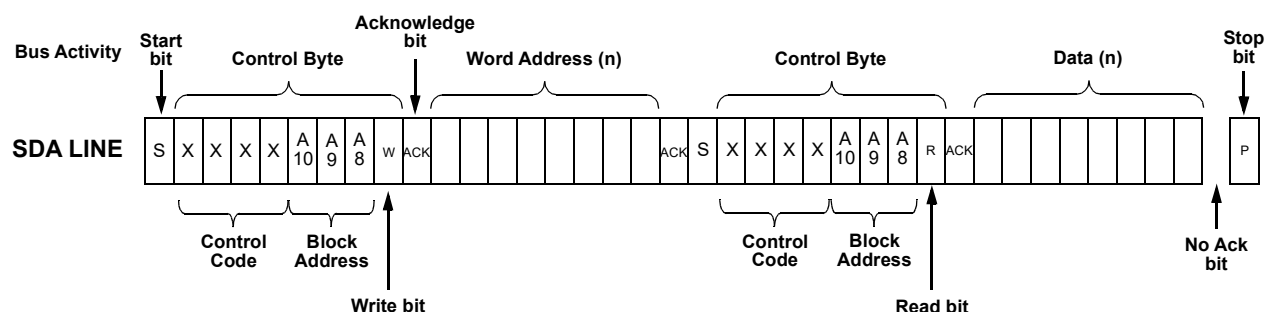
Figure 231: Random Read Command
