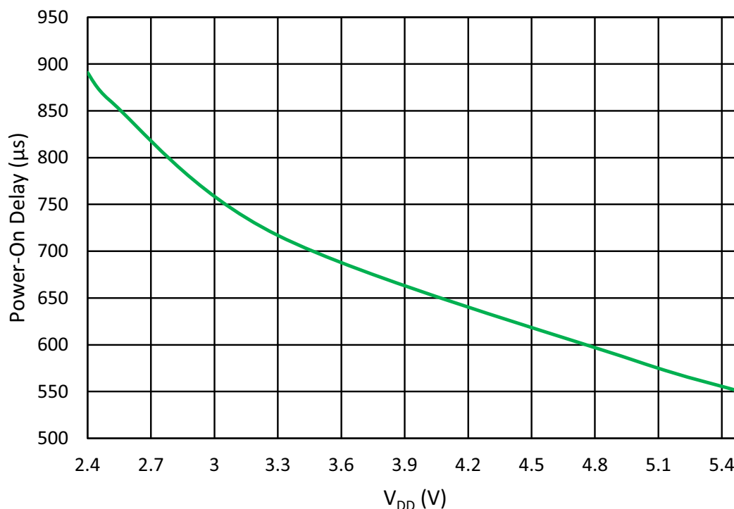
Figure 206: OSC0 Maximum Power-On Delay vs. V DD at T = 25 °C, OSC0 = 2.048 kHz
