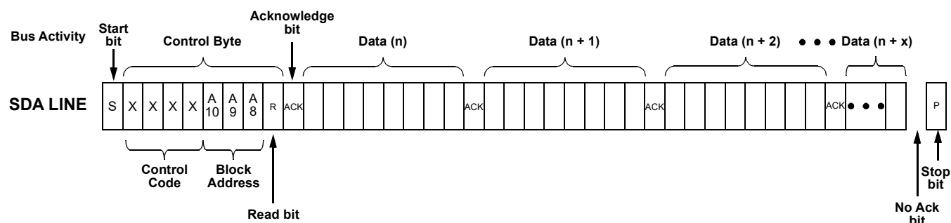
Figure 232: Sequential Read Command
