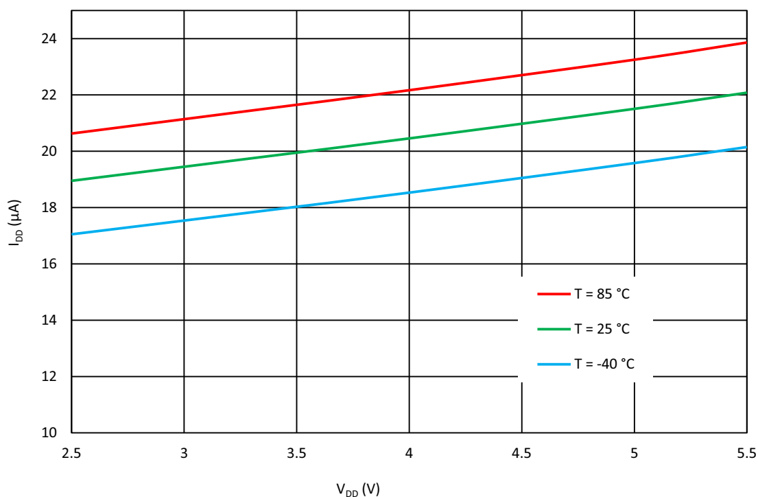
Figure 217: OSC1 Current Consumption vs. V DD (Pre-Divider = 1)
