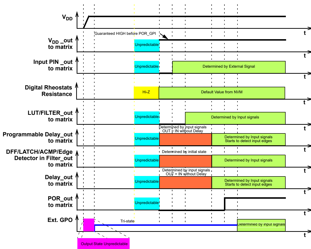
Figure 224: Internal Macrocell States During POR Sequence
