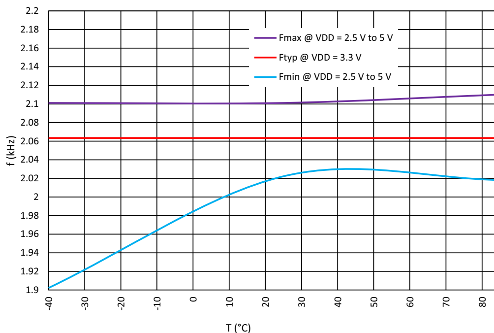
Figure 209: OSC0 Frequency vs. Temperature, OSC0 = 2.048 kHz
