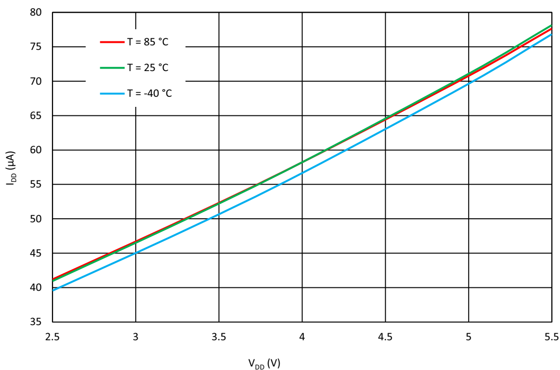
Figure 220: OSC2 Current Consumption vs. V DD (Pre-Divider = 1)
