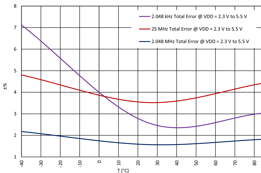
Figure 212: Oscillators Total Error vs. Temperature
