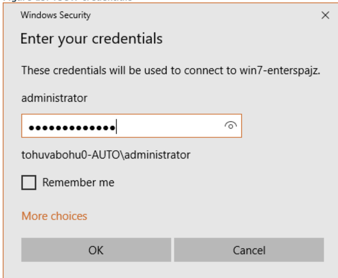
Figure 15: TSGW credentials
