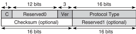
Figure 8 GRE Header
