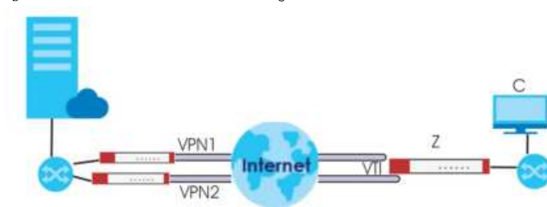
Figure 210 VTI and Trunk for VPN Load Balancing
