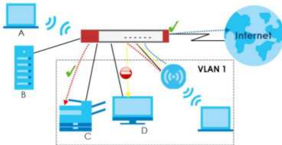
Figure 286 Layer-2 Isolation Application
