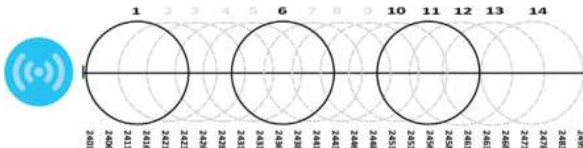
Figure 177 An Example Three-Channel Deployment
