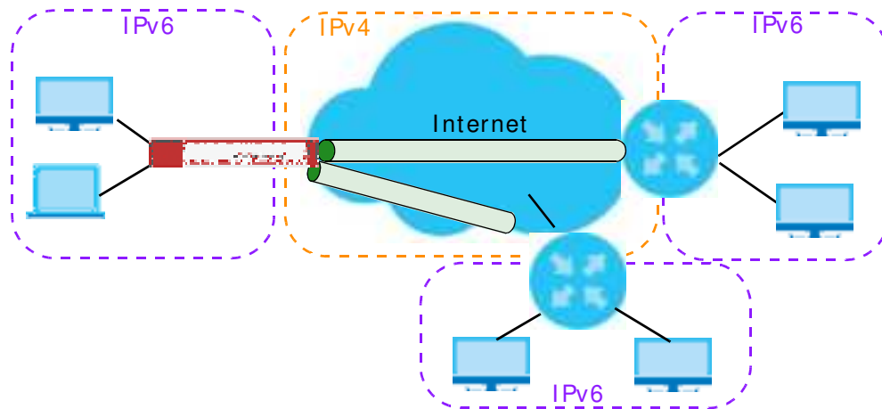
Figure 201 6to4 Tunnel
