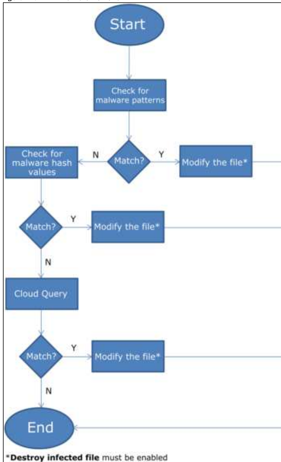
Figure 410 Anti-Malware Flowchart
