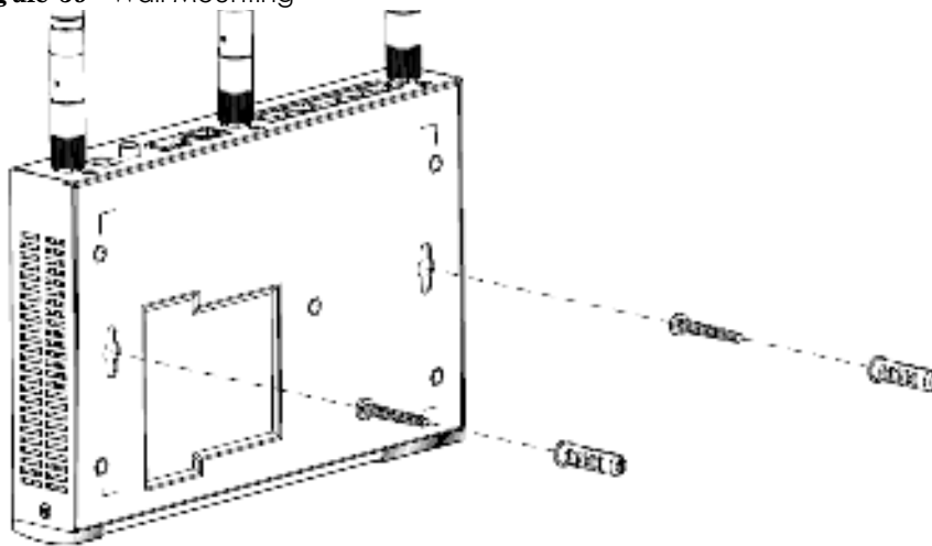
Figure 59 Wall Mounting
