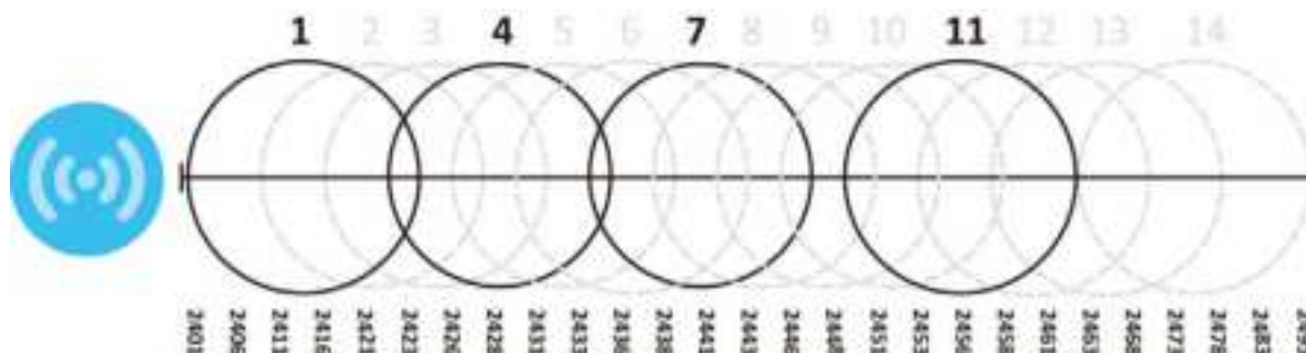
Figure 178 An Example Four-Channel Deployment
