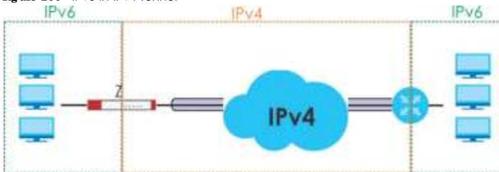
Figure 200 IPv6-in-IPv4 Tunnel
