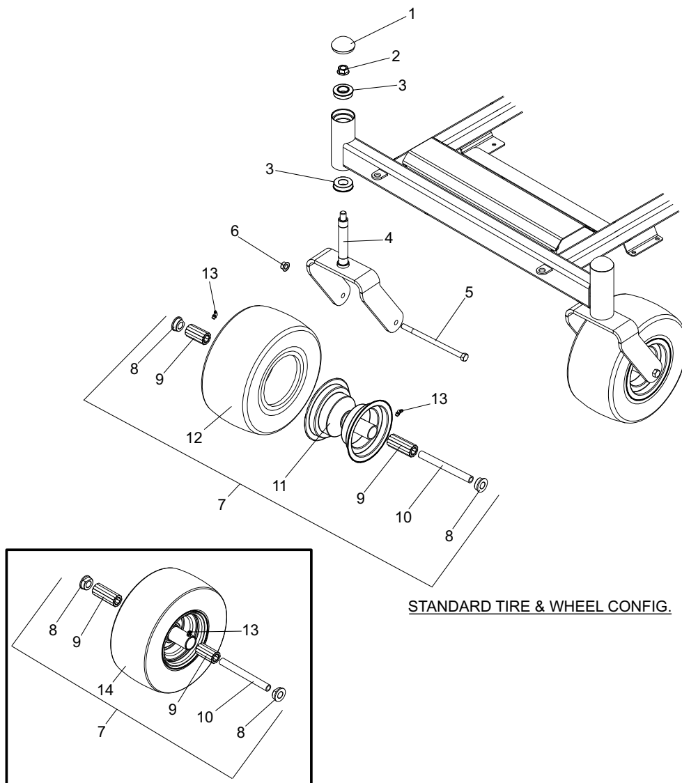
RUN FLAT TIRE & WHEEL CONFIG. (OPTIONAL)
