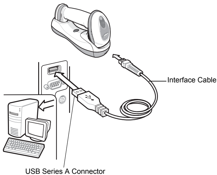
Figure 7-1 USB Connection
