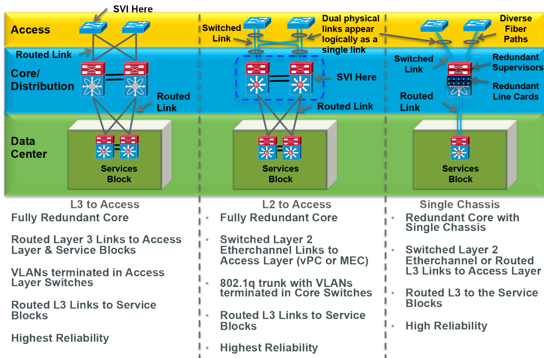
Figure 2. Connected Stadium Core Options
