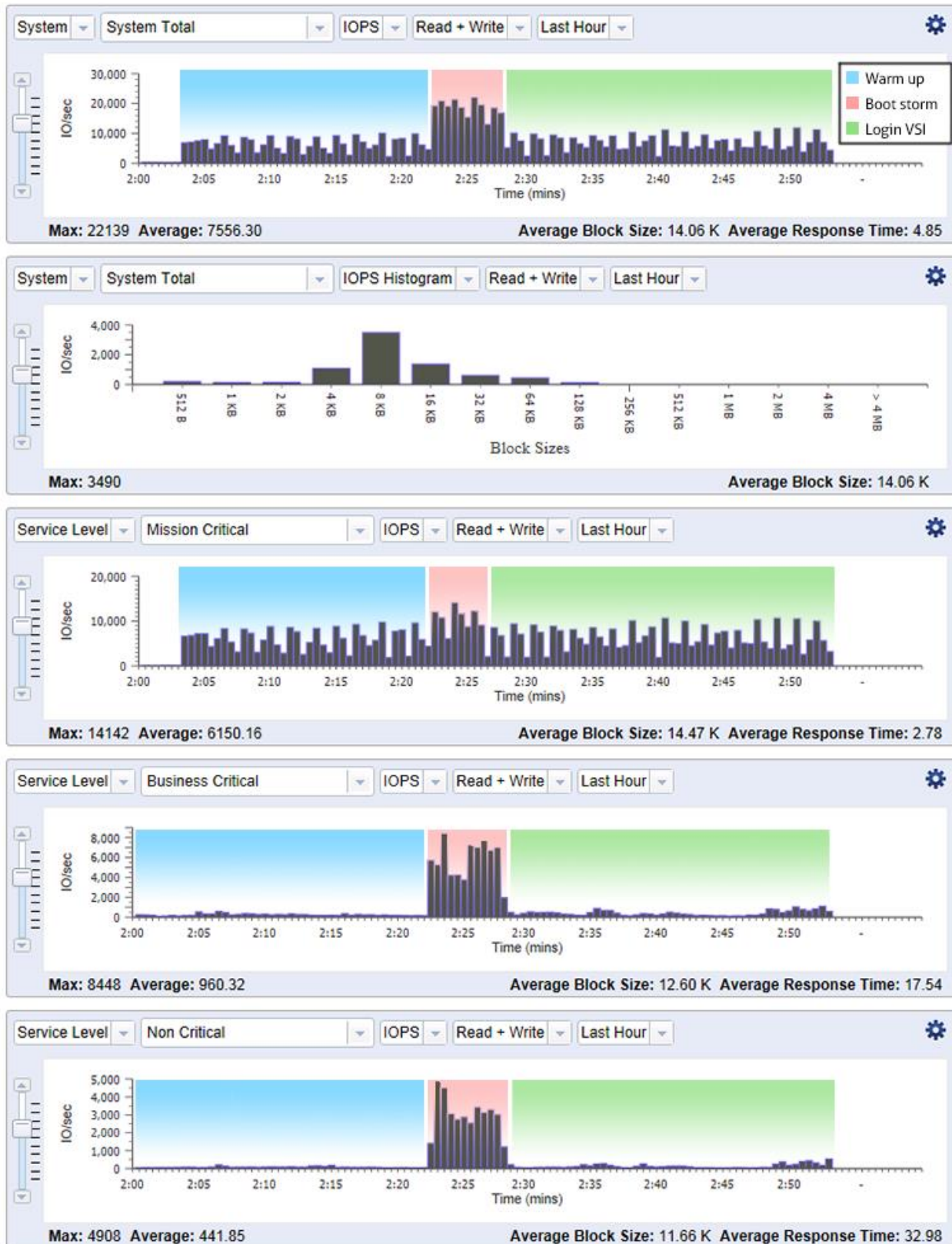
Figure 46: ioControl interface showing IOPS generated during testing.
