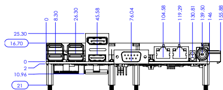
Figure 1.6 MIO-5393 Mechanical Drawing (with Heat Spreader)
