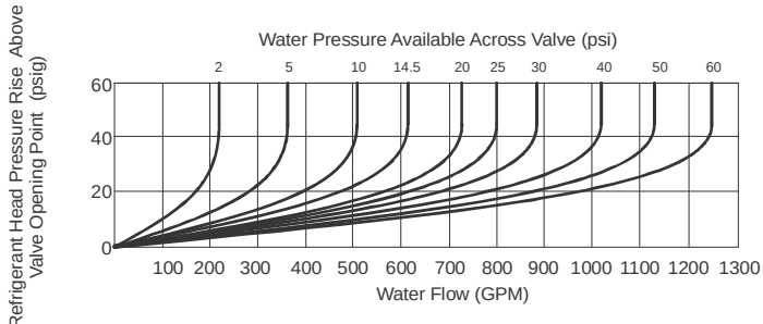
CAPACITY CHART FOR 4 in. VALVE
