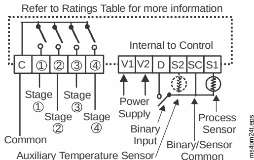
MS4PM24T Panel Mount Control Wiring
