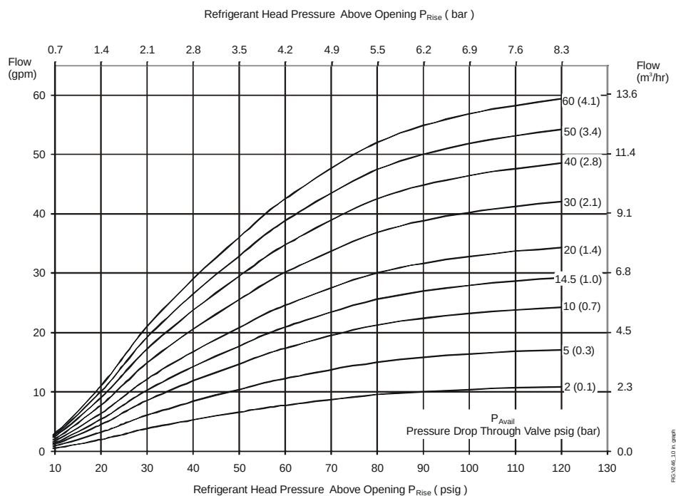
1 in. Direct Acting Valve Flowchart
