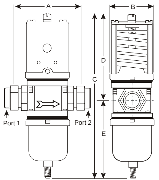
High Refrigerant Pressure 1 in. V146GL1 Valves
