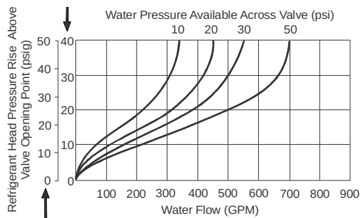
CAPACITY CHART FOR 4 in. VALVE
