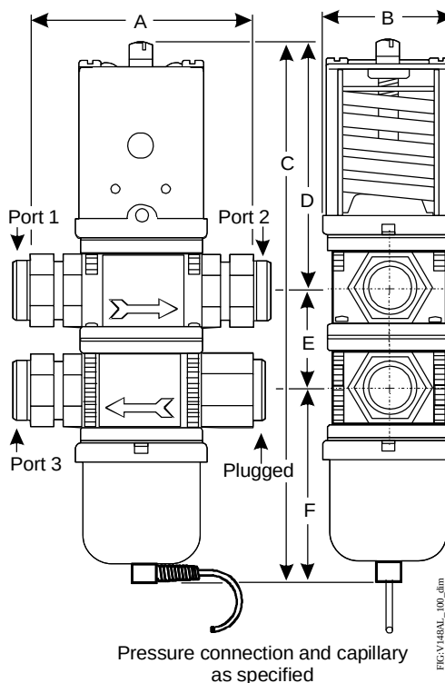
1 in. V148AL Valve
