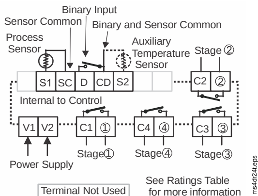
MS4DR24T Din Rail Mount Control Wiring
