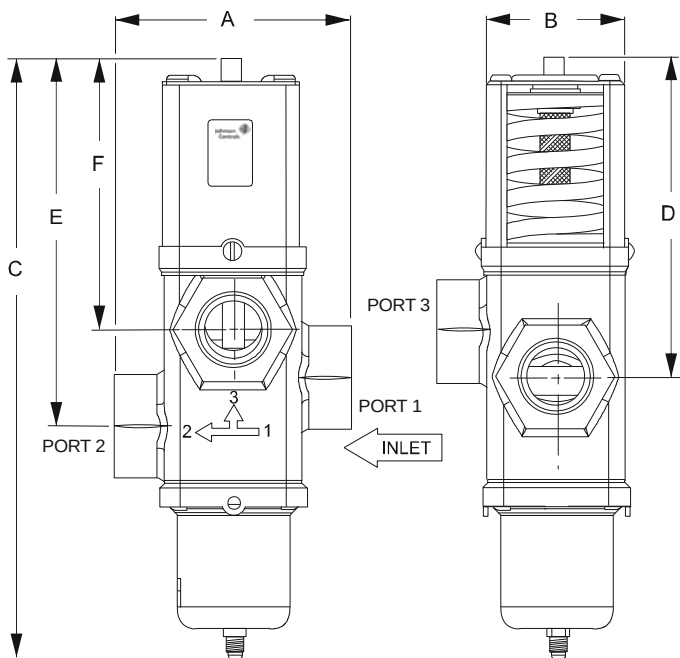
V248 1-1/2 in. Screw Connection Valves Dimensions
