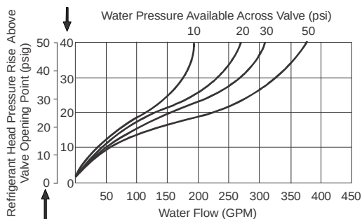
CAPACITY CHART FOR 2-1/2 in. VALVE
