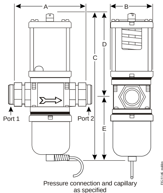
3/4 in. V146EK Valves
