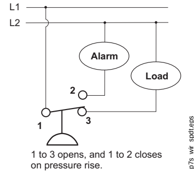
Typical Wiring for SPDT Switch (P70E, F Models)
