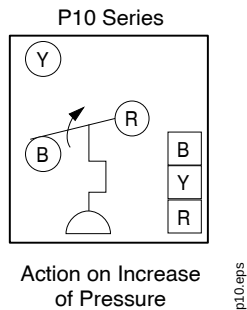
P10 Series Action Diagram
