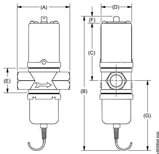
V46 Series Threaded Type Valves
