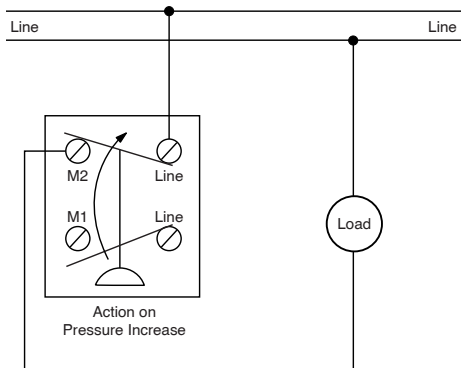
P67 Wiring Diagram (no alarm)
