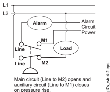
Typical Wiring for Four-Wire Two-Circuit Switch used for a High Pressure Cutout Application with an Alarm Circuit (P70J, K, and P170K Models)
