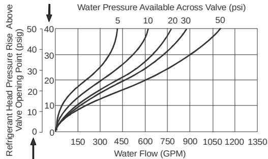
CAPACITY CHART FOR 4 in. VALVE
