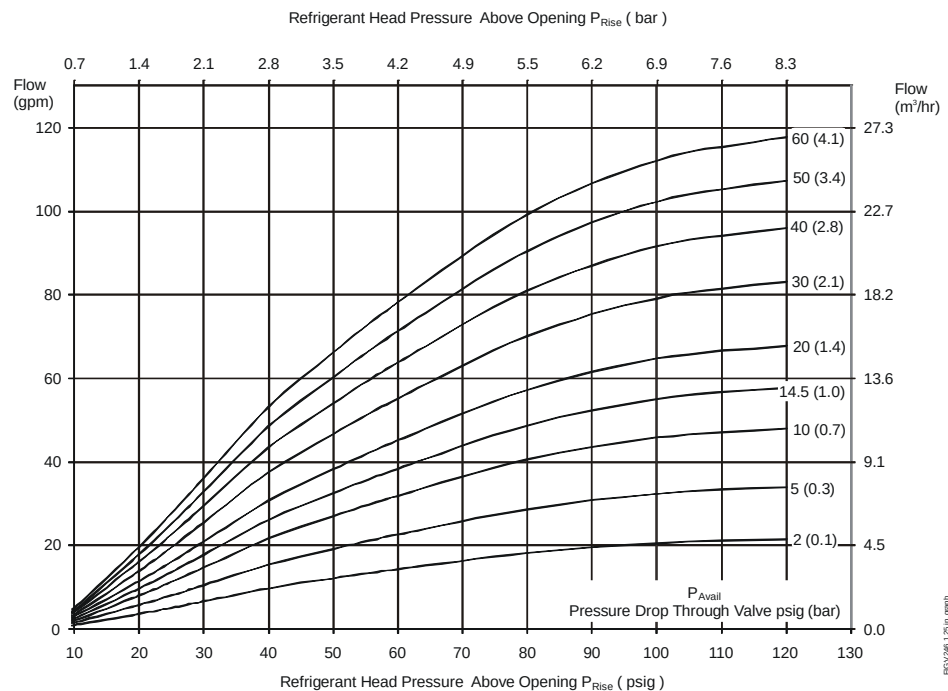
1-1/4 in. Direct Acting Valve Flowchart
