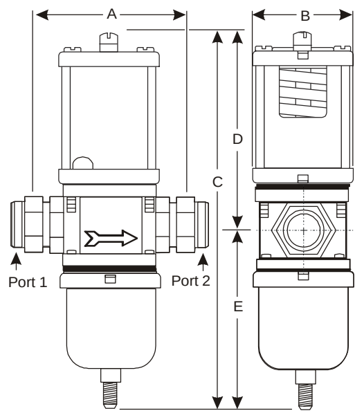
High Refrigerant Pressure 3/4 in. V146GK1 Valves
