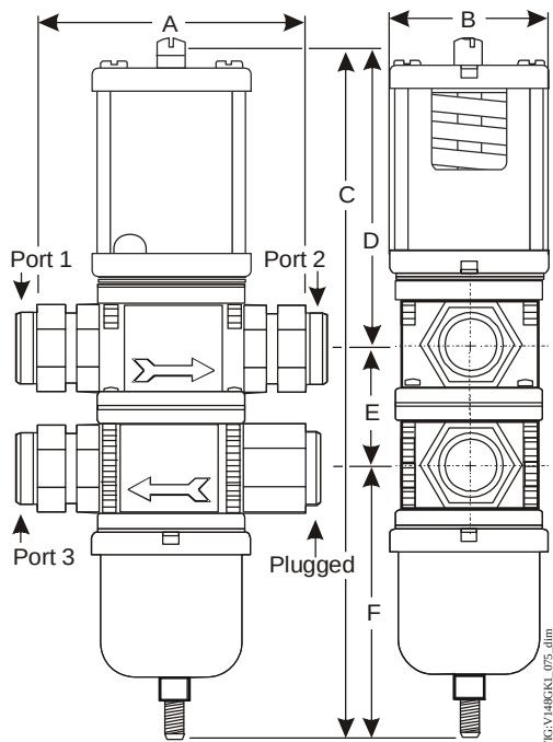
3/4 in. High Refrigerant Pressure V148GK1 Valves
