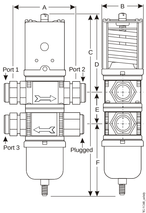
V248 Union Sweat Connection Valves Dimensions
