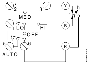
T23A Thermostat
