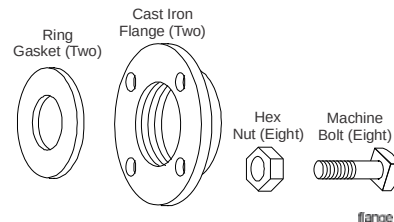
Companion Flange Kit
