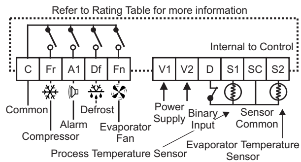
MR4 Panel Mount Control
