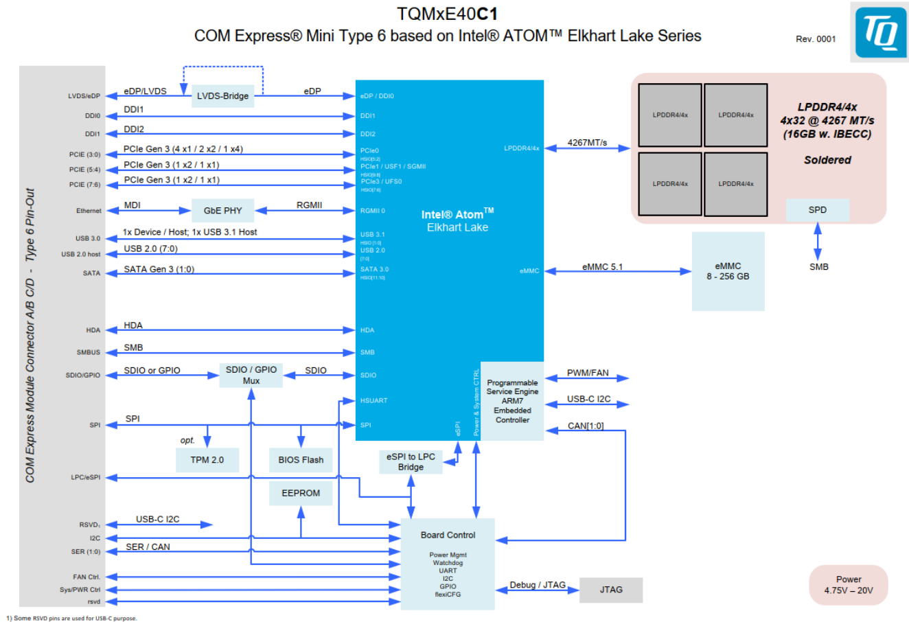
Illustration 1: TQMxE40C1 Block Diagram
