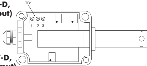
Figure 5: Terminal Connections
