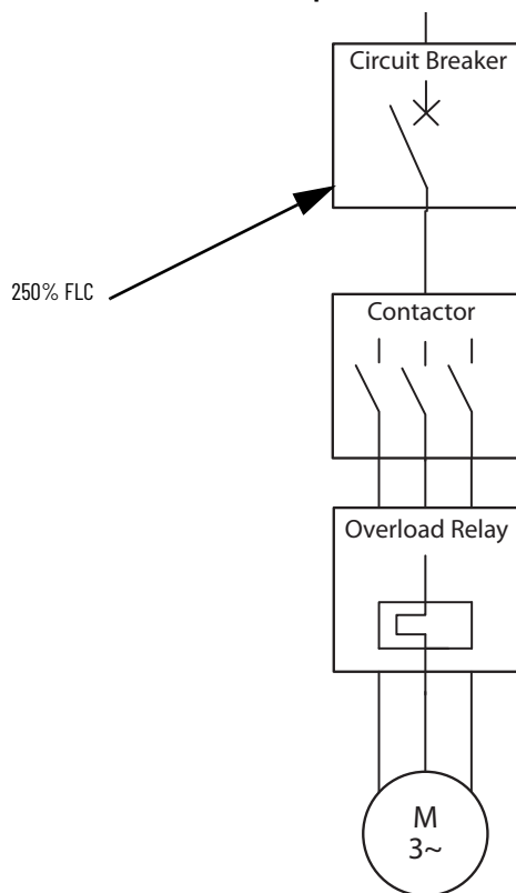
Figure 16 - Standard short-circuit protection
