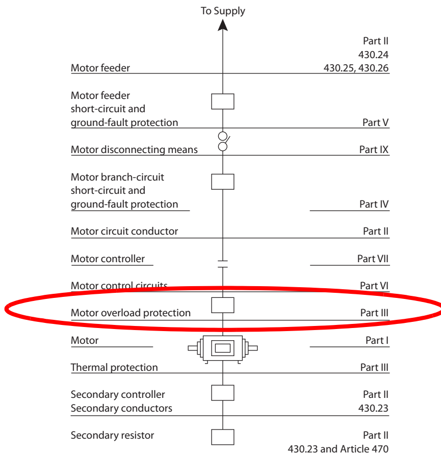
Figure 13 - NEC Article 430 Contents
