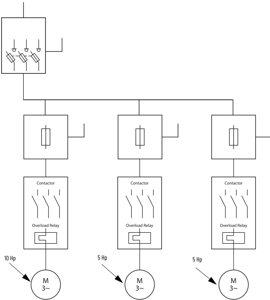
Figure 22 - Sizing the motor feeder protective device (Min)
