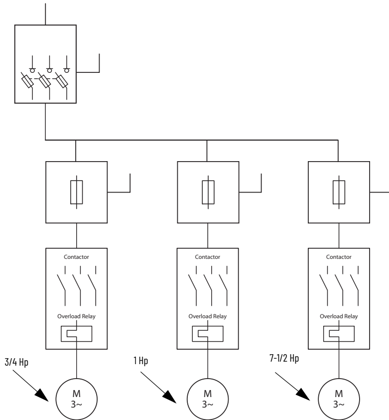
Figure 21 - Sizing the motor feeder protective device (max.)
