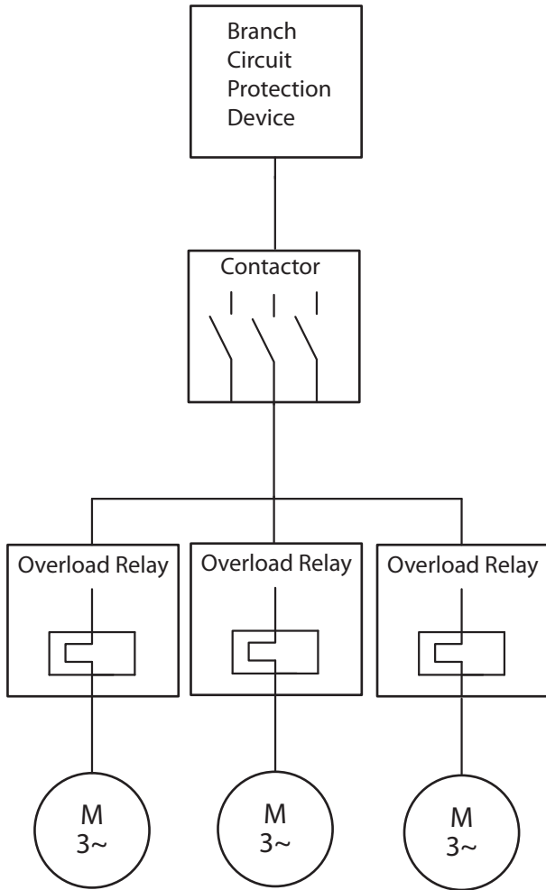
Figure 26 - Single controller with multiple motors
