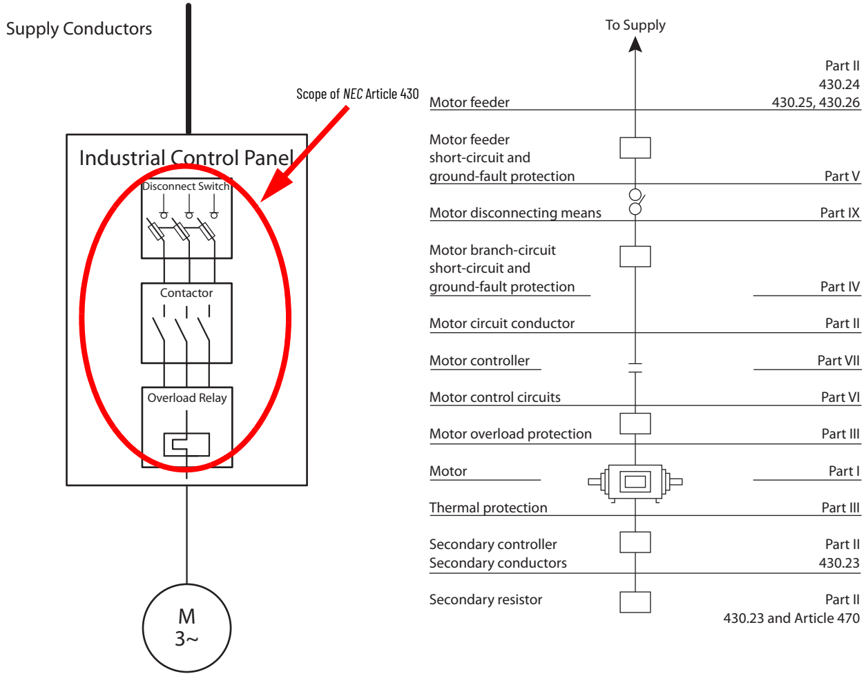
Figure 3 - NEC Article 430 Contents
