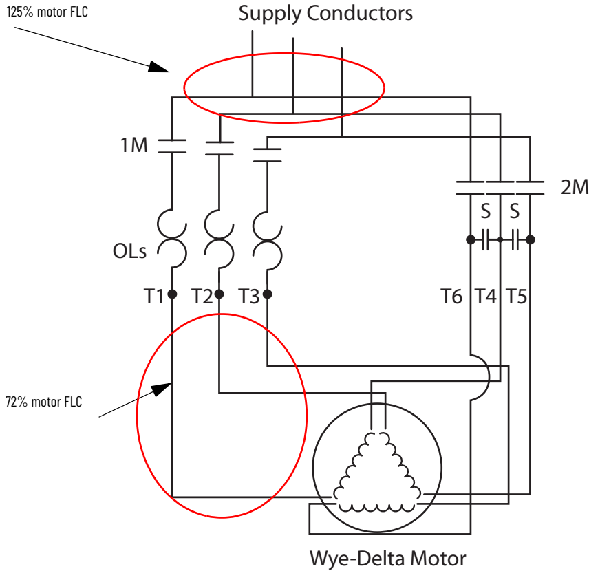
Figure 10 - Conductor sizing for Wye-Delta motors
