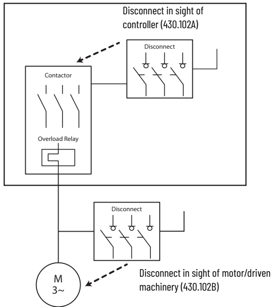
Figure 31 - Motor Disconnecting Means
