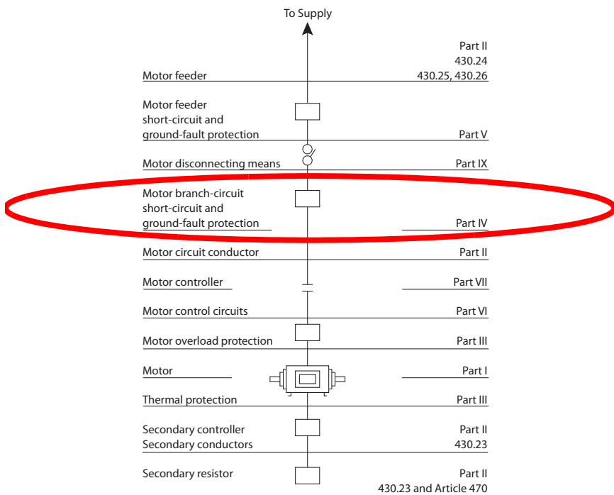
Figure 15 - NEC Article 430 Contents
