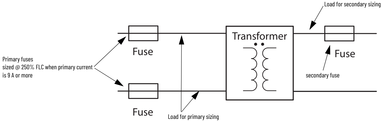
Figure 28 - Transformer with primary and secondary fusing
