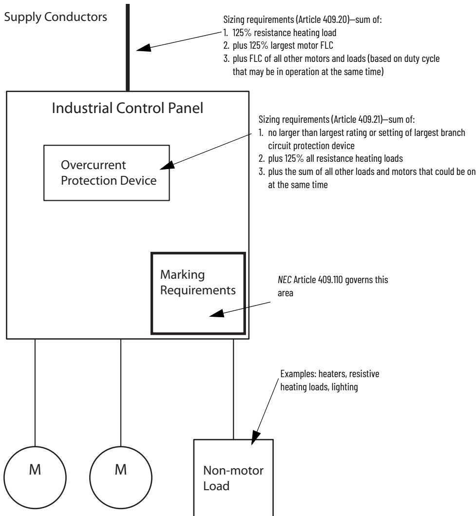
Figure 2 - Conductor and Marking Requirements for Industrial Control Panel Supply
