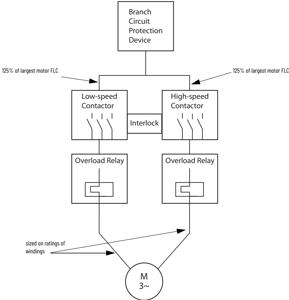
Figure 11 - Conductor sizing for multi-speed motors
