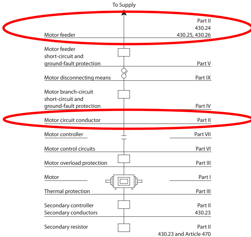
Figure 8 - NEC Article 430 Contents
