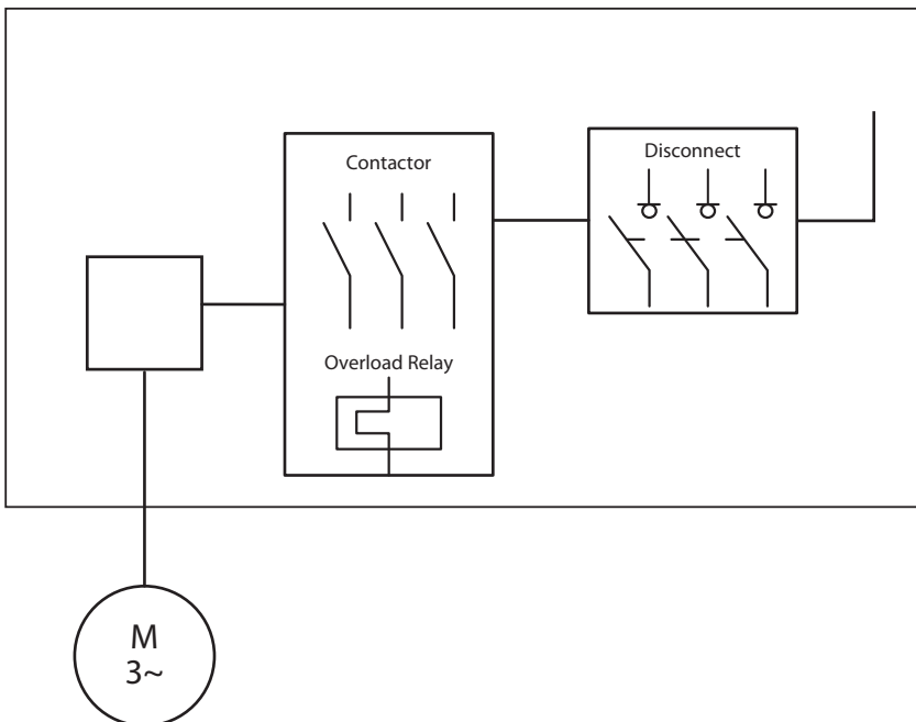
Figure 32 - Motor within Sight of Disconnect
