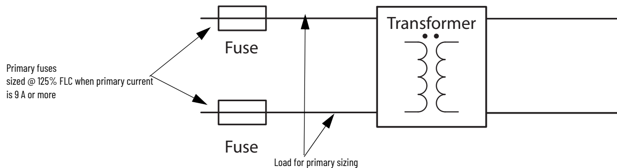
Figure 29 - Transformer with only primary fusing
