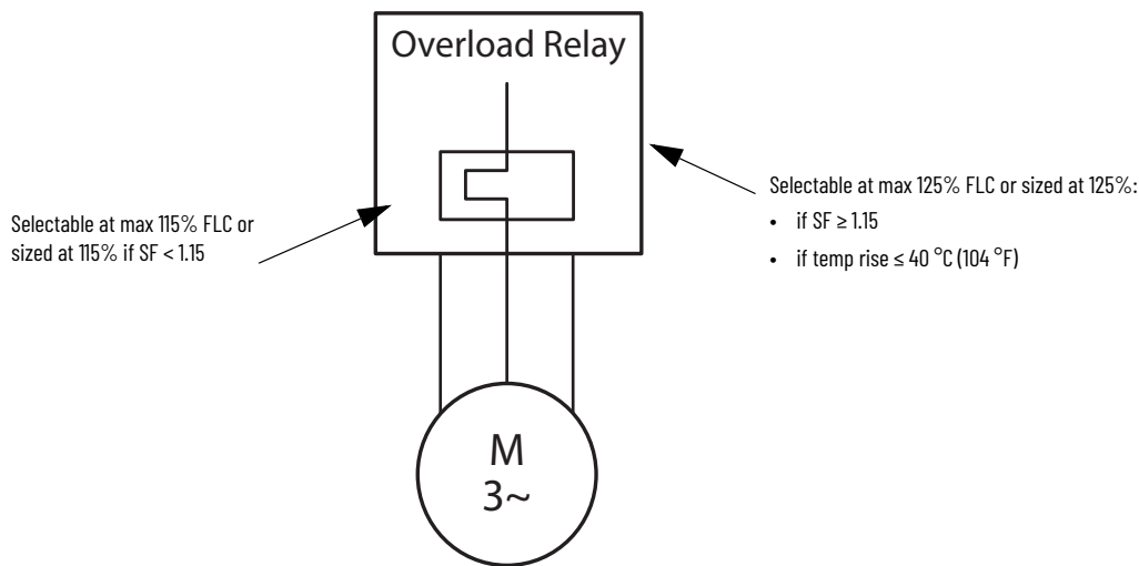
Figure 14 - Basic overload sizing (Max ratings)
