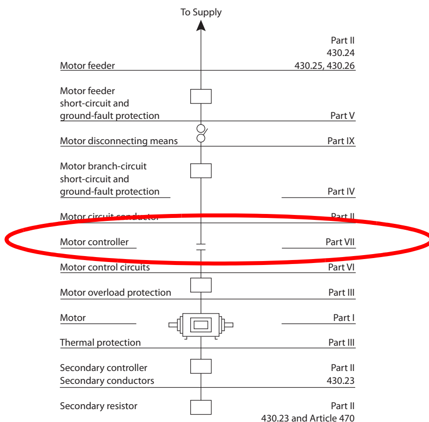
Figure 23 - NEC Article 430 Contents
