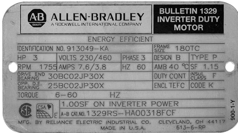
Figure 5 - Typical Motor Nameplate
