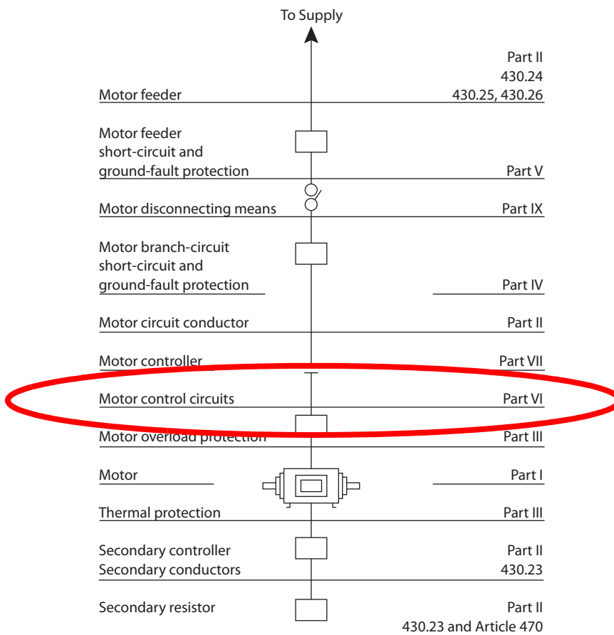
Figure 27 - NEC Article 430 Contents
