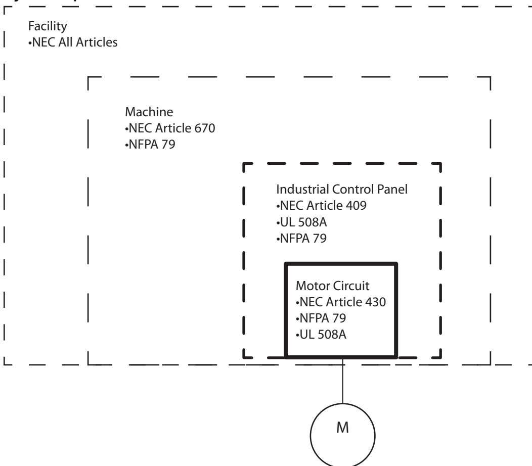
Figure 1 - Scope of American Standards
