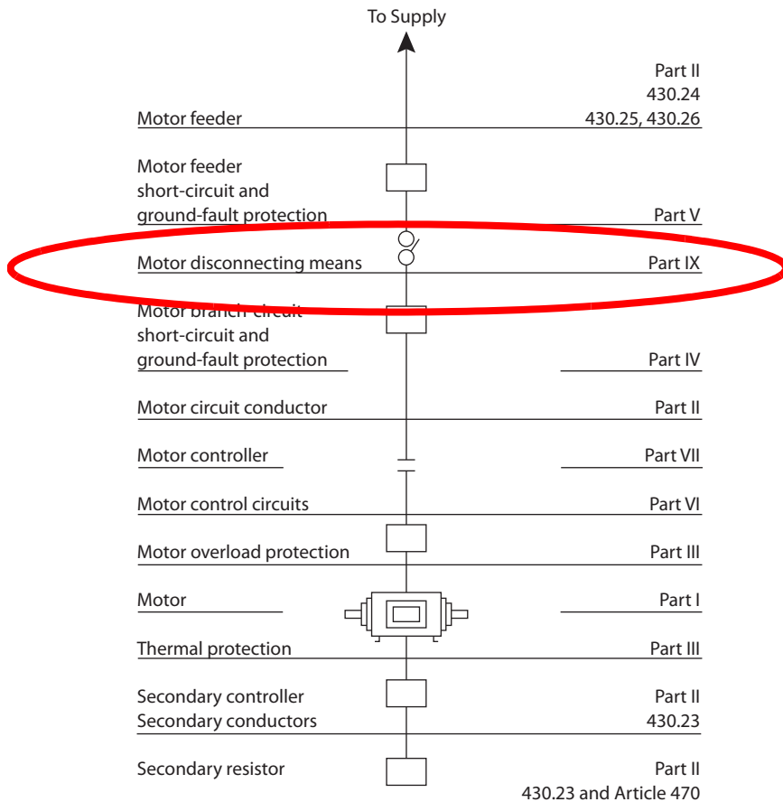
Figure 30 - NEC Article 430 Contents
