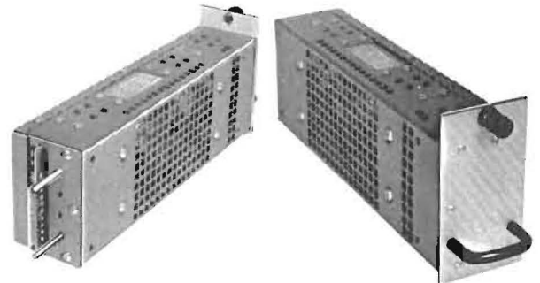
Rear view showing printed circuit board connector and keying pins
