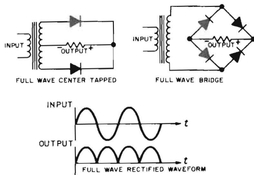
Figure 6: Full wave rectification.
