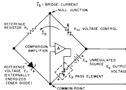
Figure 1: Kepco comparison bridge connected as a voltage regulator.
