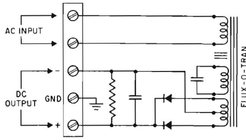
120 SERIES SCHEMATIC
