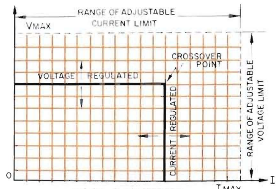
TYPICAL CHARACTERISTIC AUTOMATIC VOLTAGE/CURRENT CROSSOVER
