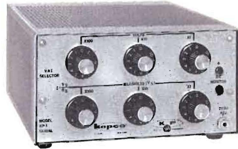
MODEL KP-1 for use with Kepco ABC, CK and PAX Groups of Regulated Power Supplies. (1 milliampere Kepco Bridge Circuit).
