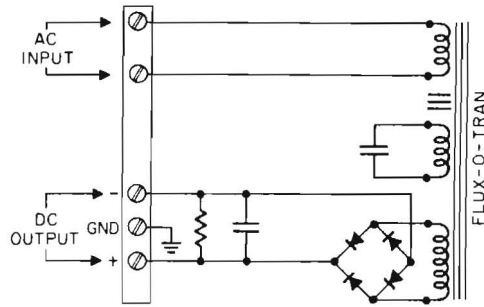
180 SERIES SCHEMATIC
