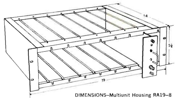
DIMENSIONS—Multiunit Housing RA19-8 Shipped disassembled Assembly instructions included
