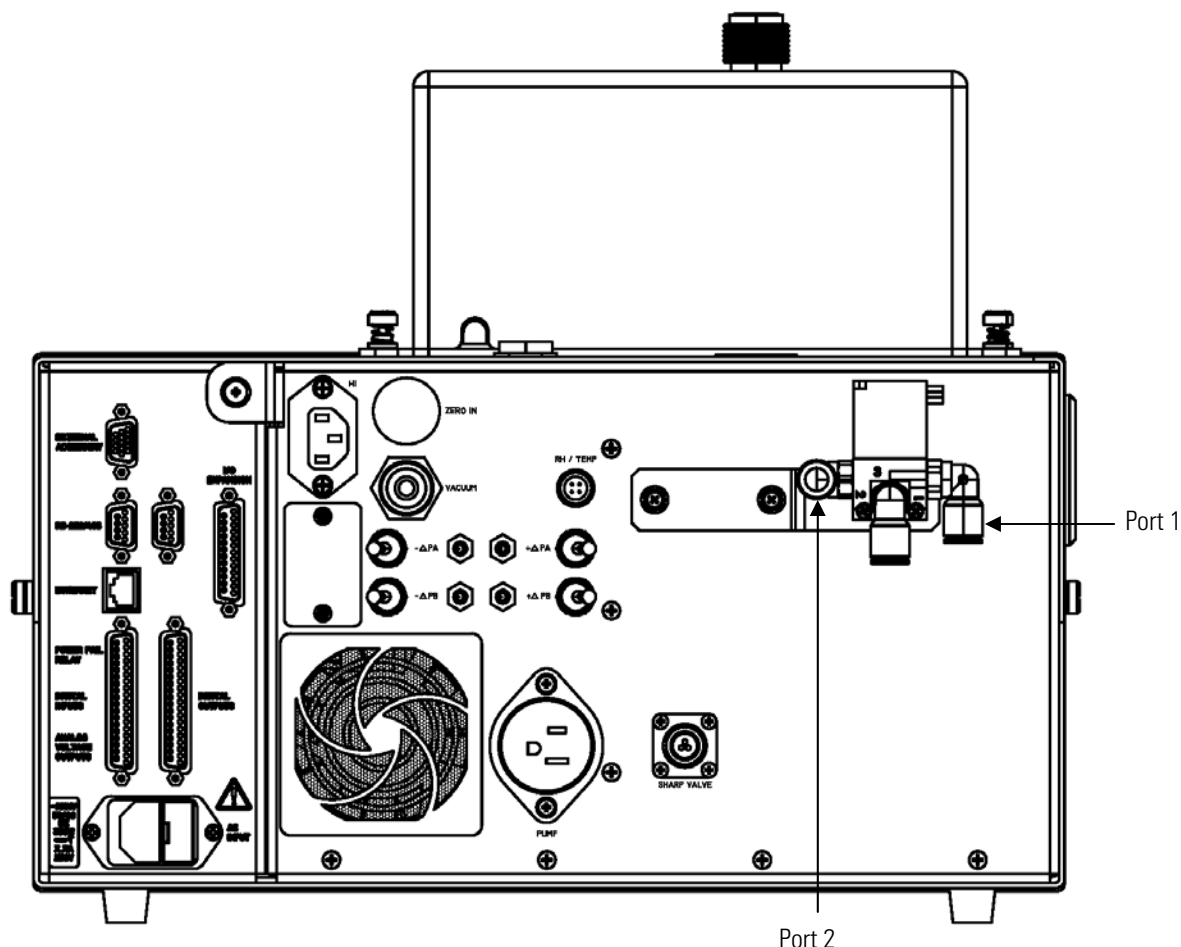
Figure 10–7. Rear Valve Assembly Installation
