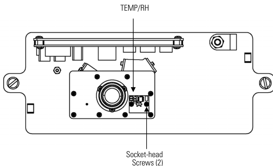
Figure 7–26. Disconnecting the RH/Temp Connector
