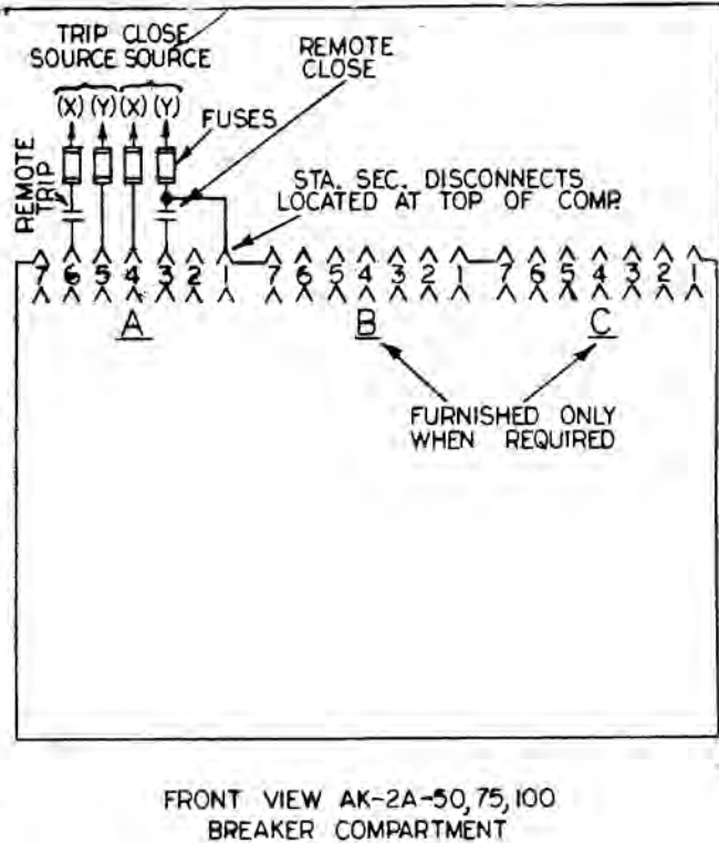
TYPICAL WIRING DIAGRAMS
