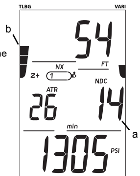
Fig. 48 - NO DECO MAIN (DTR is NDC)
