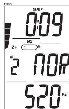
Fig. 3 - NORM SURF MAIN (> 10 min after dive 1)
