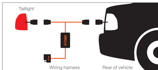
Custom wiring harnesses use multiple plugs to 'T' into the taillight assembly
