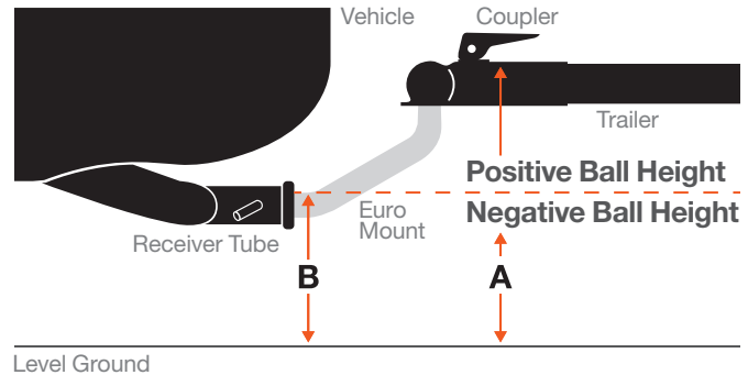
45571 Euro Mount® vs 45521 old-style
