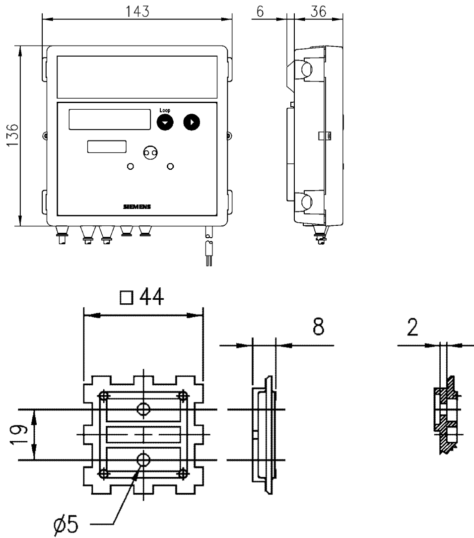
Adapter plate
