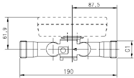
Mounting length 190 mm (threaded)
