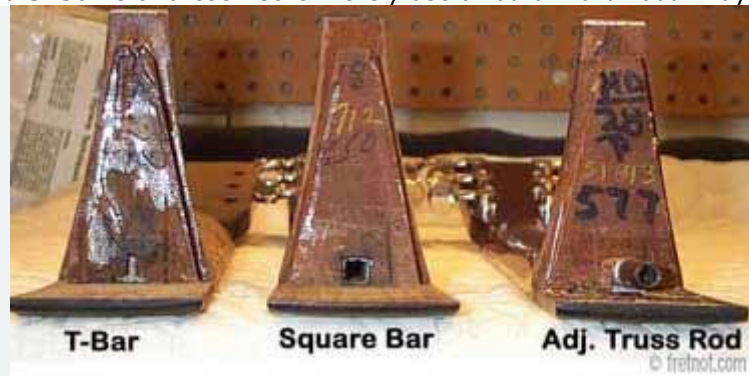
Comparison of Truss Rod Types
