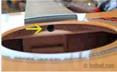
A heel end truss rod nut accessible thru a hole in the top brace.
