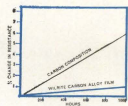
AGING STABILITY
